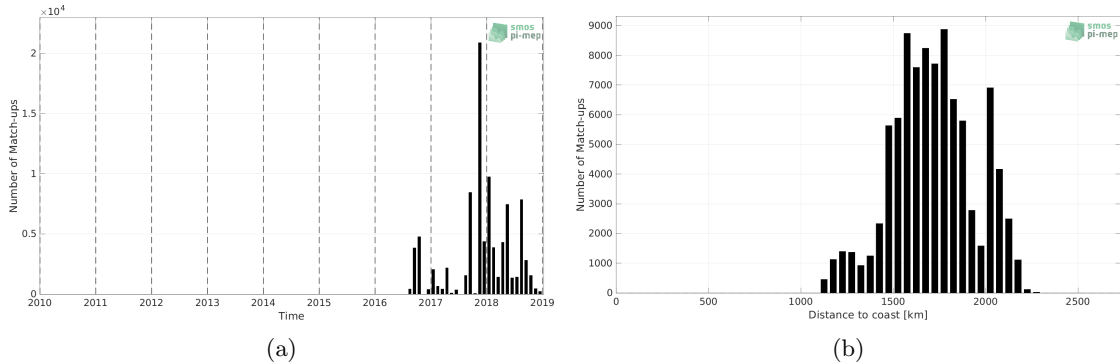
Figure 1: Number of match-ups between Surface drifters and SMOS and SMAP SSS L4 OI v1 - 7 Days (LOPS) SSS as a function of time (a) and as function of the distance to coast (b) over the SPURS 2 Pi-MEP region and for the full satellite product period.
