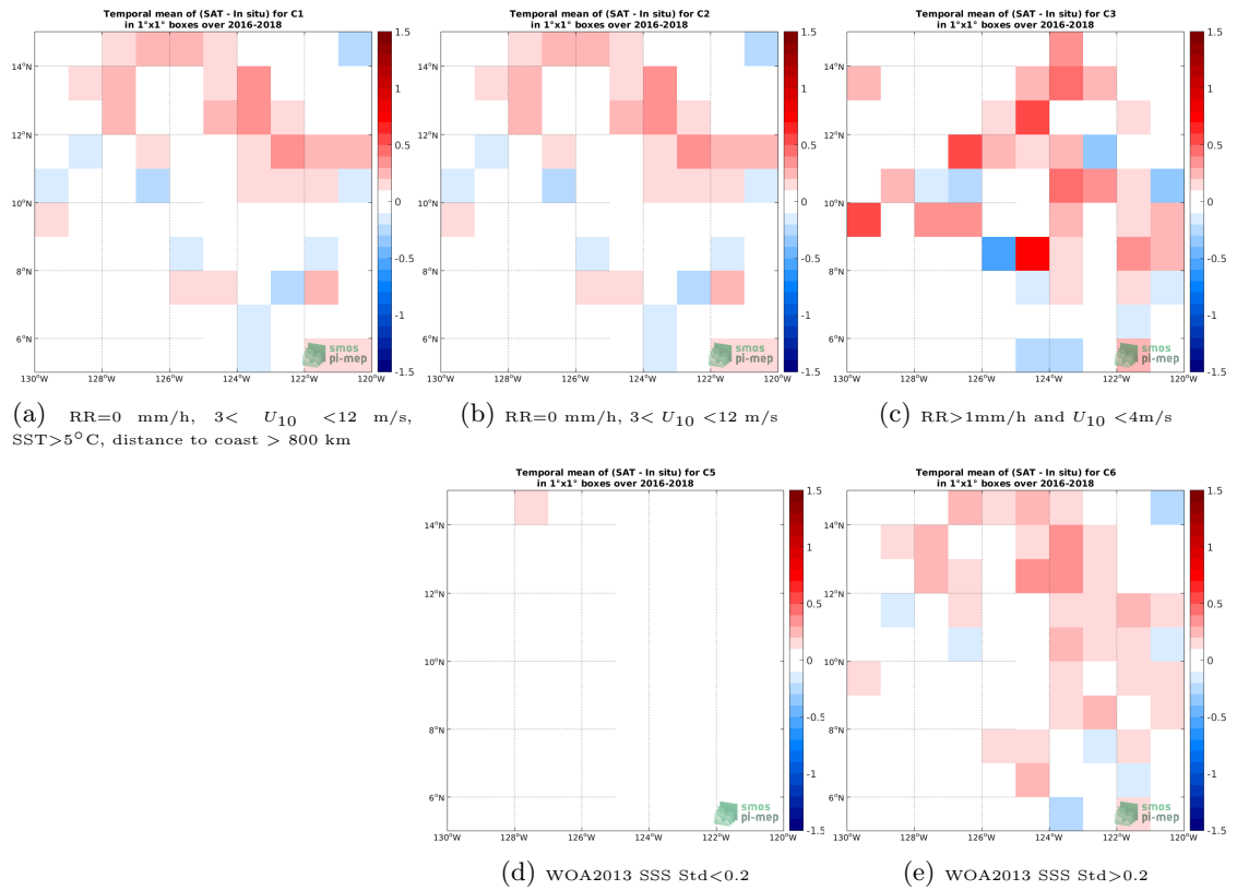
Figure 11: Temporal mean gridded over spatial boxes of size 1^\circ \times 1^\circ of \Delta SSS (SMOS and SMAP SSS L4 OI v1 - 7 Days (LOPS) - Surface drifters) for 5 different subdatasets corresponding to: RR=0 mm/h, 3 < U_{10} < 12 m/s, SST >5^\circ\text{C} , distance to coast > 800 km (a), RR=0 mm/h, 3 < U_{10} < 12 m/s (b), RR >1 mm/h and U_{10} < 4 m/s (c), WOA2013 SSS Std <0.2 (d), WOA2013 SSS Std >0.2 (e).
