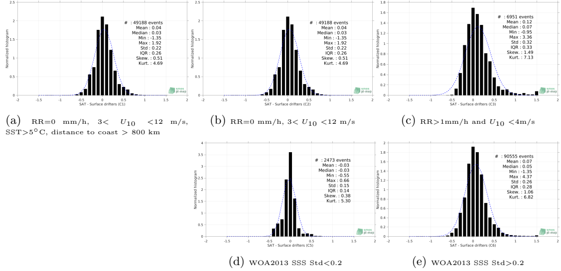
Figure 12: Normalized histogram of \Delta SSS (SMOS and SMAP SSS L4 OI v1 - 7 Days (LOPS) - Surface drifters) for 5 different subdatasets corresponding to: RR=0 mm/h, 3 < U_{10} < 12 m/s, SST>5°C, distance to coast > 800 km (a), RR=0 mm/h, 3 < U_{10} < 12 m/s (b), RR>1mm/h and U_{10} < 4 m/s (c), WOA2013 SSS Std<0.2 (d), WOA2013 SSS Std>0.2 (e).
