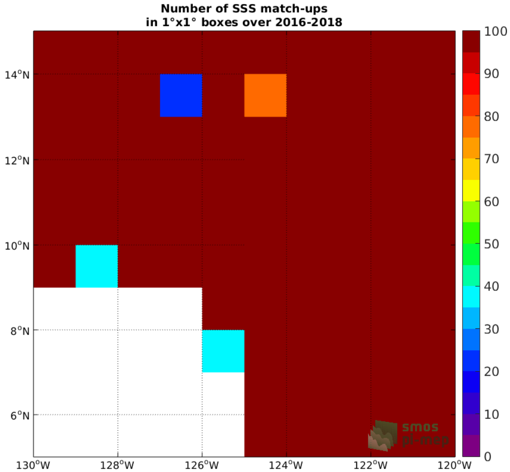
Figure 3: Number of SSS match-ups between Surface drifters SSS and the SMOS and SMAP SSS L4 OI v1 - 7 Days (LOPS) SSS product for the SPURS 2 Pi-MEP region over 1°x1° boxes and for the full satellite product period.
