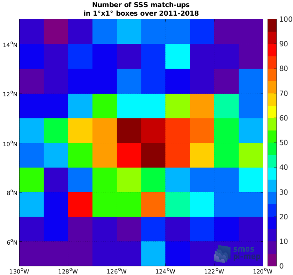
Figure 4: Number of SSS match-ups between Argo SSS and the SMOS and SMAP SSS L4 OI v1 - 7 Days (LOPS) SSS product for the SPURS 2 Pi-MEP region over 1^\circ \times 1^\circ boxes and for the full satellite product period.
