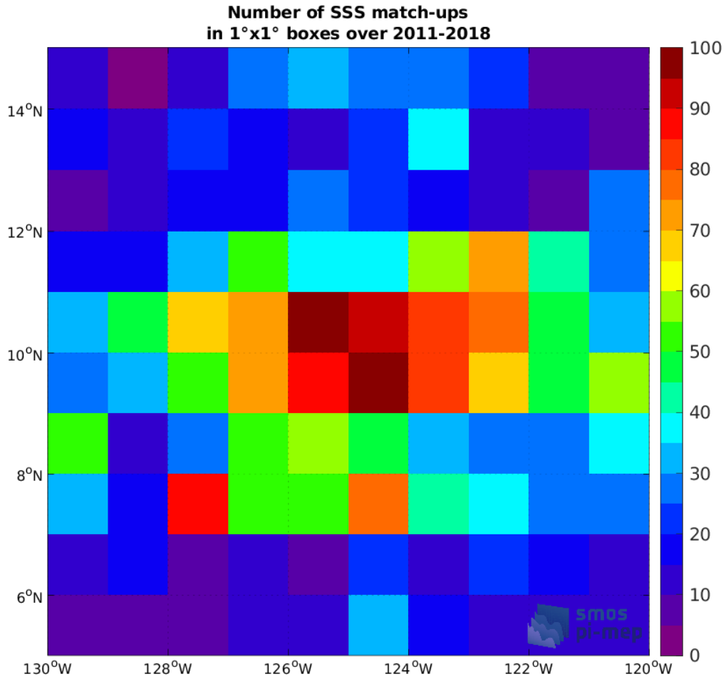
Figure 4: Number of SSS match-ups between Argo SSS and the SMOS and SMAP SSS L4 OI v1 - 7 Days (LOPS) SSS product for the SPURS 2 Pi-MEP region over 1°×1° boxes and for the full satellite product period.
