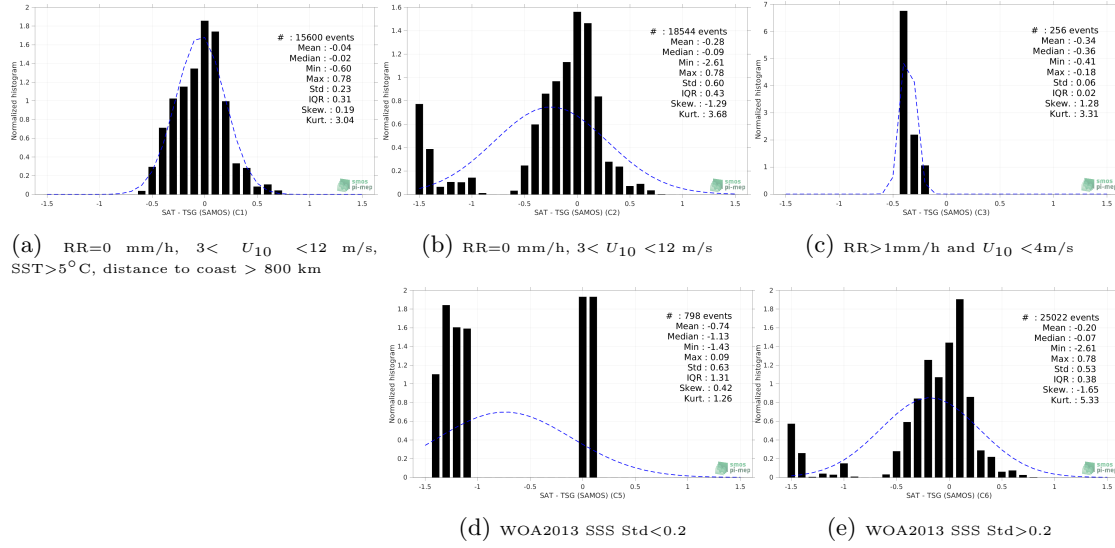
Figure 13: Normalized histogram of \Delta\text{SSS} (SMOS SSS L4 v1 - Weekly (CMEMS-CNR) - TSG (SAMOS)) for 5 different subdatasets corresponding to: RR=0 mm/h, 3 < U_{10} < 12 m/s, SST > 5^\circ\text{C} , distance to coast > 800 km (a), RR=0 mm/h, 3 < U_{10} < 12 m/s (b), RR > 1\text{mm/h} and U_{10} < 4\text{m/s} (c), WOA2013 SSS Std < 0.2 (d), WOA2013 SSS Std > 0.2 (e).
