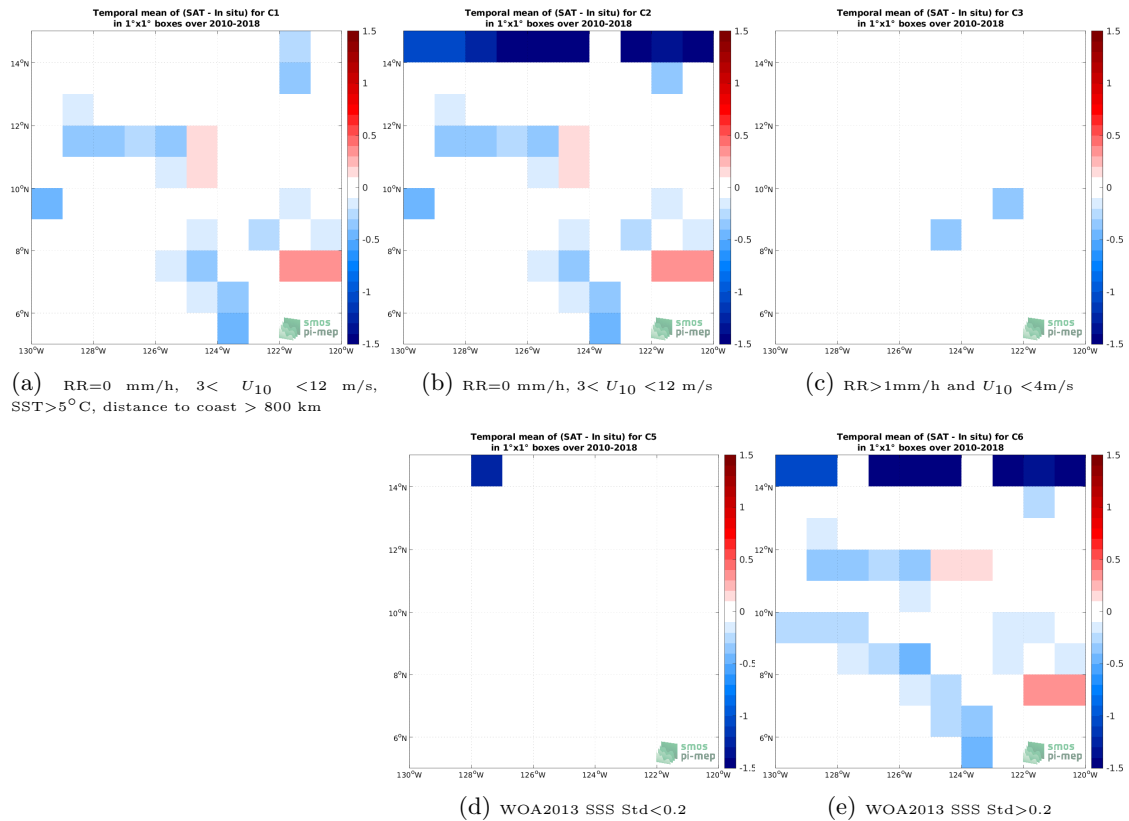
Figure 12: Temporal mean gridded over spatial boxes of size 1^\circ \times 1^\circ of \Delta SSS (SMOS SSS L4 v1 - Weekly (CMEMS-CNR) - TSG (SAMOS)) for 5 different subdatasets corresponding to:RR=0 mm/h, 3 < U_{10} < 12 m/s, SST >5^\circ\text{C} , distance to coast > 800 km (a), RR=0 mm/h, 3 < U_{10} < 12 m/s (b), RR >1 mm/h and U_{10} < 4 m/s (c), WOA2013 SSS Std <0.2 (d), WOA2013 SSS Std >0.2 (e).
