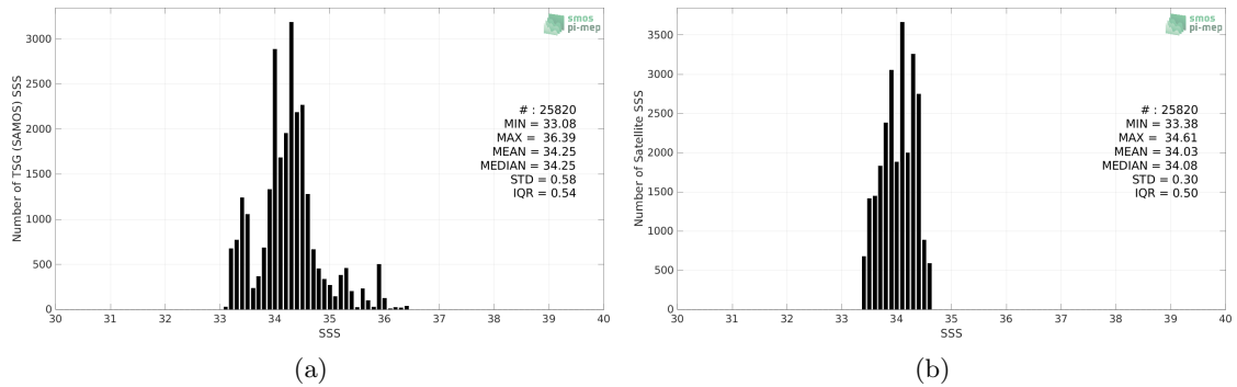
Figure 2: Histograms of SSS from TSG (SAMOS) (a) and SMOS SSS L4 v1 - Weekly (CMEMS-CNR) (b) considering all match-up pairs per bins of 0.1 over the SPURS 2 Pi-MEP region and for the full satellite product period.
