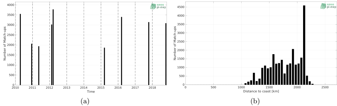
Figure 1: Number of match-ups between TSG (SAMOS) and SMOS SSS L4 v1 - Weekly (CMEMS-CNR) SSS as a function of time (a) and as function of the distance to coast (b) over the SPURS 2 Pi-MEP region and for the full satellite product period.
