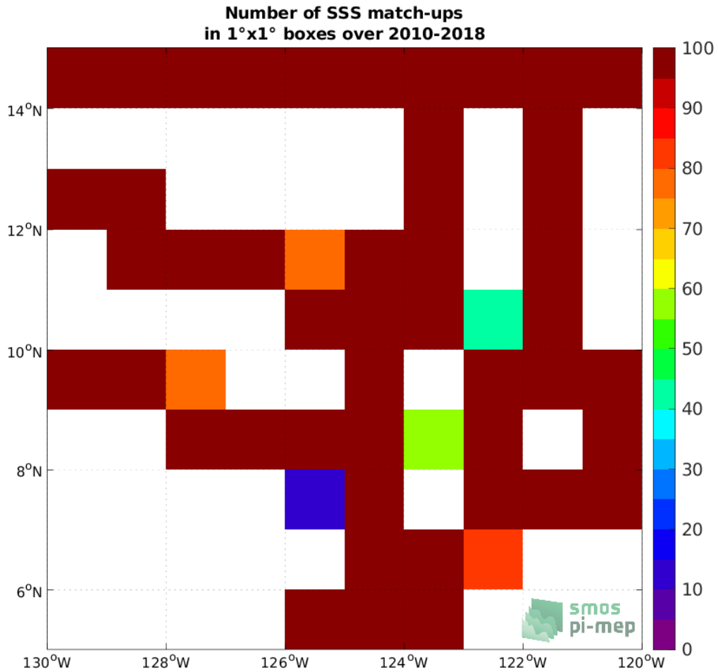
Figure 4: Number of SSS match-ups between TSG (SAMOS) SSS and the SMOS SSS L4 v1 - Weekly (CMEMS-CNR) SSS product for the SPURS 2 Pi-MEP region over 1°x1° boxes and for the full satellite product period.
