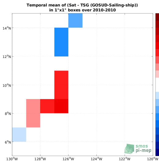
(e) MEAN( \Delta SSS) (Satellite - TSG (GOSUD-Sailing-ship))
