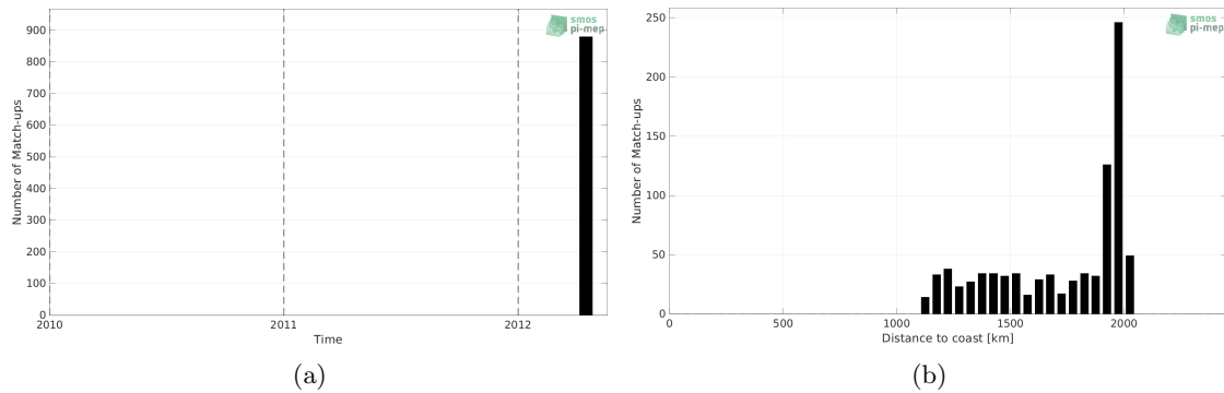
Figure 1: Number of match-ups between TSG (GOSUD-Research-vessel) and SMOS SSS L4 v1 - Weekly (CMEMS-CNR) SSS as a function of time (a) and as function of the distance to coast (b) over the SPURS 2 Pi-MEP region and for the full satellite product period.
