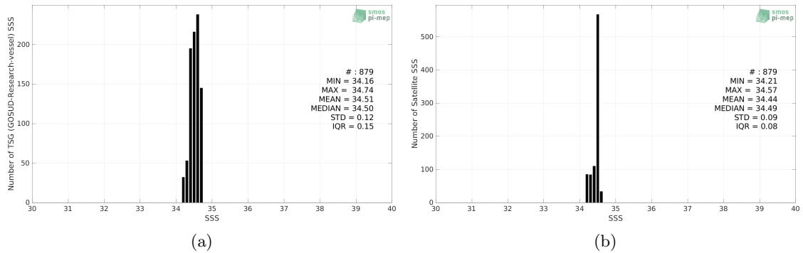
Figure 2: Histograms of SSS from TSG (GOSUD-Research-vessel) (a) and SMOS SSS L4 v1 - Weekly (CMEMS-CNR) (b) considering all match-up pairs per bins of 0.1 over the SPURS 2 Pi-MEP region and for the full satellite product period.
