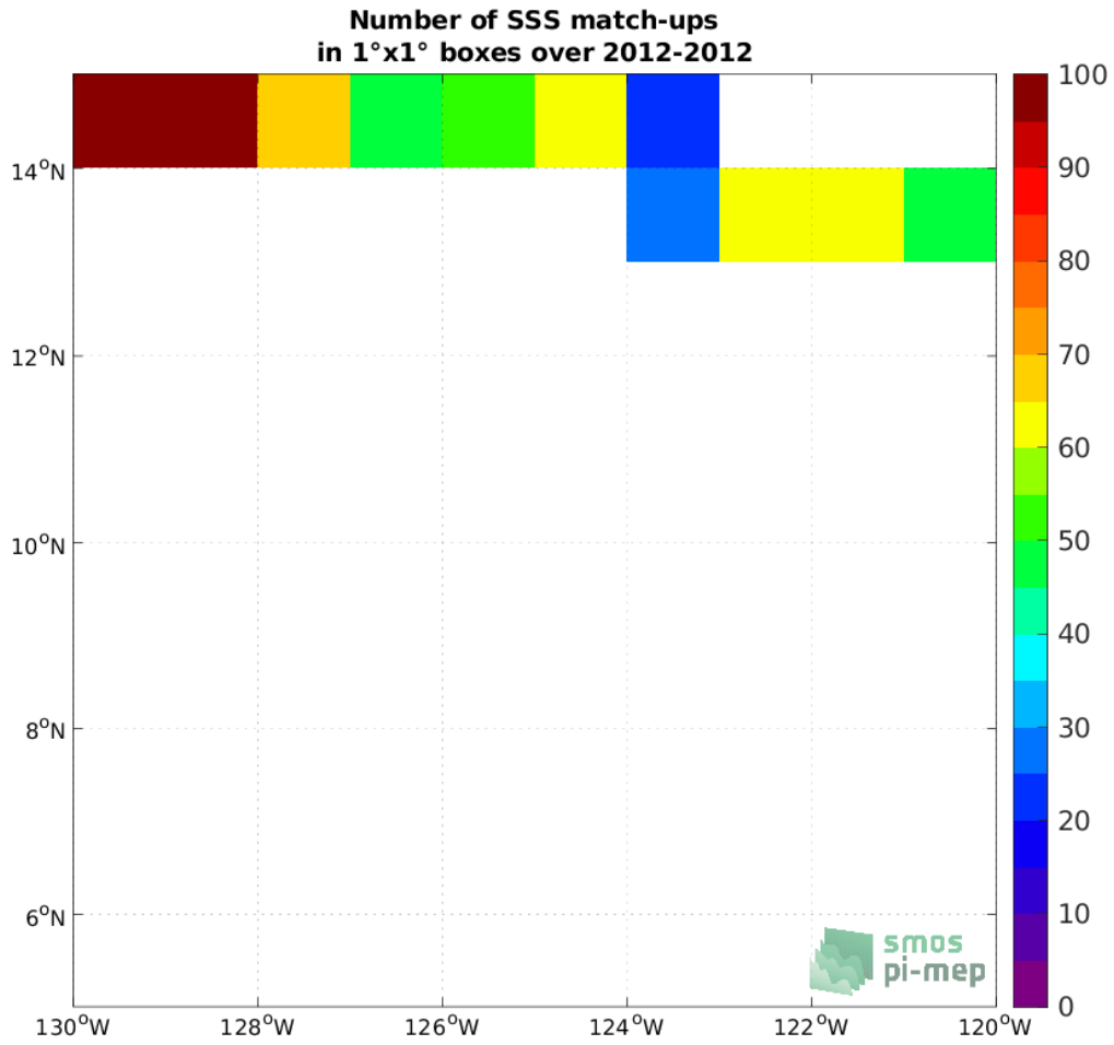
Figure 4: Number of SSS match-ups between TSG (GOSUD-Research-vessel) SSS and the SMOS SSS L4 v1 - Weekly (CMEMS-CNR) SSS product for the SPURS 2 Pi-MEP region over 1°x1° boxes and for the full satellite product period.
