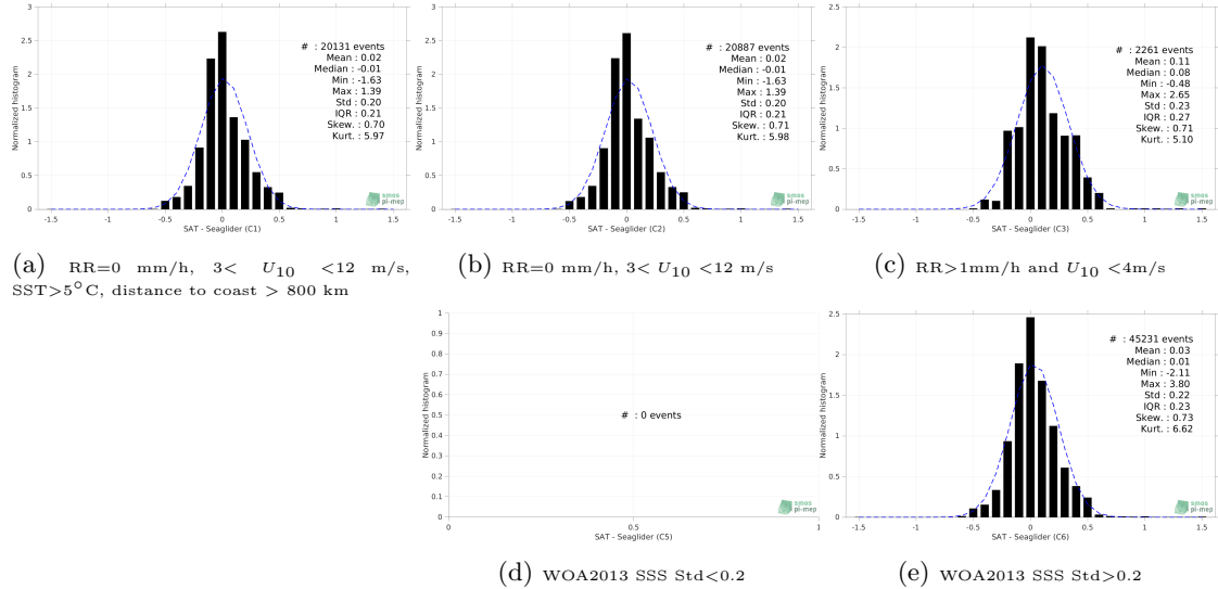
Figure 12: Normalized histogram of \Delta SSS (SMOS SSS L4 v1 - Weekly (CMEMS-CNR) - Seaglider) for 5 different subdatasets corresponding to: RR=0 mm/h, 3 < U_{10} < 12 m/s, SST > 5°C, distance to coast > 800 km (a), RR=0 mm/h, 3 < U_{10} < 12 m/s (b), RR > 1mm/h and U_{10} < 4 m/s (c), WOA2013 SSS Std < 0.2 (d), WOA2013 SSS Std > 0.2 (e).
