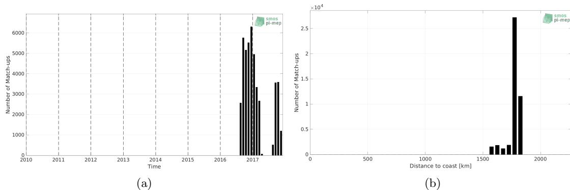
Figure 1: Number of match-ups between Seaglider and SMOS SSS L4 v1 - Weekly (CMEMS-CNR) SSS as a function of time (a) and as function of the distance to coast (b) over the SPURS 2 Pi-MEP region and for the full satellite product period.
