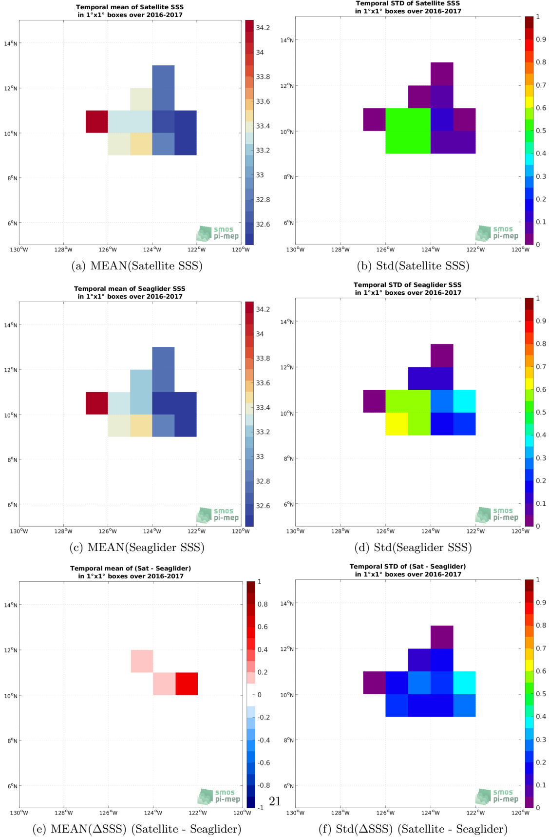
Figure 5: Temporal mean (left) and Std (right) of SSS from SMOS SSS L4 v1 - Weekly (CMEMS-CNR) (top), Seaglider (middle), and of \Delta SSS (Satellite - Seaglider). Only match-up pairs are used to generate these maps.
