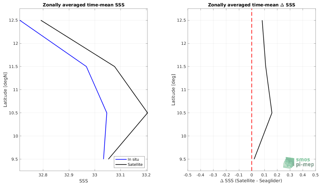
Figure 7: Left panel: Zonal mean SSS from SMOS SSS L4 v1 - Weekly (CMEMS-CNR) satellite product (black) and from Seaglider (blue). Right panel: Zonal mean of \Delta SSS (Satellite - Seaglider) for all the collected Pi-MEP match-up pairs estimated over the full satellite product period.
