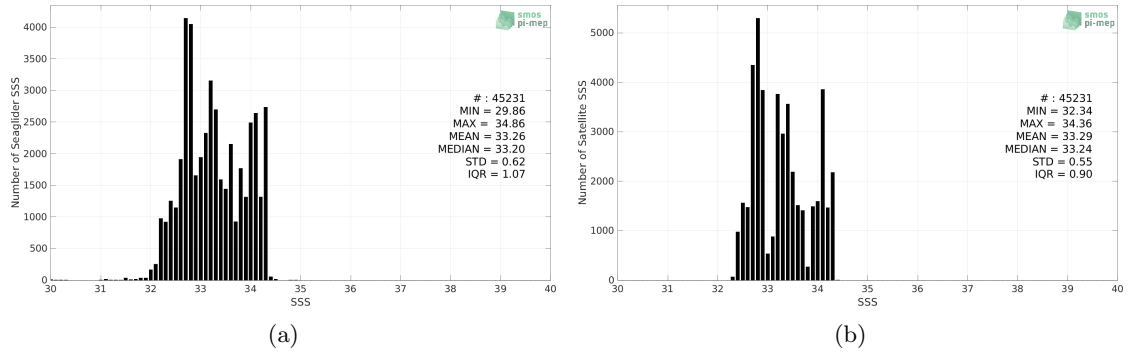
Figure 2: Histograms of SSS from Seaglider (a) and SMOS SSS L4 v1 - Weekly (CMEMS-CNR) (b) considering all match-up pairs per bins of 0.1 over the SPURS 2 Pi-MEP region and for the full satellite product period.
