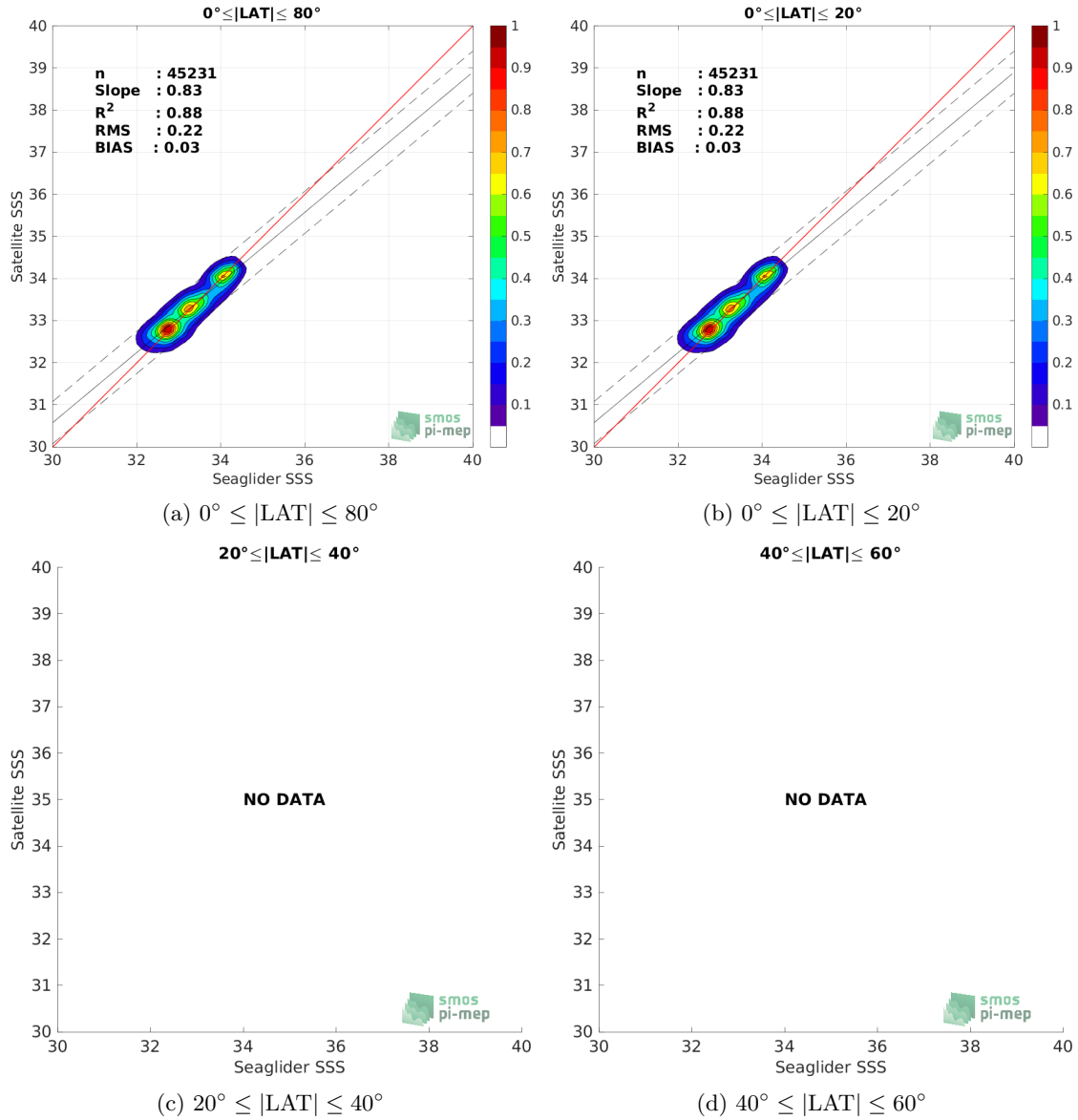
Figure 8: Contour maps of the concentration of SMOS SSS L4 v1 - Weekly (CMEMS-CNR) SSS (y-axis) versus Seaglider SSS (x-axis) at match-up pairs for different latitude bands. For each plot, the red line shows x=y . The black thin and dashed lines indicate a linear fit through the data cloud and the \pm 95\% confidence levels, respectively. The number match-up pairs n , the slope and R^2 coefficient of the linear fit, the root mean square (RMS) and the mean bias between satellite and in situ data are indicated for each latitude band in each plots.
