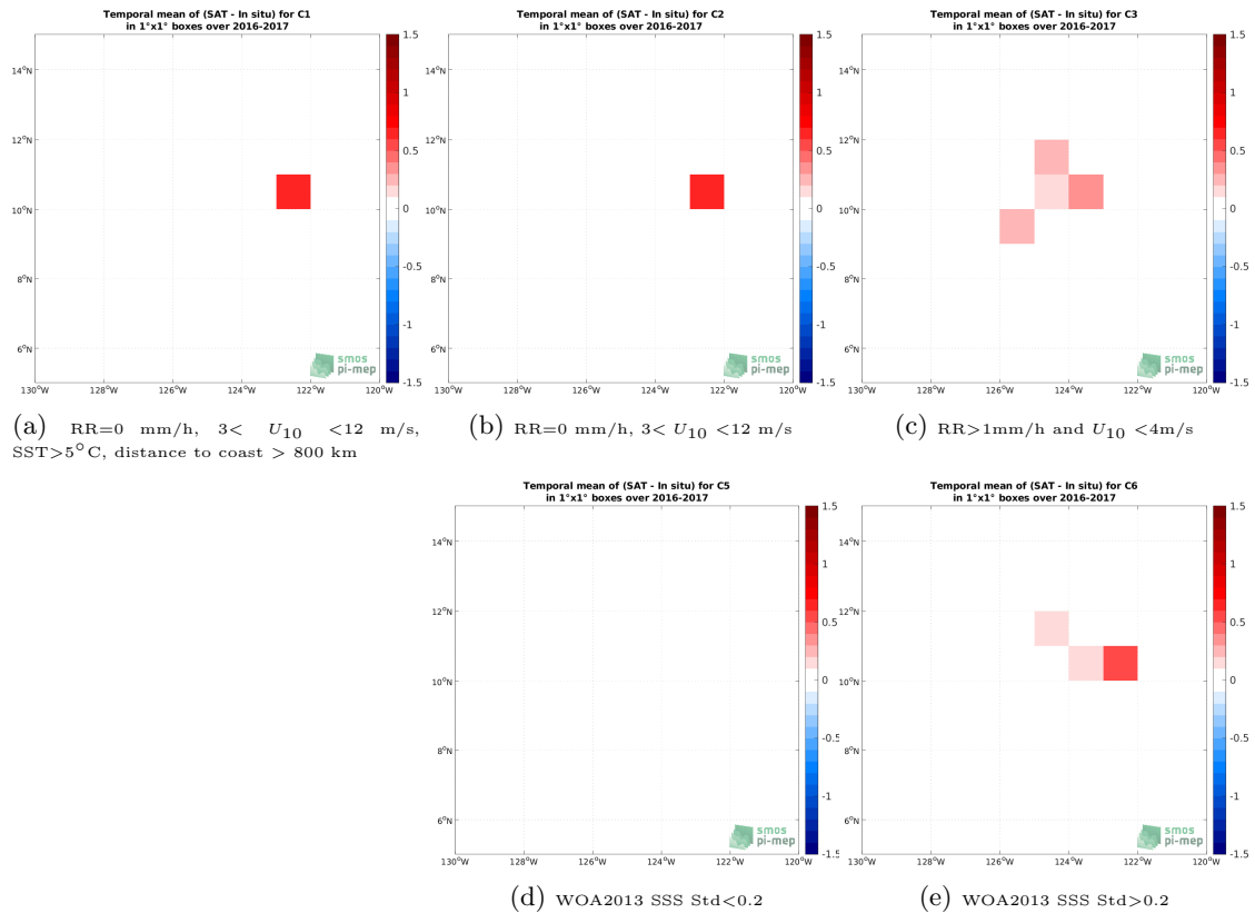
Figure 11: Temporal mean gridded over spatial boxes of size 1^\circ \times 1^\circ of \Delta SSS (SMOS SSS L4 v1 - Weekly (CMEMS-CNR) - Seaglider) for 5 different subdatasets corresponding to:RR=0 mm/h, 3 < U_{10} < 12 m/s, SST >5^\circ C, distance to coast > 800 km (a), RR=0 mm/h, 3 < U_{10} < 12 m/s (b), RR >1 mm/h and U_{10} < 4 m/s (c), WOA2013 SSS Std <0.2 (d), WOA2013 SSS Std >0.2 (e).
