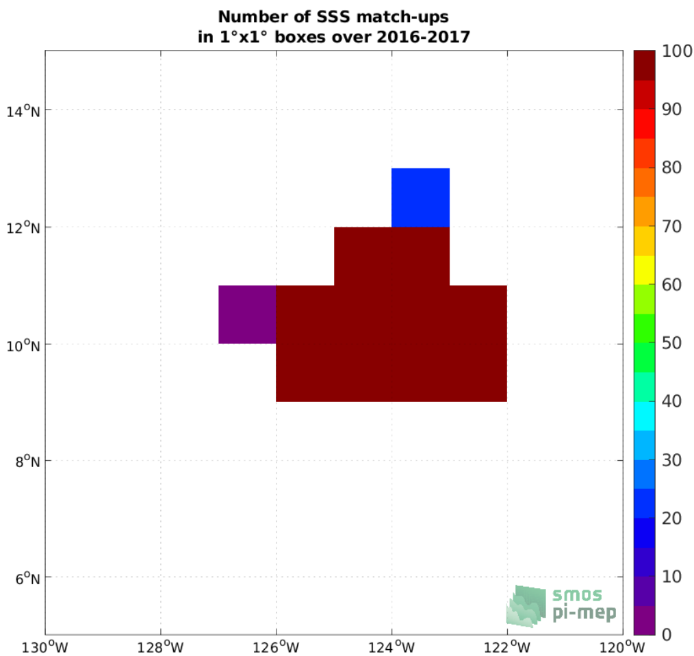
Figure 3: Number of SSS match-ups between Seaglider SSS and the SMOS SSS L4 v1 - Weekly (CMEMS-CNR) SSS product for the SPURS 2 Pi-MEP region over 1°x1° boxes and for the full satellite product period.
