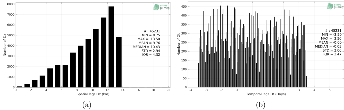
Figure 4: Histograms of the spatial (a) and temporal (b) lags between the location/time of the Seaglider measurement and the date of the corresponding SMOS SSS L4 v1 - Weekly (CMEMS-CNR) SSS pixel.
