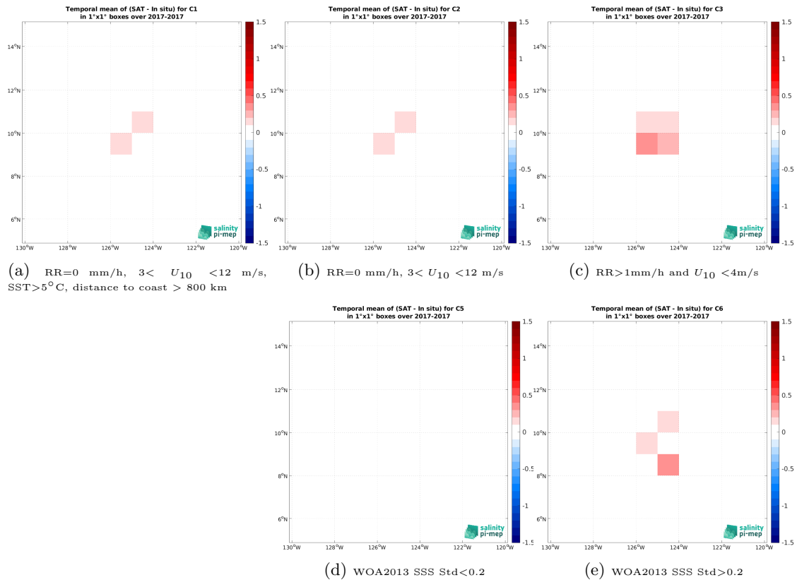
Figure 12: Temporal mean gridded over spatial boxes of size 1^\circ \times 1^\circ of \Delta SSS (SMOS SSS L4 v1 - Weekly (CMEMS-CNR) - Sailability (SPURS 2)) for 5 different subdatasets corresponding to:RR=0 mm/h, 3 < U_{10} < 12 m/s, SST >5^\circ C, distance to coast > 800 km (a), RR=0 mm/h, 3 < U_{10} < 12 m/s (b), RR >1 mm/h and U_{10} < 4 m/s (c), WOA2013 SSS Std <0.2 (d), WOA2013 SSS Std >0.2 (e).
