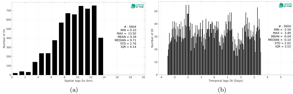
Figure 5: Histograms of the spatial (a) and temporal (b) lags between the location/time of the Saildrone (SPURS 2) measurement and the date of the corresponding SMOS SSS L4 v1 - Weekly (CMEMS-CNR) SSS pixel.
