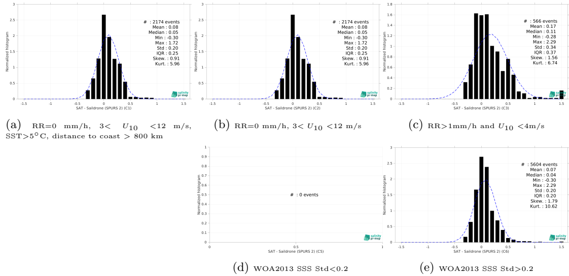
Figure 13: Normalized histogram of \Delta SSS (SMOS SSS L4 v1 - Weekly (CMEMS-CNR) - Saildrone (SPURS 2)) for 5 different subdatasets corresponding to: RR=0 mm/h, 3 < U_{10} < 12 m/s, SST>5°C, distance to coast > 800 km (a), RR=0 mm/h, 3 < U_{10} < 12 m/s (b), RR>1mm/h and U_{10} < 4 m/s (c), WOA2013 SSS Std<0.2 (d), WOA2013 SSS Std>0.2 (e).
