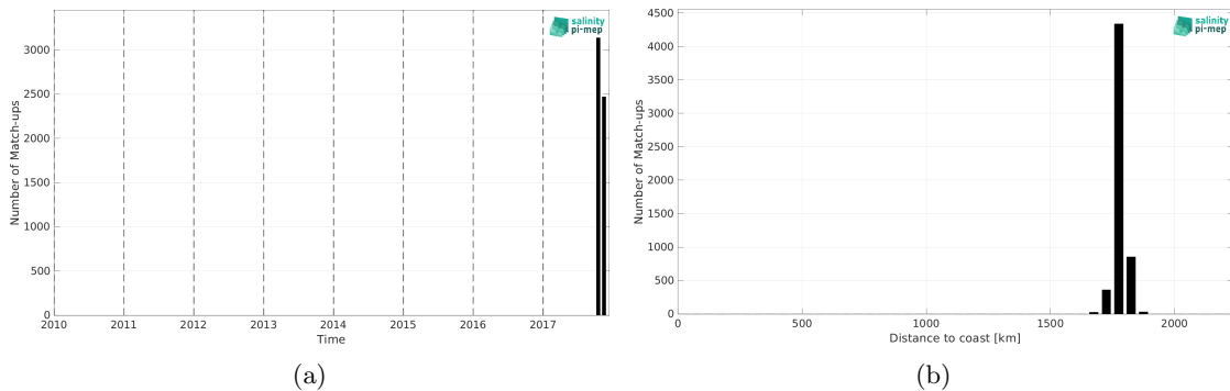
Figure 1: Number of match-ups between Saildrone (SPURS 2) and SMOS SSS L4 v1 - Weekly (CMEMS-CNR) SSS as a function of time (a) and as function of the distance to coast (b) over the SPURS 2 Pi-MEP region and for the full satellite product period.
