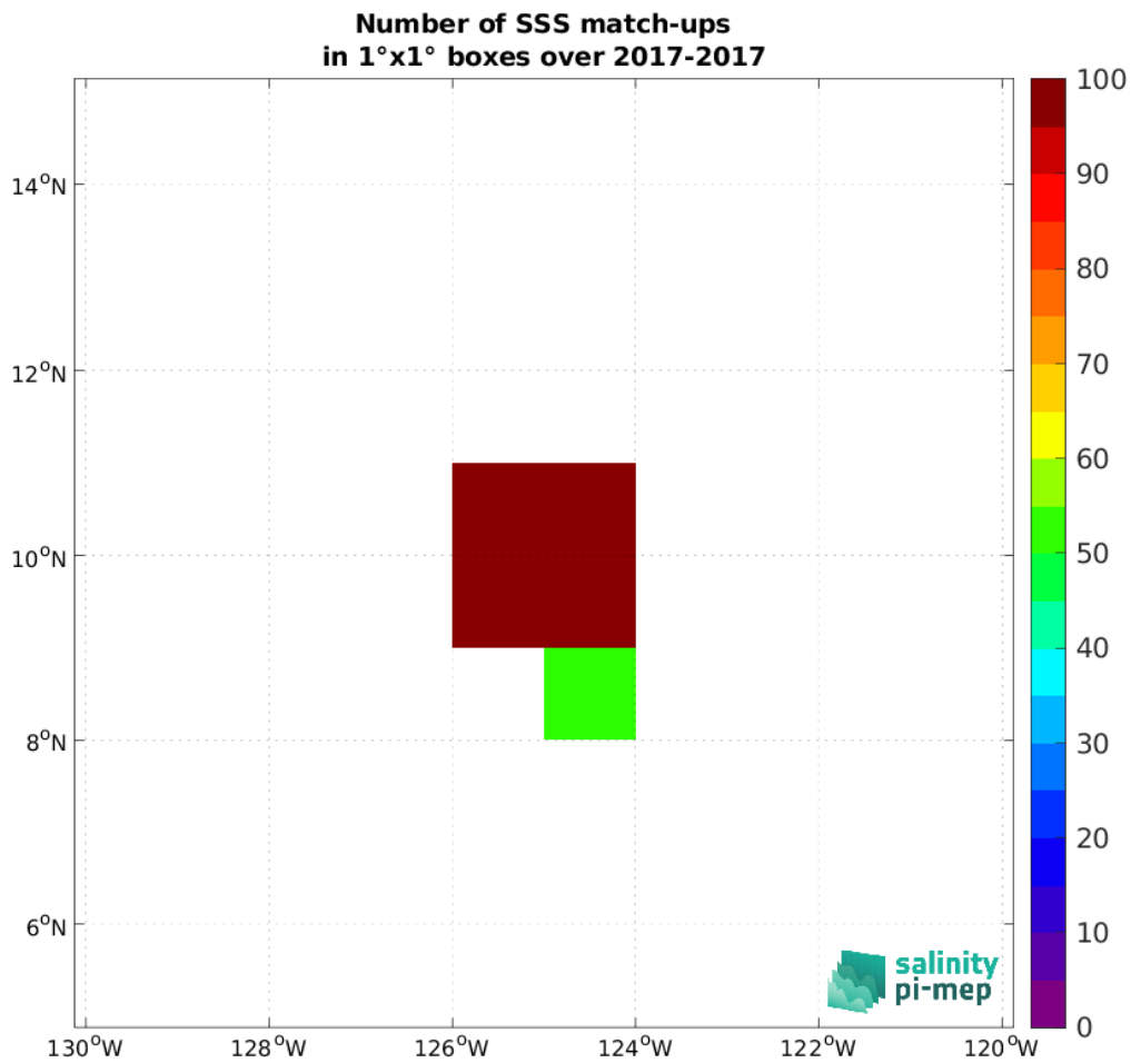
Figure 4: Number of SSS match-ups between Saildrone (SPURS 2) SSS and the SMOS SSS L4 v1 - Weekly (CMEMS-CNR) SSS product for the SPURS 2 Pi-MEP region over 1°x1° boxes and for the full satellite product period.
