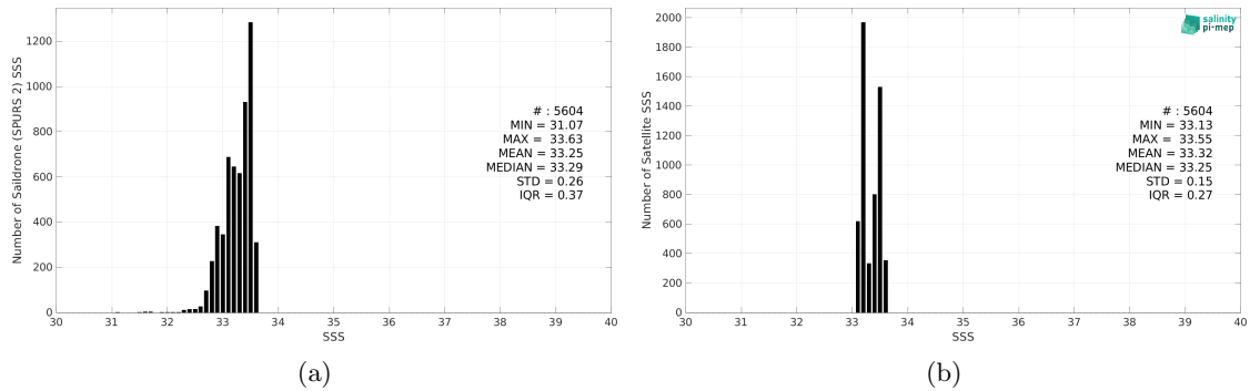
Figure 2: Histograms of SSS from Saildrone (SPURS 2) (a) and SMOS SSS L4 v1 - Weekly (CMEMS-CNR) (b) considering all match-up pairs per bins of 0.1 over the SPURS 2 Pi-MEP region and for the full satellite product period.
