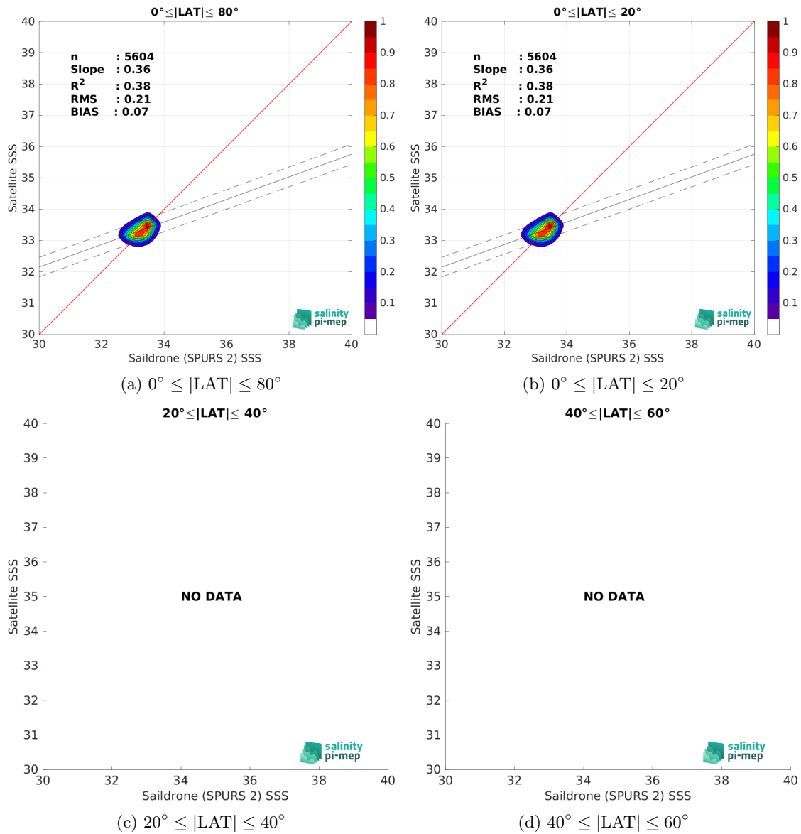
Figure 9: Contour maps of the concentration of SMOS SSS L4 v1 - Weekly (CMEMS-CNR) SSS (y-axis) versus Saildrone (SPURS 2) SSS (x-axis) at match-up pairs for different latitude bands. For each plot, the red line shows x=y . The black thin and dashed lines indicate a linear fit through the data cloud and the \pm 95\% confidence levels, respectively. The number match-up pairs n , the slope and R^2 coefficient of the linear fit, the root mean square (RMS) and the mean bias between satellite and in situ data are indicated for each latitude band in each plots.
