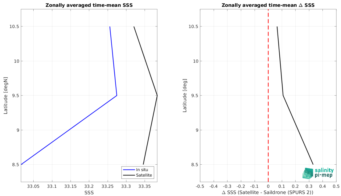
Figure 8: Left panel: Zonal mean SSS from SMOS SSS L4 v1 - Weekly (CMEMS-CNR) satellite product (black) and from Sairdron (SPURS 2) (blue). Right panel: Zonal mean of \Delta SSS (Satellite - Sairdron (SPURS 2)) for all the collected Pi-MEP match-up pairs estimated over the full satellite product period.
