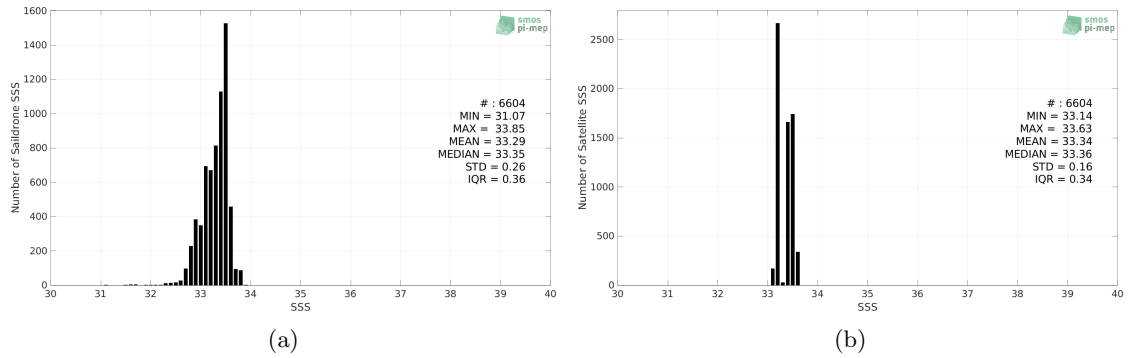
Figure 2: Histograms of SSS from Sairdrone (a) and SMOS SSS L4 v1 - Weekly (CMEMS-CNR) (b) considering all match-up pairs per bins of 0.1 over the SPURS 2 Pi-MEP region and for the full satellite product period.
