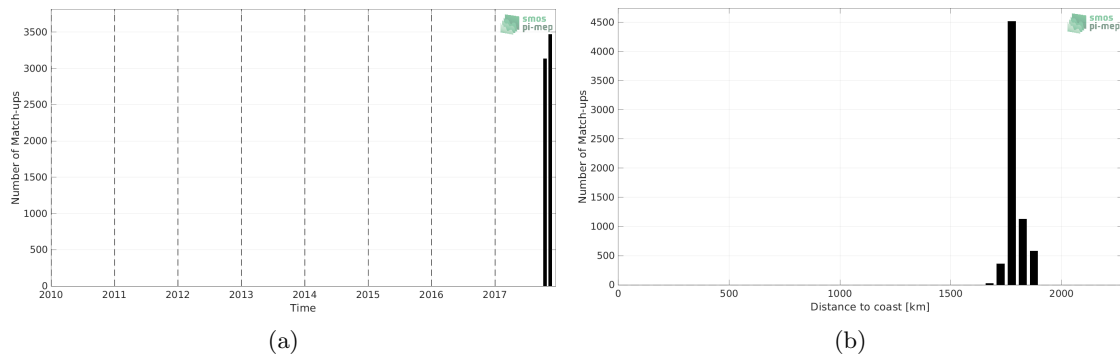
Figure 1: Number of match-ups between Saildrone and SMOS SSS L4 v1 - Weekly (CMEMS-CNR) SSS as a function of time (a) and as function of the distance to coast (b) over the SPURS 2 Pi-MEP region and for the full satellite product period.
