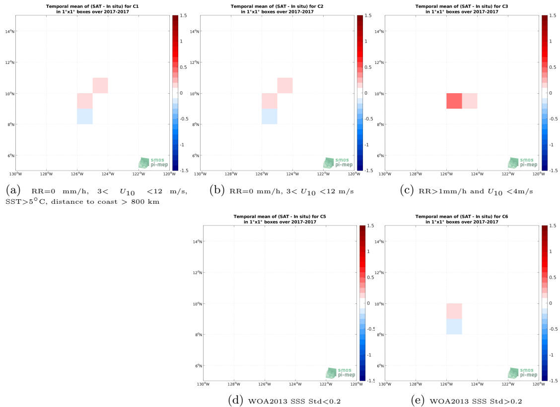
Figure 11: Temporal mean gridded over spatial boxes of size 1^\circ \times 1^\circ of \Delta SSS (SMOS SSS L4 v1 - Weekly (CMEMS-CNR) - Saildrone) for 5 different subdatasets corresponding to:RR=0 mm/h, 3 < U_{10} < 12 m/s, SST >5^\circ C, distance to coast > 800 km (a), RR=0 mm/h, 3 < U_{10} < 12 m/s (b), RR >1 mm/h and U_{10} < 4 m/s (c), WOA2013 SSS Std <0.2 (d), WOA2013 SSS Std >0.2 (e).
