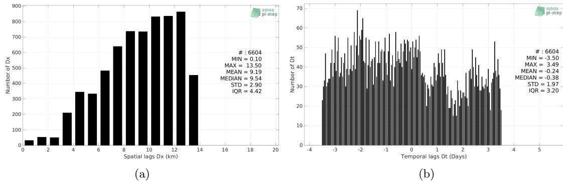
Figure 4: Histograms of the spatial (a) and temporal (b) lags between the location/time of the Saildrone measurement and the date of the corresponding SMOS SSS L4 v1 - Weekly (CMEMS-CNR) SSS pixel.
