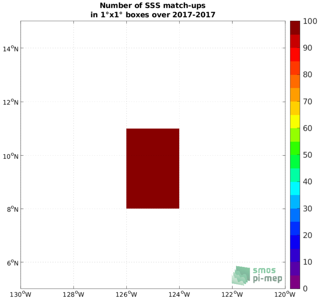
Figure 3: Number of SSS match-ups between Saildrone SSS and the SMOS SSS L4 v1 - Weekly (CMEMS-CNR) SSS product for the SPURS 2 Pi-MEP region over 1^\circ \times 1^\circ boxes and for the full satellite product period.
