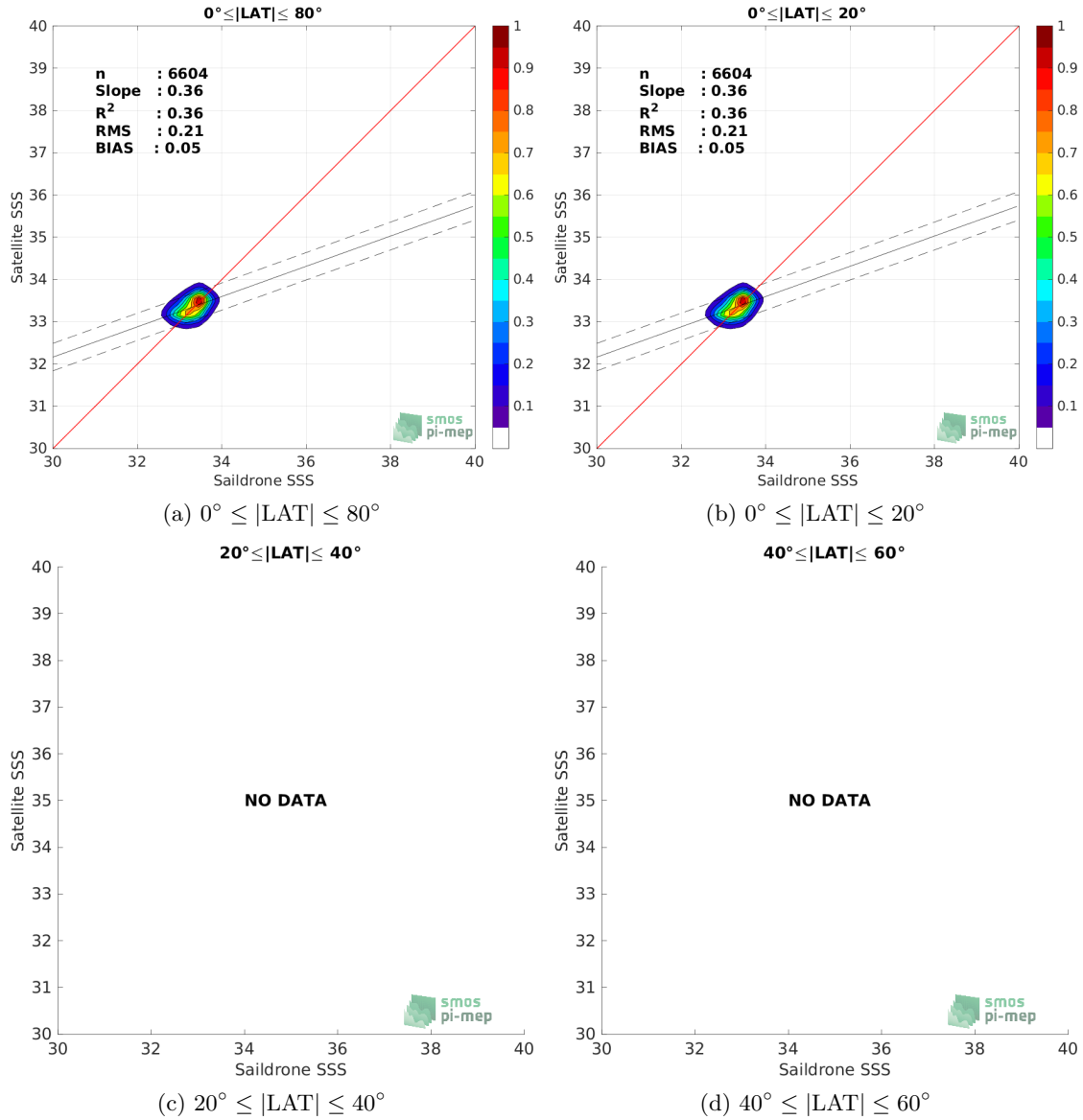
Figure 8: Contour maps of the concentration of SMOS SSS L4 v1 - Weekly (CMEMS-CNR) SSS (y-axis) versus Saildrone SSS (x-axis) at match-up pairs for different latitude bands. For each plot, the red line shows x=y . The black thin and dashed lines indicate a linear fit through the data cloud and the \pm 95\% confidence levels, respectively. The number match-up pairs n , the slope and R^2 coefficient of the linear fit, the root mean square (RMS) and the mean bias between satellite and in situ data are indicated for each latitude band in each plots.
