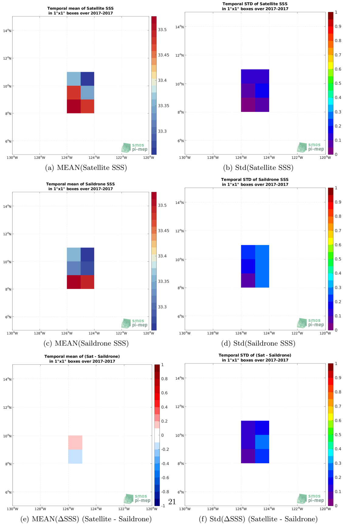
Figure 5: Temporal mean (left) and Std (right) of SSS from SMOS SSS L4 v1 - Weekly (CMEMS-CNR) (top), Saildrone (middle), and of \Delta SSS (Satellite - Saildrone). Only match-up pairs are used to generate these maps.
