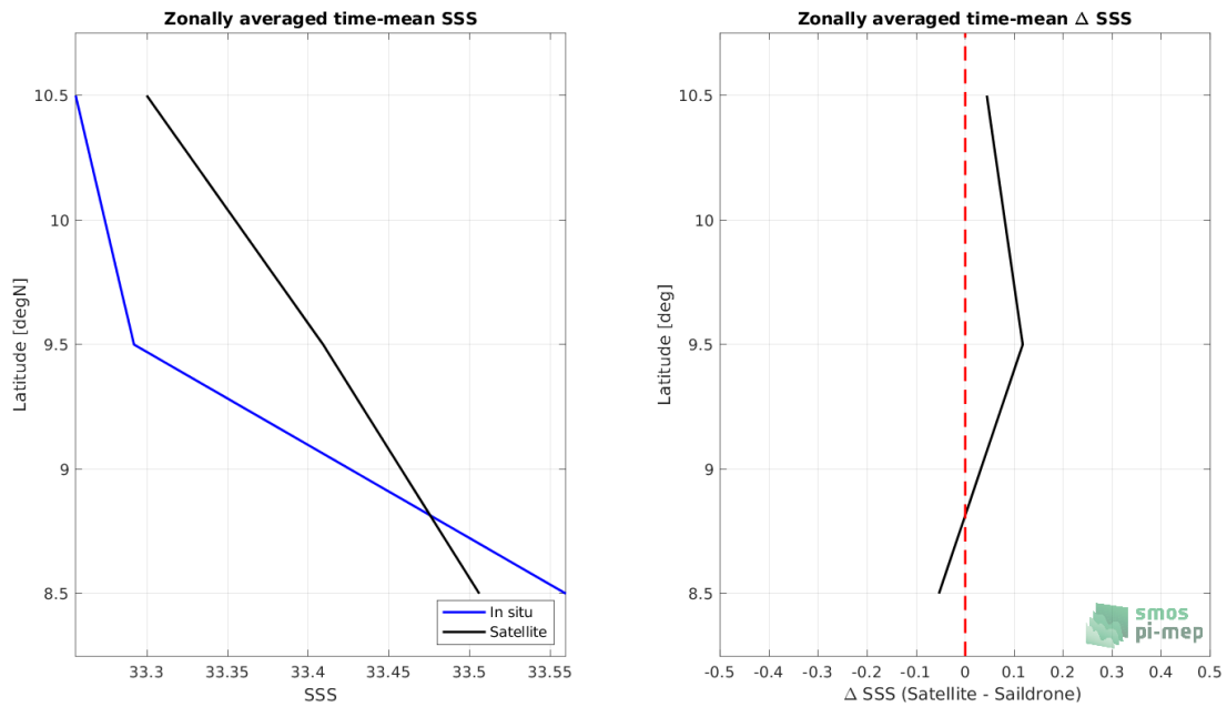
Figure 7: Left panel: Zonal mean SSS from SMOS SSS L4 v1 - Weekly (CMEMS-CNR) satellite product (black) and from Sairdron (blue). Right panel: Zonal mean of \Delta SSS (Satellite - Sairdron) for all the collected Pi-MEP match-up pairs estimated over the full satellite product period.
