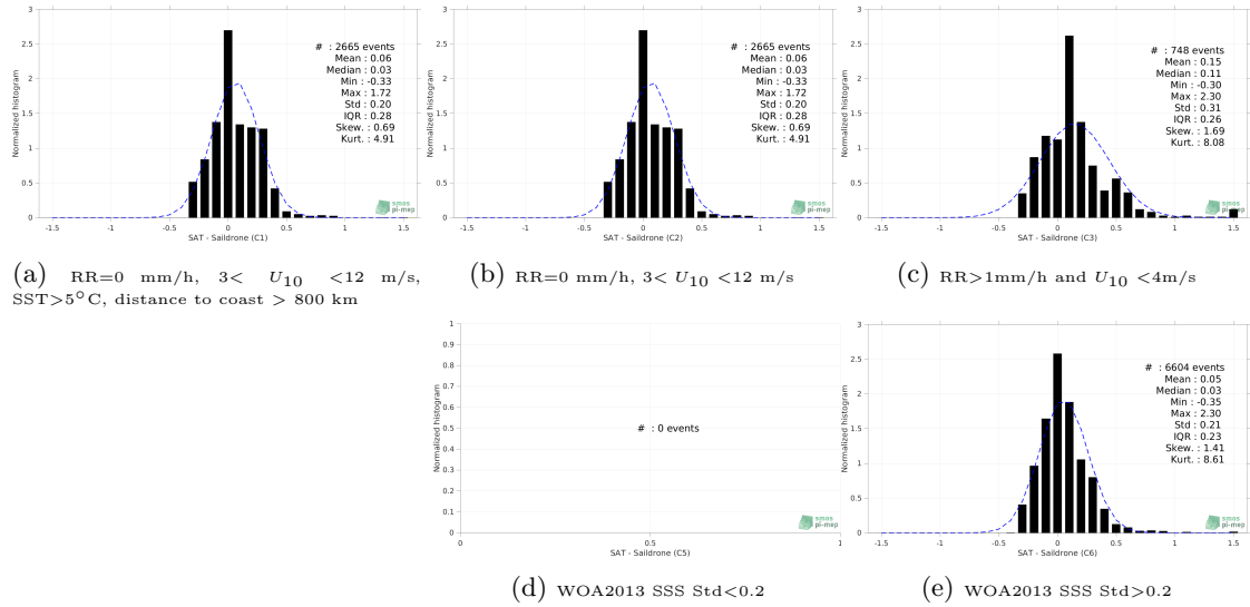
Figure 12: Normalized histogram of \Delta SSS (SMOS SSS L4 v1 - Weekly (CMEMS-CNR) - Saildrone) for 5 different subdatasets corresponding to: RR=0 mm/h, 3 < U_{10} < 12 m/s, SST > 5°C, distance to coast > 800 km (a), RR=0 mm/h, 3 < U_{10} < 12 m/s (b), RR > 1mm/h and U_{10} < 4 m/s (c), WOA2013 SSS Std < 0.2 (d), WOA2013 SSS Std > 0.2 (e).
