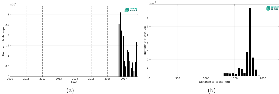
Figure 2: Number of match-ups between Waveglider (SPURS 2) and SMOS SSS L4 v1 - Monthly (CMEMS-CNR) SSS as a function of time (a) and as function of the distance to coast (b) over the SPURS 2 Pi-MEP region and for the full satellite product period.
