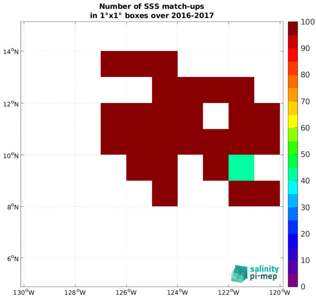
Figure 5: Number of SSS match-ups between Waveglider (SPURS 2) SSS and the SMOS SSS L4 v1 - Monthly (CMEMS-CNR) SSS product for the SPURS 2 Pi-MEP region over 1°x1° boxes and for the full satellite product period.
