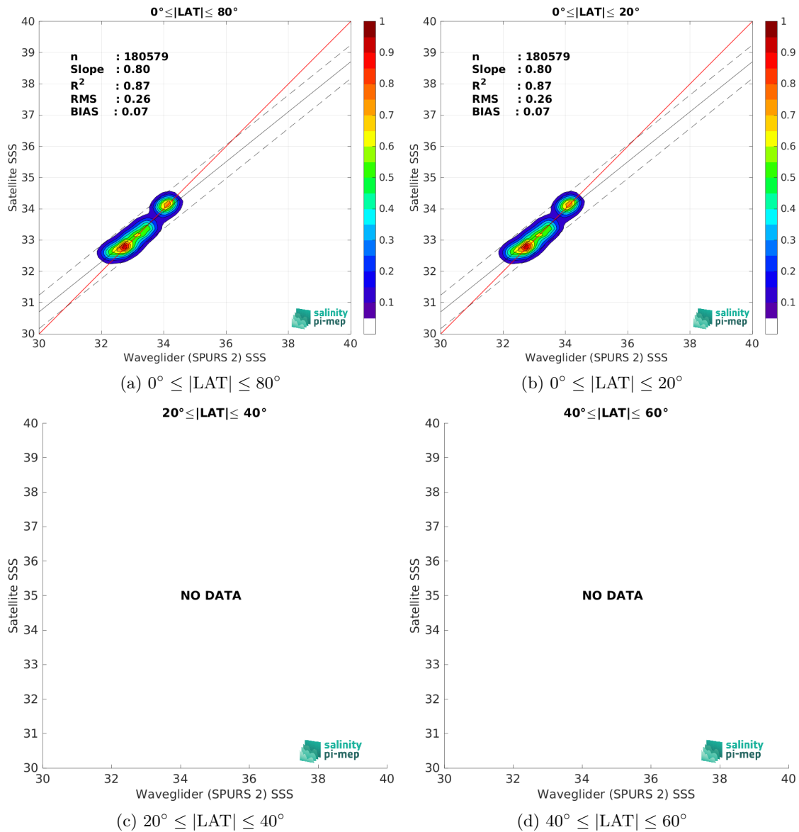
Figure 10: Contour maps of the concentration of SMOS SSS L4 v1 - Monthly (CMEMS-CNR) SSS (y-axis) versus Waveglider (SPURS 2) SSS (x-axis) at match-up pairs for different latitude bands. For each plot, the red line shows x=y . The black thin and dashed lines indicate a linear fit through the data cloud and the \pm 95\% confidence levels, respectively. The number match-up pairs n , the slope and R^2 coefficient of the linear fit, the root mean square (RMS) and the mean bias between satellite and in situ data are indicated for each latitude band in each plots.
