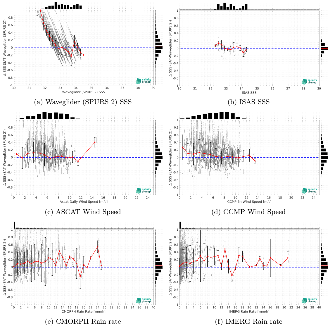
Figure 12: \Delta \text{SSS} (Satellite - Waveglider (SPURS 2)) sorted as function of Waveglider (SPURS 2) SSS values (a), ISAS SSS (b), ASCAT Wind speed (c), CCMP Wind speed (d), CMORPH rain rate (e) and IMERG rain rate (f). In all plots the median and Std of \Delta \text{SSS} for each bin is indicated by the red curves and black vertical thick bars ( \pm 1 \text{ Std} ).
