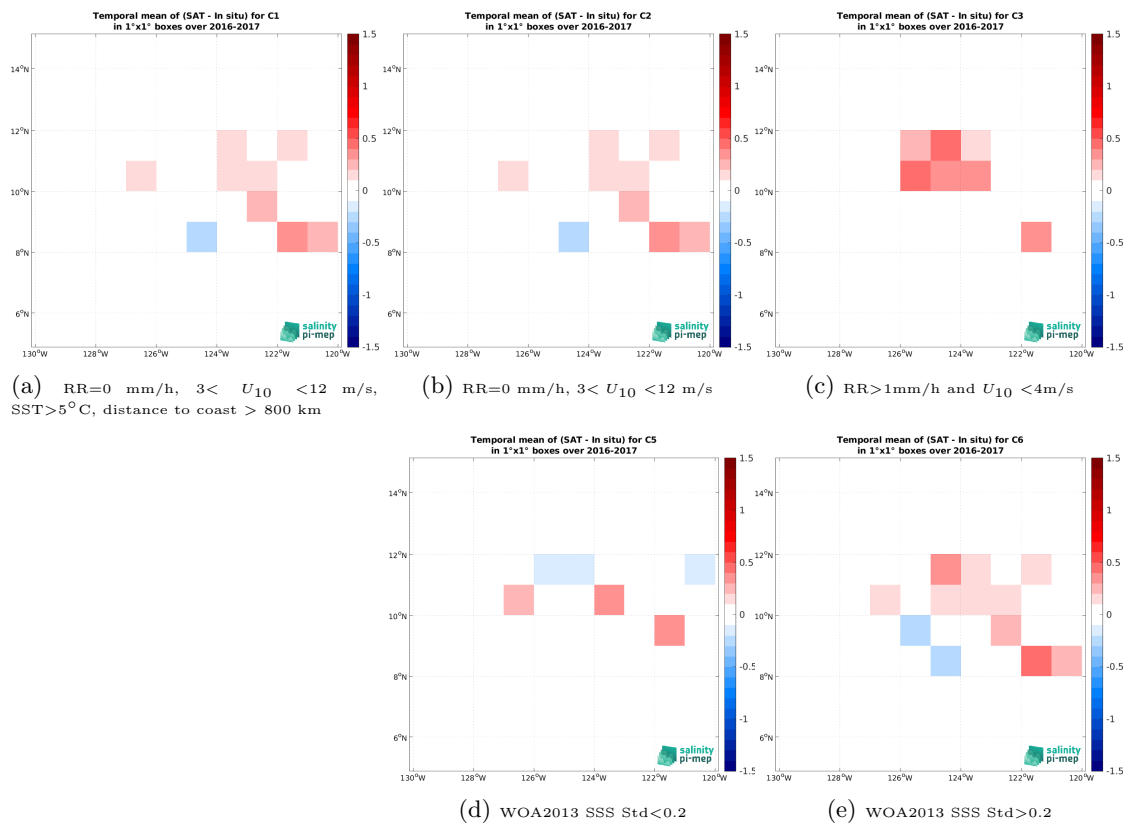
Figure 14: Temporal mean gridded over spatial boxes of size 1^\circ \times 1^\circ of \Delta SSS (SMOS SSS L4 v1 - Monthly (CMEMS-CNR) - Waveglider (SPURS 2)) for 5 different subdatasets corresponding to: RR=0 mm/h, 3 < U_{10} < 12 m/s, SST > 5°C, distance to coast > 800 km (a), RR=0 mm/h, 3 < U_{10} < 12 m/s (b), RR > 1mm/h and U_{10} < 4 m/s (c), WOA2013 SSS Std < 0.2 (d), WOA2013 SSS Std > 0.2 (e).
