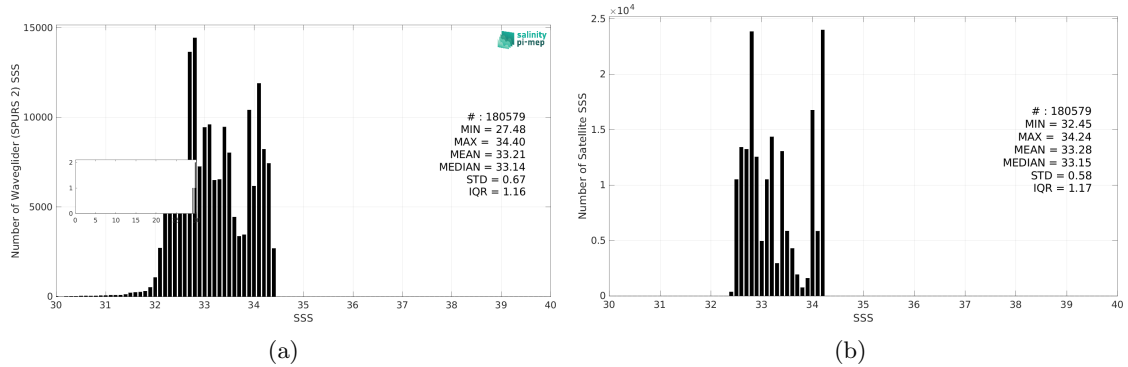
Figure 3: Histograms of SSS from Waveglider (SPURS 2) (a) and SMOS SSS L4 v1 - Monthly (CMEMS-CNR) (b) considering all match-up pairs per bins of 0.1 over the SPURS 2 Pi-MEP region and for the full satellite product period.
