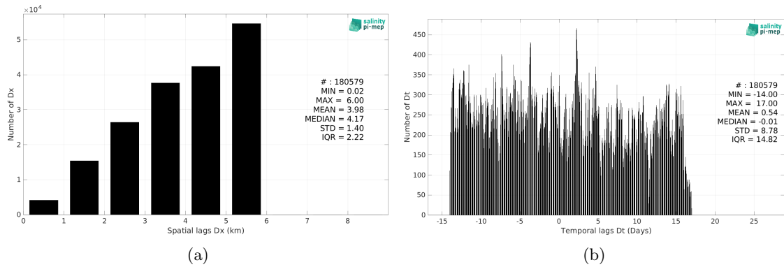
Figure 6: Histograms of the spatial (a) and temporal (b) lags between the location/time of the Waveglider (SPURS 2) measurement and the date of the corresponding SMOS SSS L4 v1 - Monthly (CMEMS-CNR) SSS pixel.
