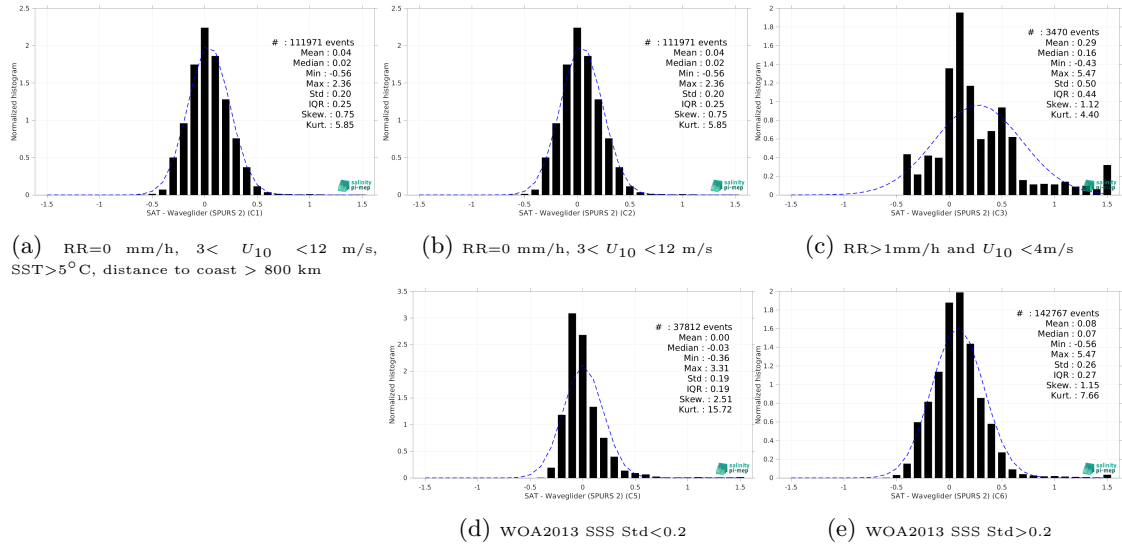
Figure 15: Normalized histogram of \Delta SSS (SMOS SSS L4 v1 - Monthly (CMEMS-CNR) - Waveglider (SPURS 2)) for 5 different subdatasets corresponding to: RR=0 mm/h, 3 < U_{10} < 12 m/s, SST > 5°C, distance to coast > 800 km (a), RR=0 mm/h, 3 < U_{10} < 12 m/s (b), RR > 1mm/h and U_{10} < 4 m/s (c), WOA2013 SSS Std < 0.2 (d), WOA2013 SSS Std > 0.2 (e).
