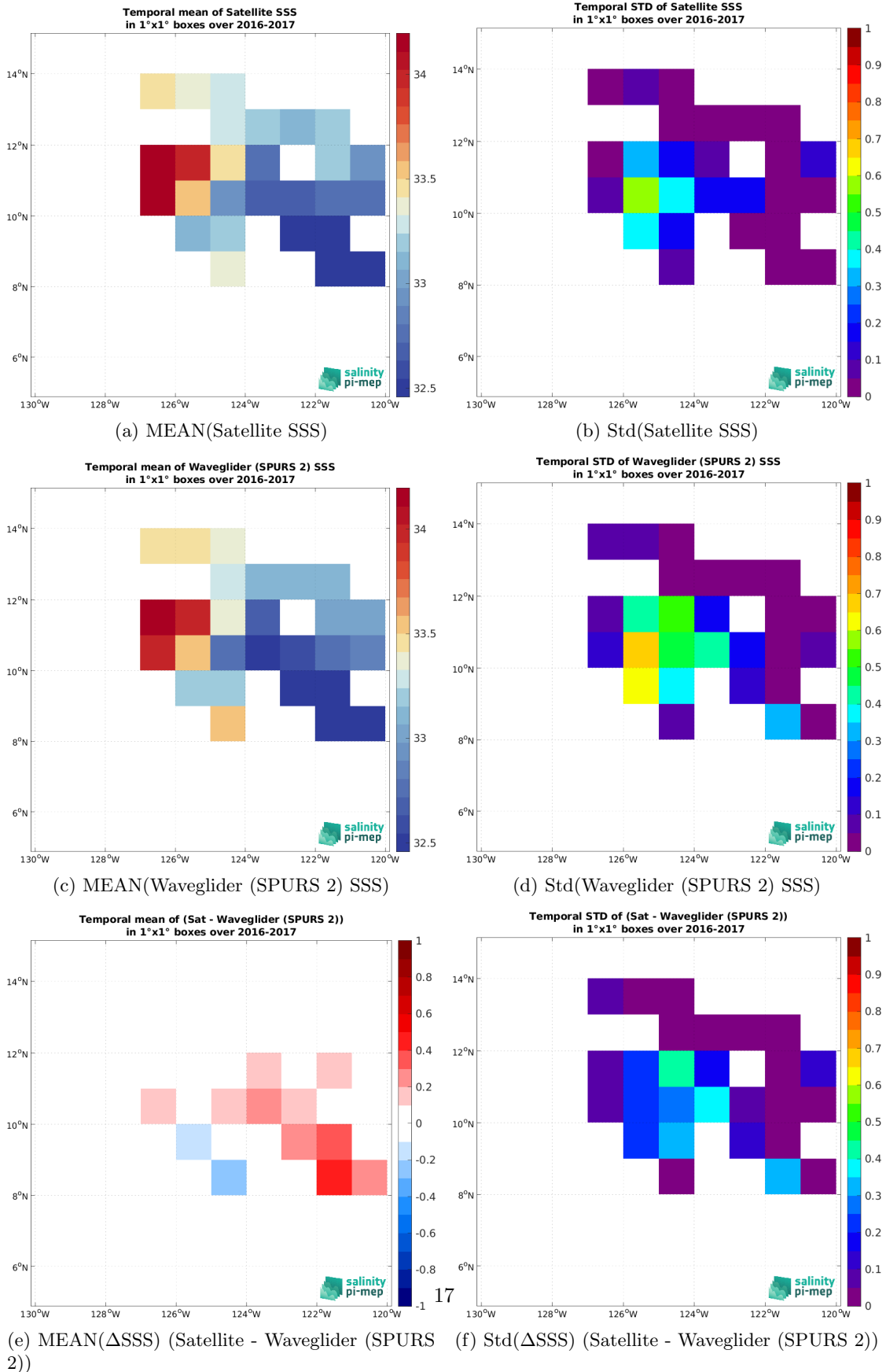
Figure 7: Temporal mean (left) and Std (right) of SSS from SMOS SSS L4 v1 - Monthly (CMEMS-CNR) (top), Waveglider (SPURS 2) (middle), and of \Delta SSS (Satellite - Waveglider (SPURS 2)). Only match-up pairs are used to generate these maps.
