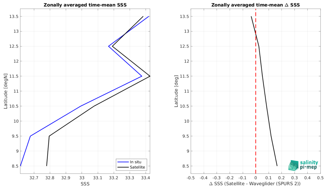
Figure 9: Left panel: Zonal mean SSS from SMOS SSS L4 v1 - Monthly (CMEMS-CNR) satellite product (black) and from Waveglider (SPURS 2) (blue). Right panel: Zonal mean of \Delta SSS (Satellite - Waveglider (SPURS 2)) for all the collected Pi-MEP match-up pairs estimated over the full satellite product period.
