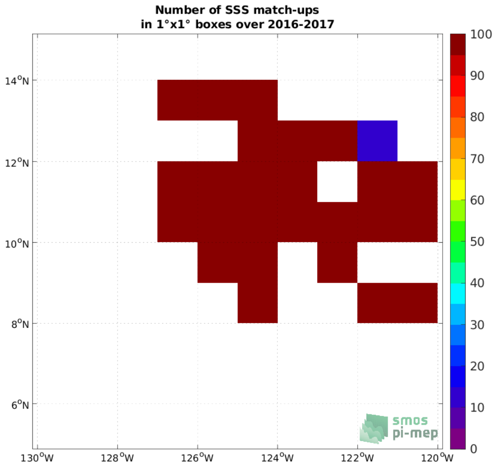
Figure 3: Number of SSS match-ups between Waveglider (SPURS 2) SSS and the SMOS SSS L4 v1 - Monthly (CMEMS-CNR) SSS product for the SPURS 2 Pi-MEP region over 1°x1° boxes and for the full satellite product period.
