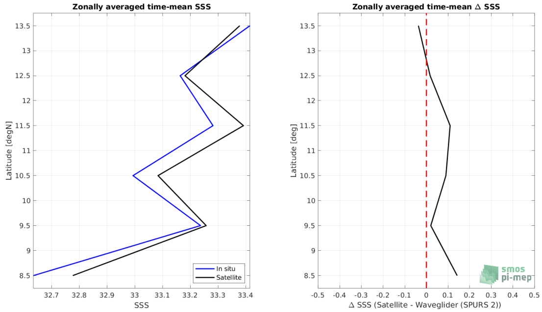
Figure 7: Left panel: Zonal mean SSS from SMOS SSS L4 v1 - Monthly (CMEMS-CNR) satellite product (black) and from Waveglider (SPURS 2) (blue). Right panel: Zonal mean of \Delta SSS (Satellite - Waveglider (SPURS 2)) for all the collected Pi-MEP match-up pairs estimated over the full satellite product period.
