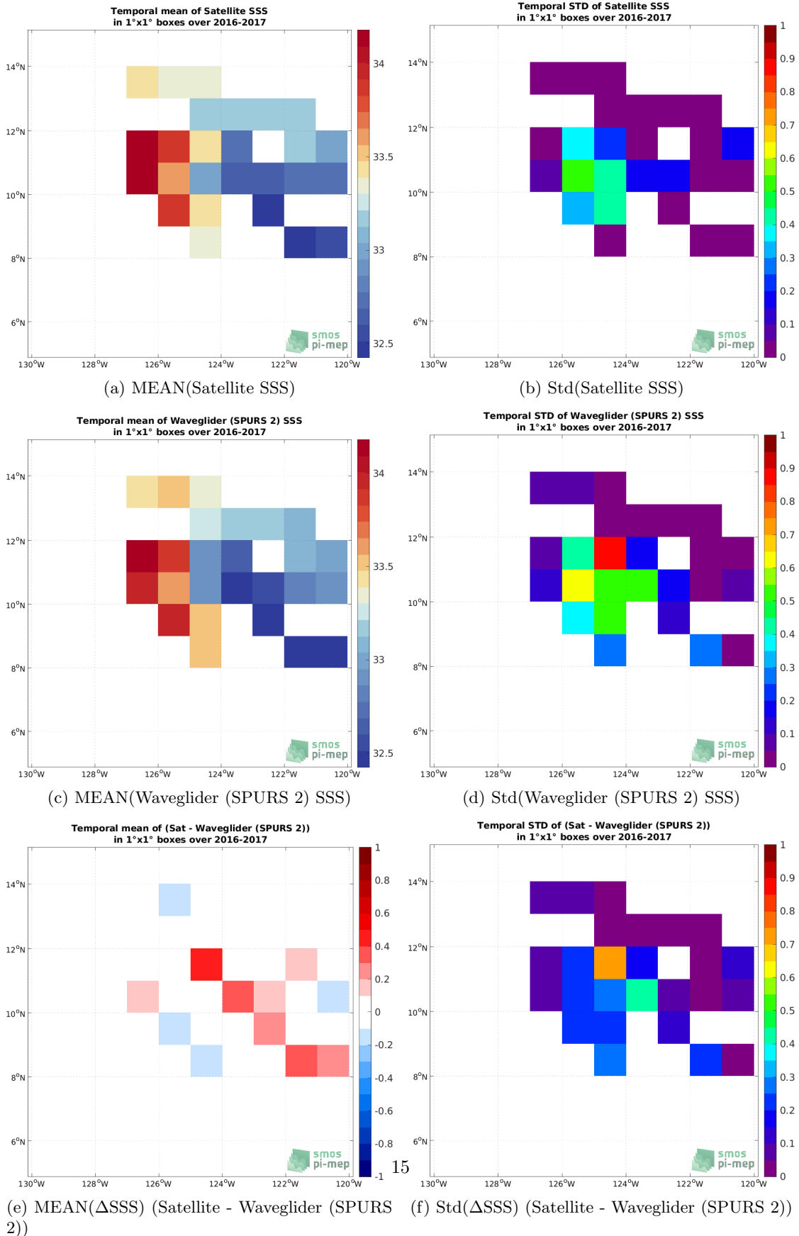
Figure 5: Temporal mean (left) and Std (right) of SSS from SMOS SSS L4 v1 - Monthly (CMEMS-CNR) (top), Waveglider (SPURS 2) (middle), and of \Delta SSS (Satellite - Waveglider (SPURS 2)). Only match-up pairs are used to generate these maps.
