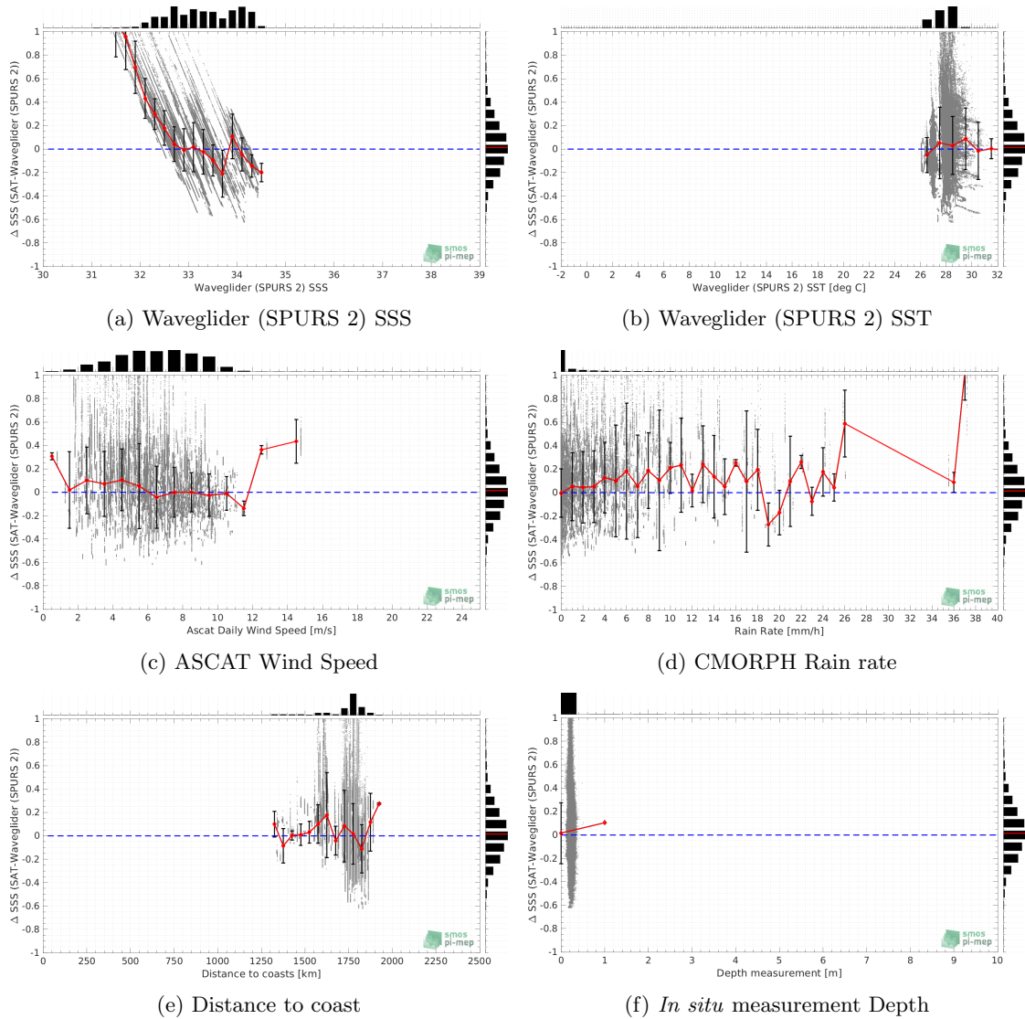
Figure 10: \Delta SSS (Satellite - Waveglider (SPURS 2)) sorted as function of Waveglider (SPURS 2) SSS values a), Waveglider (SPURS 2) SST b), ASCAT Wind speed c), CMORPH rain rate d), distance to coast (e) and in situ measurement depth (f). In all plots the median and Std of \Delta SSS for each bin is indicated by the red curves and black vertical thick bars ( \pm 1 Std)
