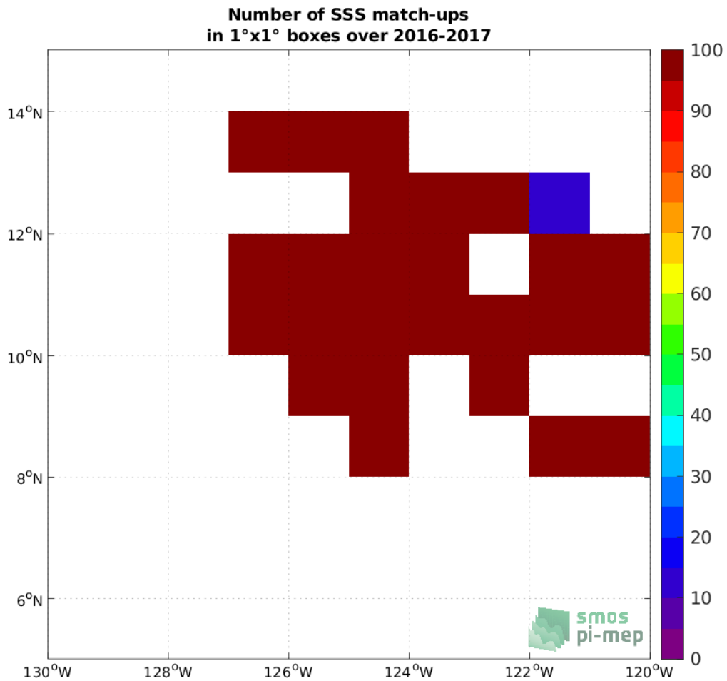
Figure 3: Number of SSS match-ups between Waveglider SSS and the SMOS SSS L4 v1 - Monthly (CMEMS-CNR) SSS product for the SPURS 2 Pi-MEP region over 1°×1° boxes and for the full satellite product period.
