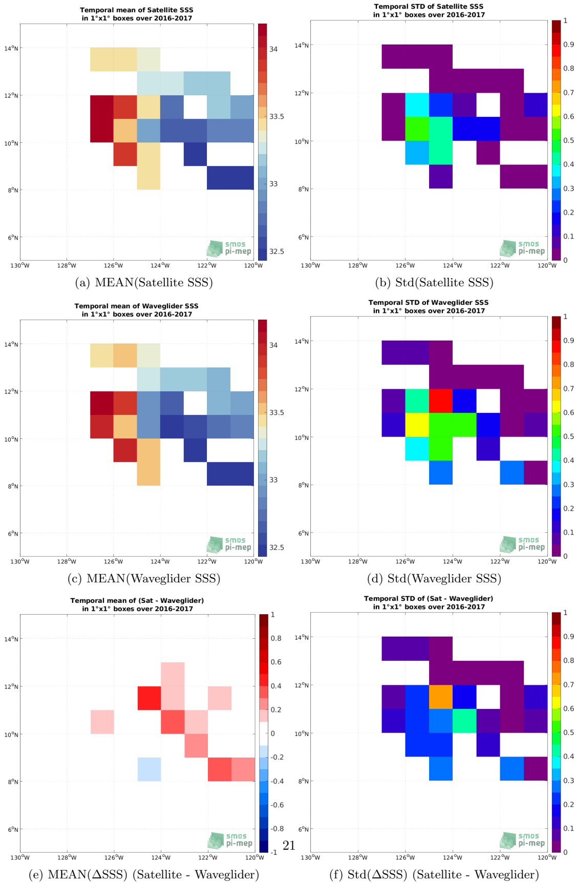
Figure 5: Temporal mean (left) and Std (right) of SSS from SMOS SSS L4 v1 - Monthly (CMEMS-CNR) (top), Waveglider (middle), and of \Delta SSS (Satellite - Waveglider). Only match-pairs are used to generate these maps.
