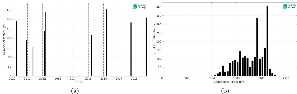
Figure 2: Number of match-ups between TSG (SAMOS) and SMOS SSS L4 v1 - Monthly (CMEMS-CNR) SSS as a function of time (a) and as function of the distance to coast (b) over the SPURS 2 Pi-MEP region and for the full satellite product period.
