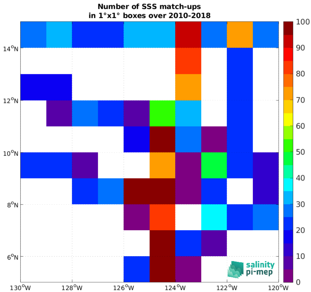
Figure 5: Number of SSS match-ups between TSG (SAMOS) SSS and the SMOS SSS L4 v1 - Monthly (CMEMS-CNR) SSS product for the SPURS 2 Pi-MEP region over 1°x1° boxes and for the full satellite product period.
