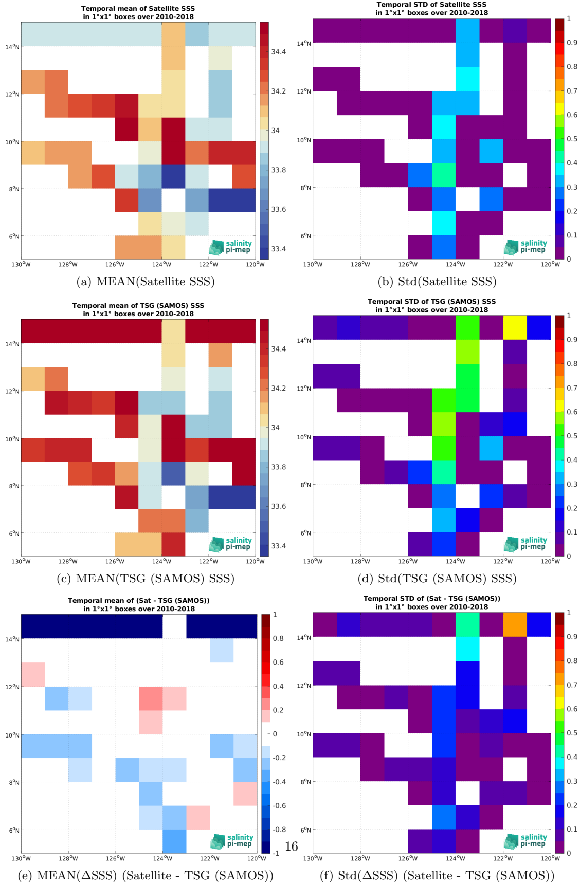
Figure 7: Temporal mean (left) and Std (right) of SSS from SMOS SSS L4 v1 - Monthly (CMEMS-CNR) (top), TSG (SAMOS) (middle), and of \Delta SSS (Satellite - TSG (SAMOS)). Only match-up pairs are used to generate these maps.
