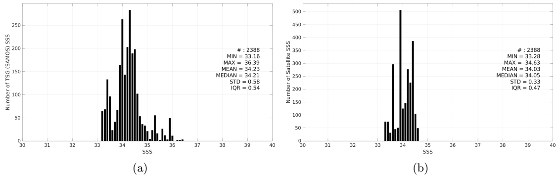
Figure 3: Histograms of SSS from TSG (SAMOS) (a) and SMOS SSS L4 v1 - Monthly (CMEMS-CNR) (b) considering all match-up pairs per bins of 0.1 over the SPURS 2 Pi-MEP region and for the full satellite product period.
