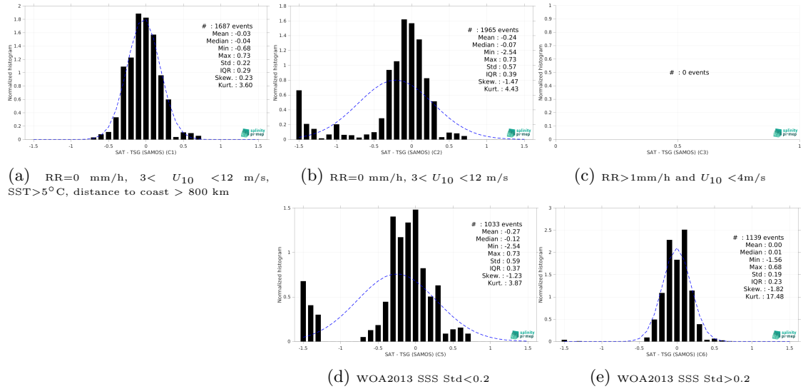
Figure 15: Normalized histogram of \Delta SSS (SMOS SSS L4 v1 - Monthly (CMEMS-CNR) - TSG (SAMOS)) for 5 different subdatasets corresponding to: RR=0 mm/h, 3 < U_{10} < 12 m/s, SST > 5°C, distance to coast > 800 km (a), RR=0 mm/h, 3 < U_{10} < 12 m/s (b), RR > 1mm/h and U_{10} < 4 m/s (c), WOA2013 SSS Std < 0.2 (d), WOA2013 SSS Std > 0.2 (e).
