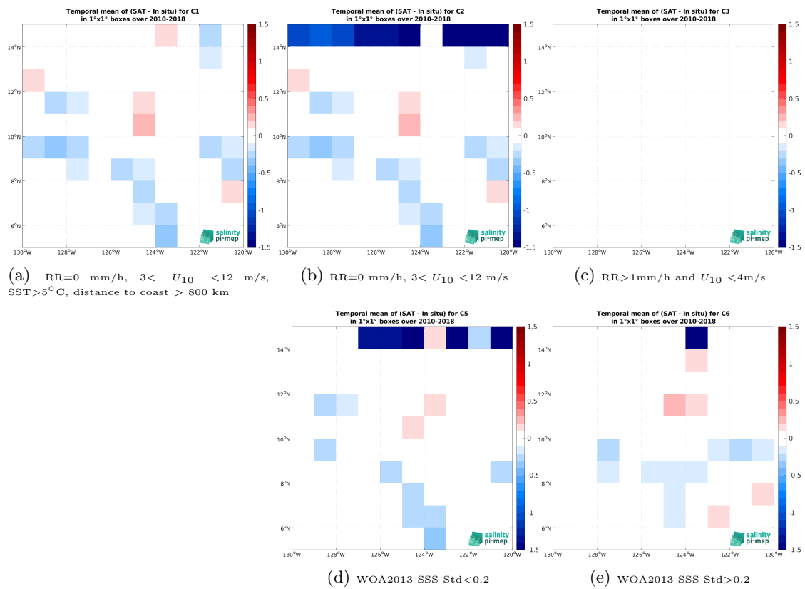
Figure 14: Temporal mean gridded over spatial boxes of size 1^\circ \times 1^\circ of \Delta SSS (SMOS SSS L4 v1 - Monthly (CMEMS-CNR) - TSG (SAMOS)) for 5 different subdatasets corresponding to:RR=0 mm/h, 3 < U_{10} < 12 m/s, SST >5^\circ\text{C} , distance to coast > 800 km (a), RR=0 mm/h, 3 < U_{10} < 12 m/s (b), RR >1 mm/h and U_{10} < 4 m/s (c), WOA2013 SSS Std <0.2 (d), WOA2013 SSS Std >0.2 (e).
