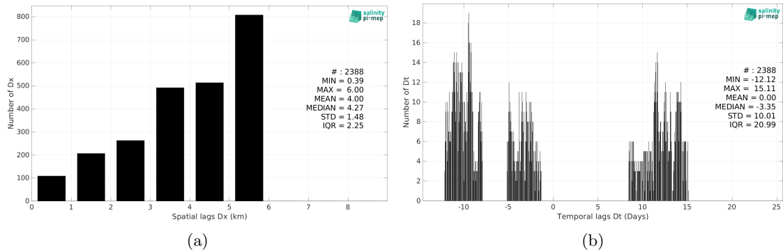
Figure 6: Histograms of the spatial (a) and temporal (b) lags between the location/time of the TSG (SAMOS) measurement and the date of the corresponding SMOS SSS L4 v1 - Monthly (CMEMS-CNR) SSS pixel.
