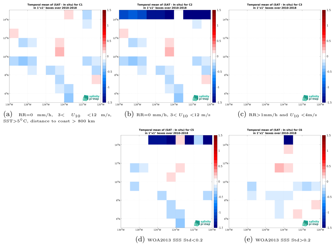
Figure 14: Temporal mean gridded over spatial boxes of size 1^\circ \times 1^\circ of \Delta\text{SSS} (SMOS SSS L4 v1 - Monthly (CMEMS-CNR) - TSG (SAMOS)) for 5 different subdatasets corresponding to:RR=0 mm/h, 3 < U_{10} < 12 m/s, SST > 5°C, distance to coast > 800 km (a), RR=0 mm/h, 3 < U_{10} < 12 m/s (b), RR > 1mm/h and U_{10} < 4 m/s (c), WOA2013 SSS Std < 0.2 (d), WOA2013 SSS Std > 0.2 (e).
