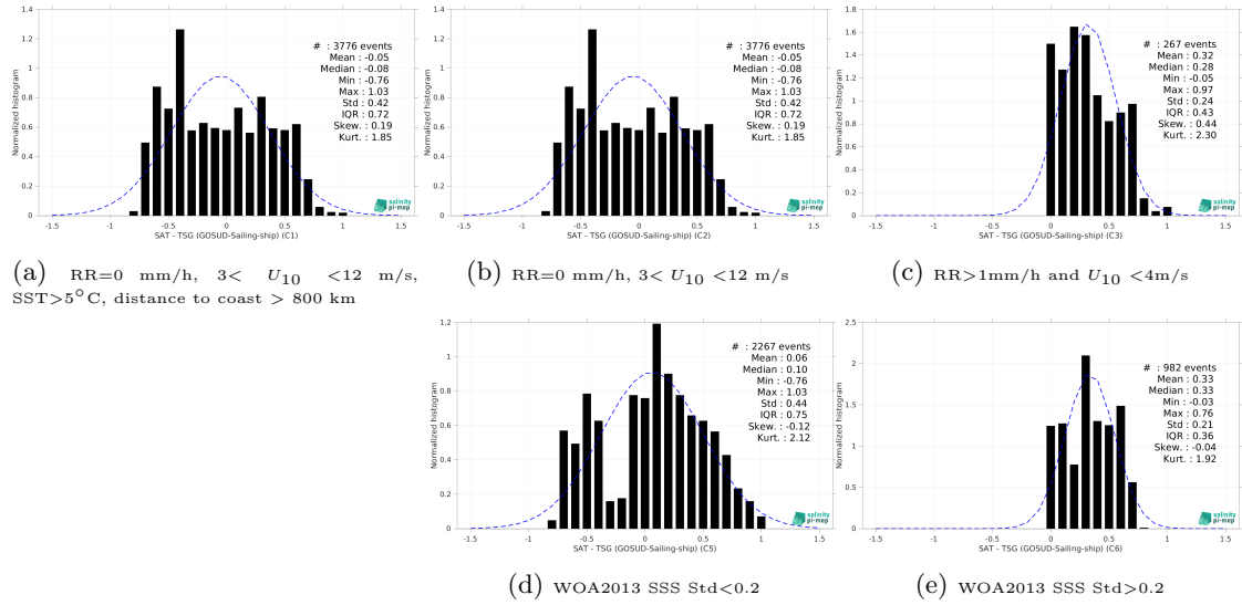
Figure 15: Normalized histogram of \Delta SSS (SMOS SSS L4 v1 - Monthly (CMEMS-CNR) - TSG (GOSUD-Sailing-ship)) for 5 different subdatasets corresponding to: RR=0 mm/h, 3 < U_{10} < 12 m/s, SST >5^{\circ} C, distance to coast > 800 km (a), RR=0 mm/h, 3 < U_{10} < 12 m/s (b), RR >1 mm/h and U_{10} < 4 m/s (c), WOA2013 SSS Std <0.2 (d), WOA2013 SSS Std >0.2 (e).
