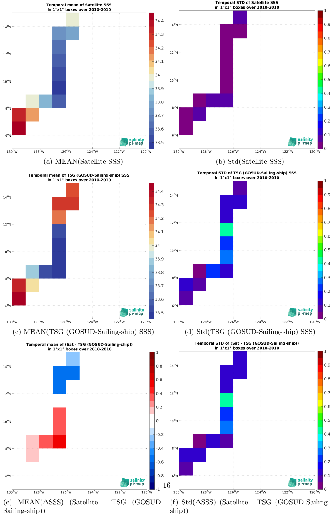
Figure 7: Temporal mean (left) and Std (right) of SSS from SMOS SSS L4 v1 - Monthly (CMEMS-CNR) (top), TSG (GOSUD-Sailing-ship) (middle), and of \Delta SSS (Satellite - TSG (GOSUD-Sailing-ship)). Only match-up pairs are used to generate these maps.
