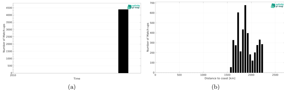
Figure 2: Number of match-ups between TSG (GOSUD-Sailing-ship) and SMOS SSS L4 v1 - Monthly (CMEMS-CNR) SSS as a function of time (a) and as function of the distance to coast (b) over the SPURS 2 Pi-MEP region and for the full satellite product period.
