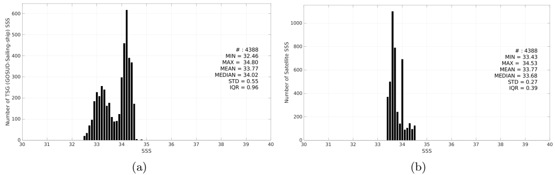
Figure 3: Histograms of SSS from TSG (GOSUD-Sailing-ship) (a) and SMOS SSS L4 v1 - Monthly (CMEMS-CNR) (b) considering all match-up pairs per bins of 0.1 over the SPURS 2 Pi-MEP region and for the full satellite product period.
