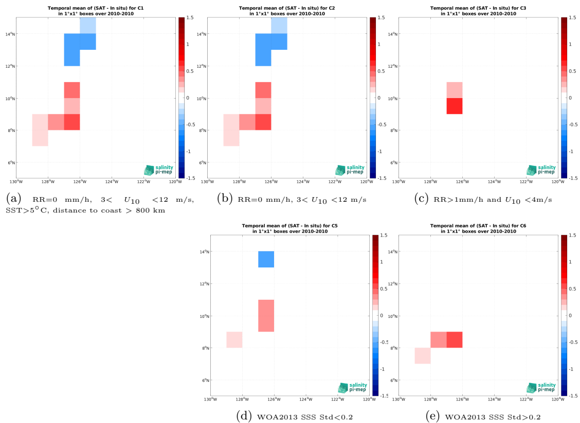
Figure 14: Temporal mean gridded over spatial boxes of size 1^\circ \times 1^\circ of \Delta\text{SSS} (SMOS SSS L4 v1 - Monthly (CMEMS-CNR) - TSG (GOSUD-Sailing-ship)) for 5 different subdatasets corresponding to:RR=0 mm/h, 3 < U_{10} < 12 m/s, SST >5^\circ\text{C} , distance to coast > 800 km (a), RR=0 mm/h, 3 < U_{10} < 12 m/s (b), RR >1 mm/h and U_{10} < 4 m/s (c), WOA2013 SSS Std <0.2 (d), WOA2013 SSS Std >0.2 (e).
