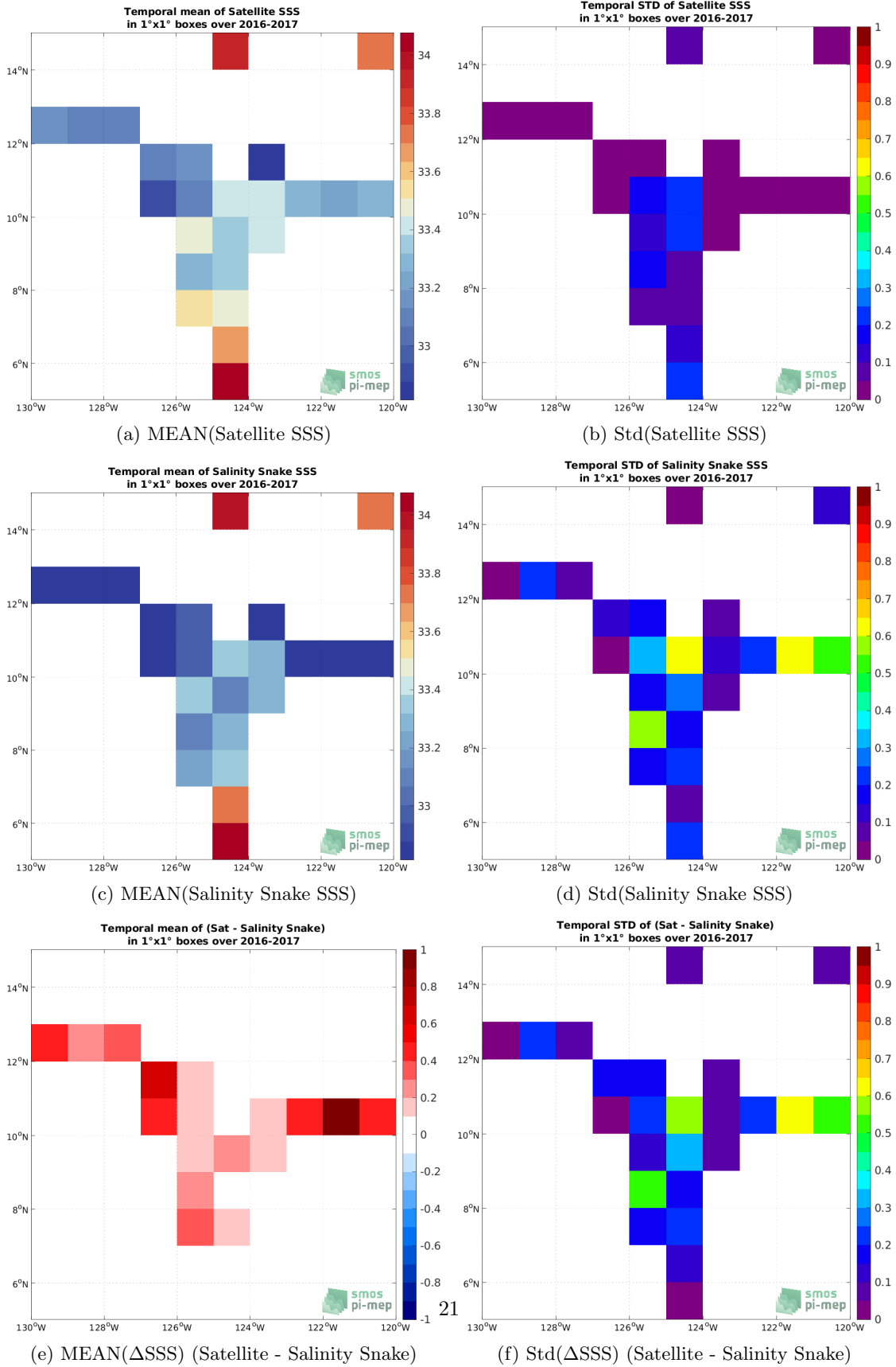
Figure 5: Temporal mean (left) and Std (right) of SSS from SMOS SSS L4 v1 - Monthly (CMEMS-CNR) (top), Salinity Snake (middle), and of \Delta SSS (Satellite - Salinity Snake). Only match-up pairs are used to generate these maps.
