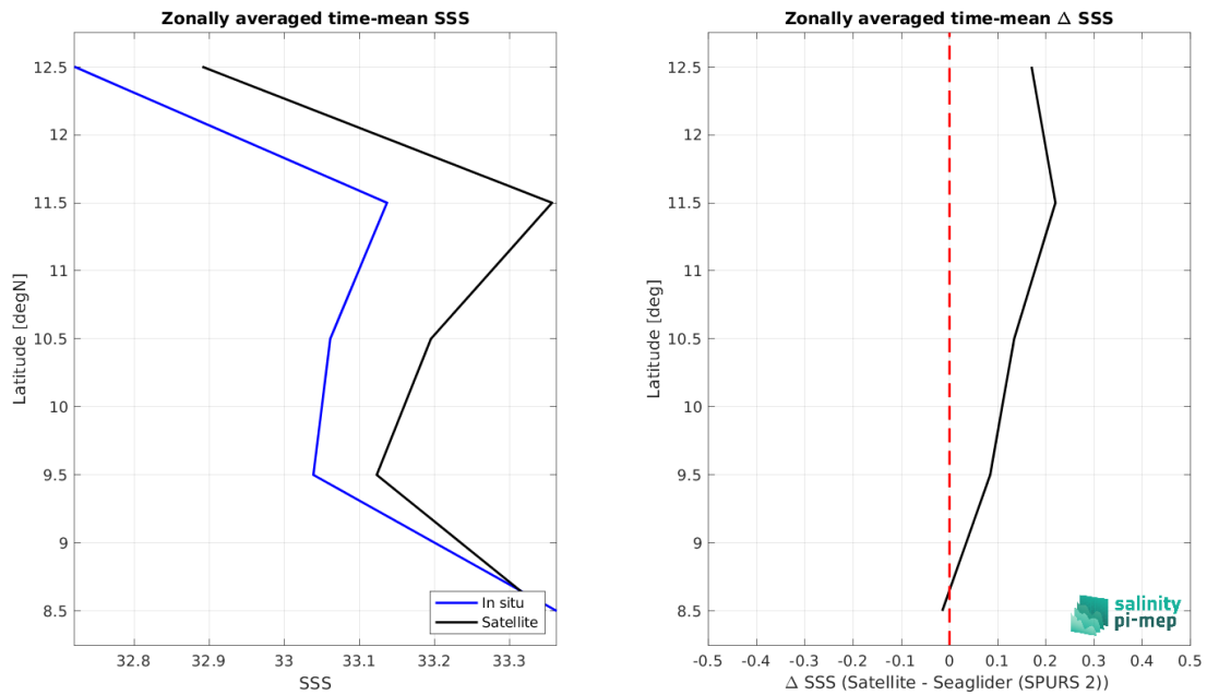
Figure 8: Left panel: Zonal mean SSS from SMOS SSS L4 v1 - Monthly (CMEMS-CNR) satellite product (black) and from Seaglider (SPURS 2) (blue). Right panel: Zonal mean of \Delta SSS (Satellite - Seaglider (SPURS 2)) for all the collected Pi-MEP match-up pairs estimated over the full satellite product period.
