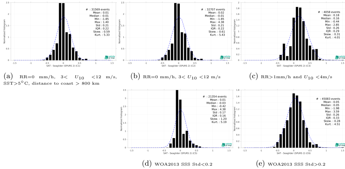
Figure 13: Normalized histogram of \Delta SSS (SMOS SSS L4 v1 - Monthly (CMEMS-CNR) - Seaglider (SPURS 2)) for 5 different subdatasets corresponding to: RR=0 mm/h, 3 < U_{10} < 12 m/s, SST>5°C, distance to coast > 800 km (a), RR=0 mm/h, 3 < U_{10} < 12 m/s (b), RR>1mm/h and U_{10} < 4 m/s (c), WOA2013 SSS Std<0.2 (d), WOA2013 SSS Std>0.2 (e).
