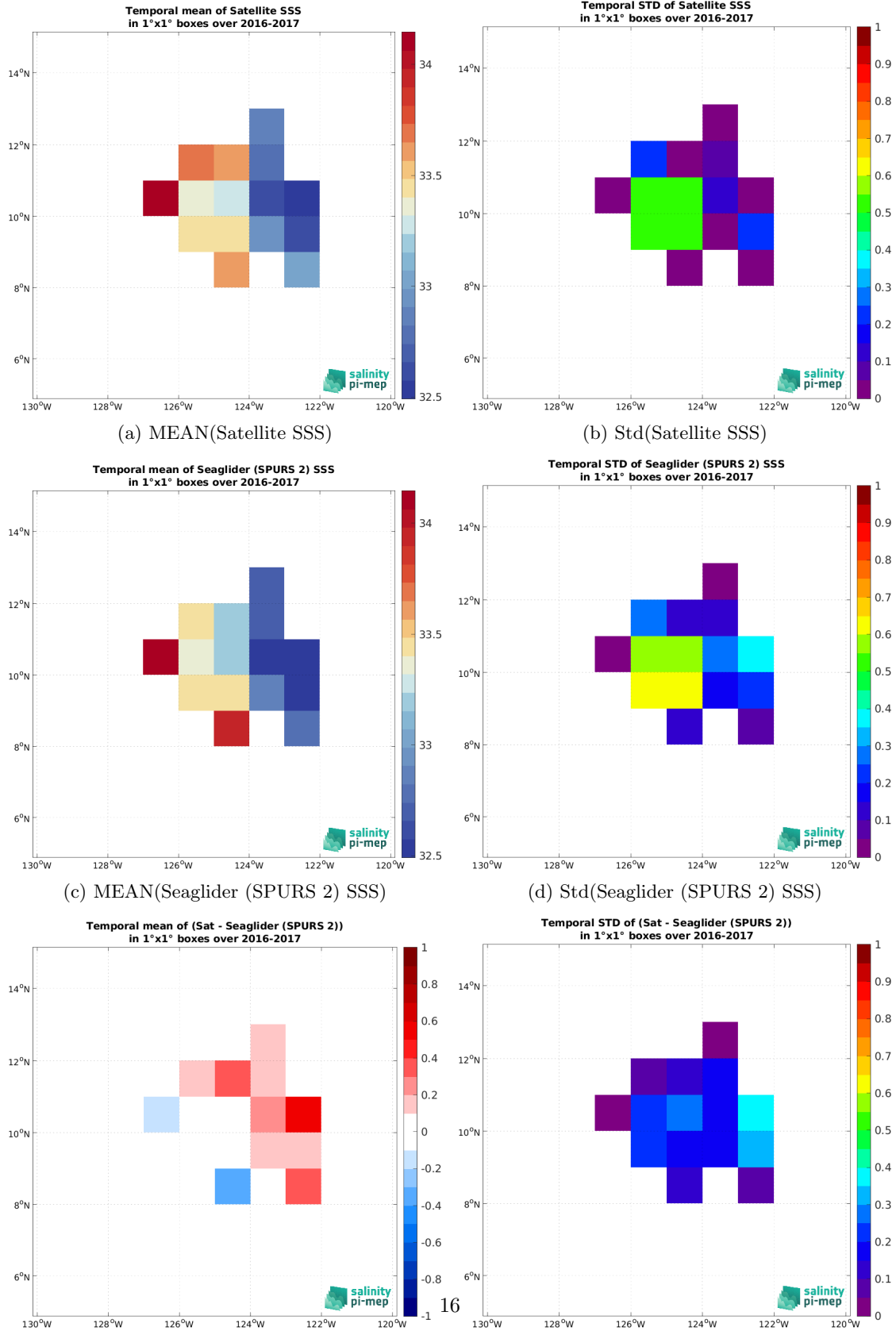
Figure 6: Temporal mean (left) and Std (right) of SSS from SMOS SSS L4 v1 - Monthly (CMEMS-CNR) (top), Seaglider (SPURS 2) (middle), and of \Delta SSS (Satellite - Seaglider (SPURS 2)). Only match-up pairs are used to generate these maps.
