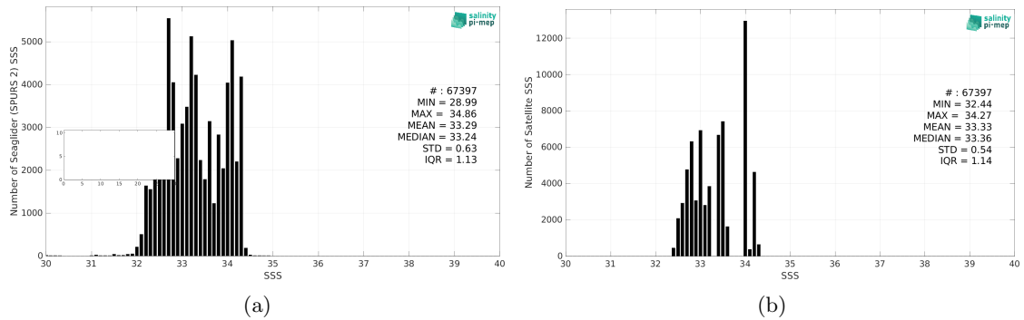
Figure 2: Histograms of SSS from Seaglider (SPURS 2) (a) and SMOS SSS L4 v1 - Monthly (CMEMS-CNR) (b) considering all match-up pairs per bins of 0.1 over the SPURS 2 Pi-MEP region and for the full satellite product period.
