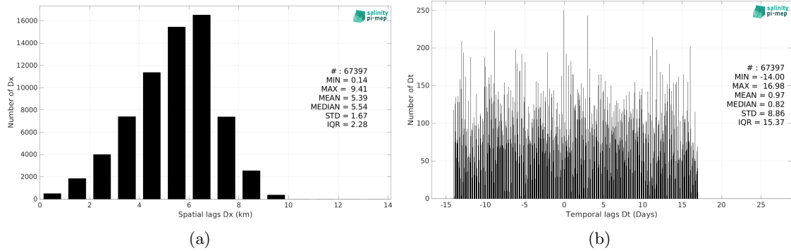
Figure 5: Histograms of the spatial (a) and temporal (b) lags between the location/time of the Seaglider (SPURS 2) measurement and the date of the corresponding SMOS SSS L4 v1 - Monthly (CMEMS-CNR) SSS pixel.
