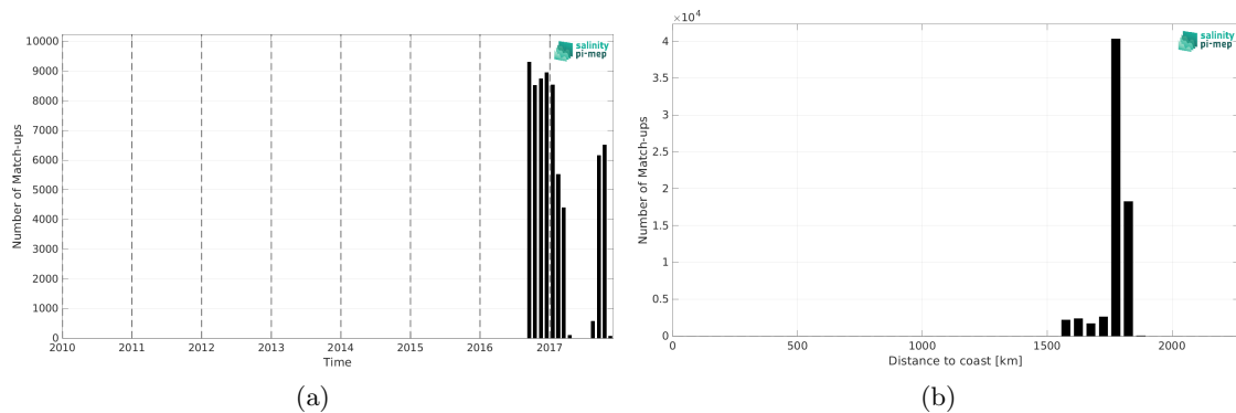
Figure 1: Number of match-ups between Seaglider (SPURS 2) and SMOS SSS L4 v1 - Monthly (CMEMS-CNR) SSS as a function of time (a) and as function of the distance to coast (b) over the SPURS 2 Pi-MEP region and for the full satellite product period.
