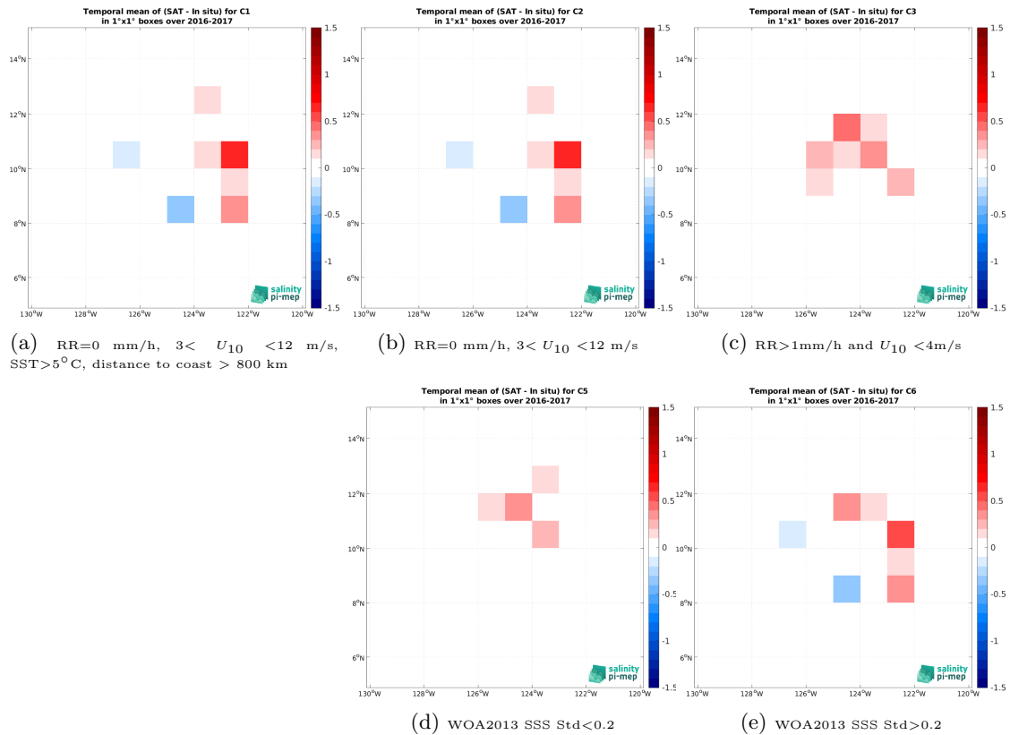
Figure 12: Temporal mean gridded over spatial boxes of size 1^\circ \times 1^\circ of \Delta SSS (SMOS SSS L4 v1 - Monthly (CMEMS-CNR) - Seagliger (SPURS 2)) for 5 different subdatasets corresponding to:RR=0 mm/h, 3 < U_{10} < 12 m/s, SST >5^\circ\text{C} , distance to coast > 800 km (a), RR=0 mm/h, 3 < U_{10} < 12 m/s (b), RR >1 mm/h and U_{10} < 4 m/s (c), WOA2013 SSS Std <0.2 (d), WOA2013 SSS Std >0.2 (e).
