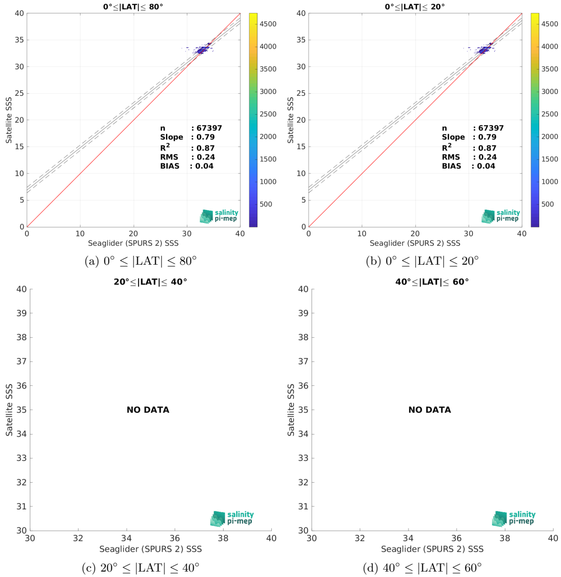
Figure 9: Contour maps of the concentration of SMOS SSS L4 v1 - Monthly (CMEMS-CNR) SSS (y-axis) versus Seaglider (SPURS 2) SSS (x-axis) at match-up pairs for different latitude bands. For each plot, the red line shows x=y . The black thin and dashed lines indicate a linear fit through the data cloud and the \pm 95\% confidence levels, respectively. The number match-up pairs n , the slope and R^2 coefficient of the linear fit, the root mean square (RMS) and the mean bias between satellite and in situ data are indicated for each latitude band in each plots.
