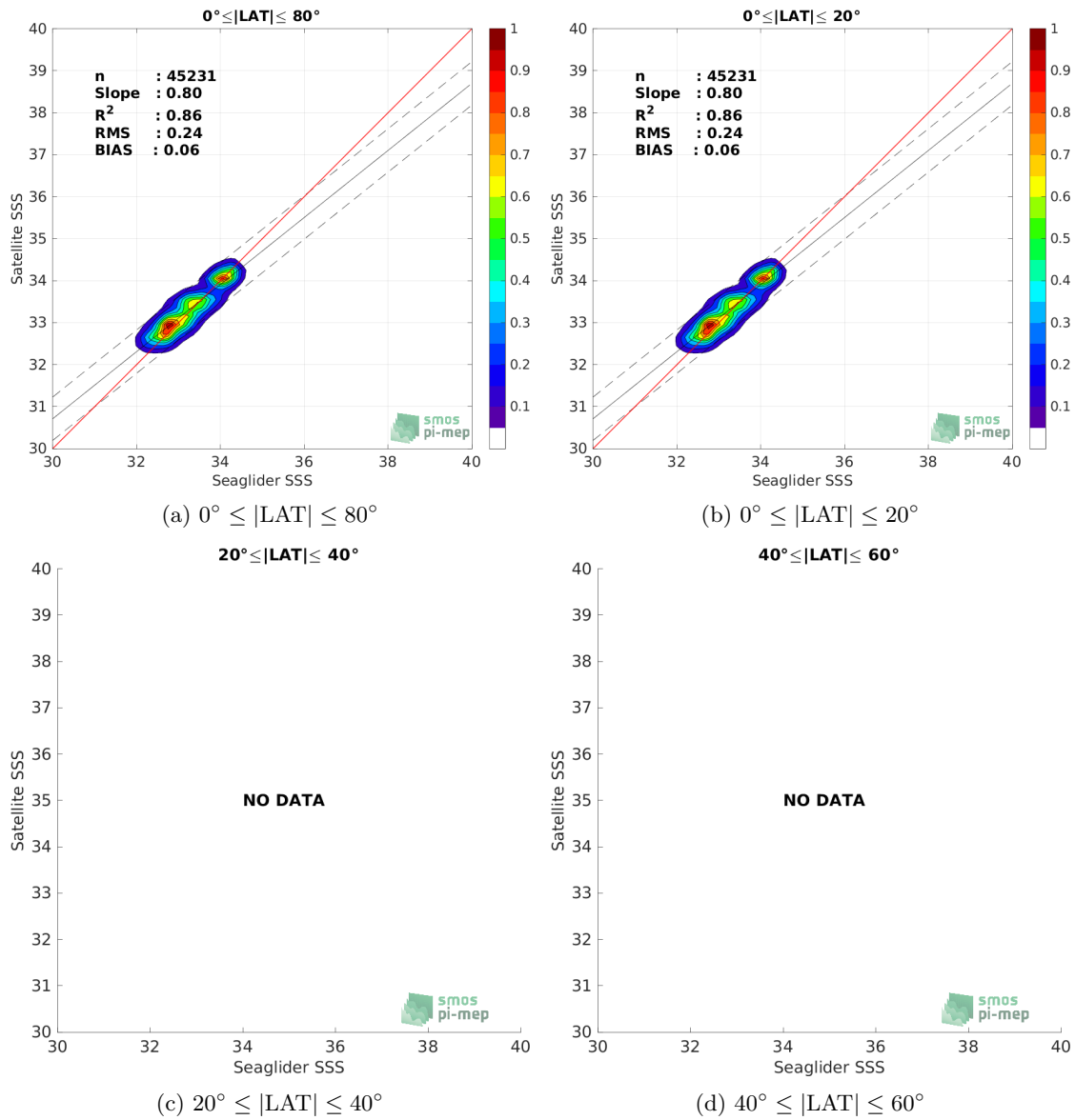
Figure 8: Contour maps of the concentration of SMOS SSS L4 v1 - Monthly (CMEMS-CNR) SSS (y-axis) versus Seaglider SSS (x-axis) at match-up pairs for different latitude bands. For each plot, the red line shows x=y . The black thin and dashed lines indicate a linear fit through the data cloud and the \pm 95\% confidence levels, respectively. The number match-up pairs n , the slope and R^2 coefficient of the linear fit, the root mean square (RMS) and the mean bias between satellite and in situ data are indicated for each latitude band in each plots.
