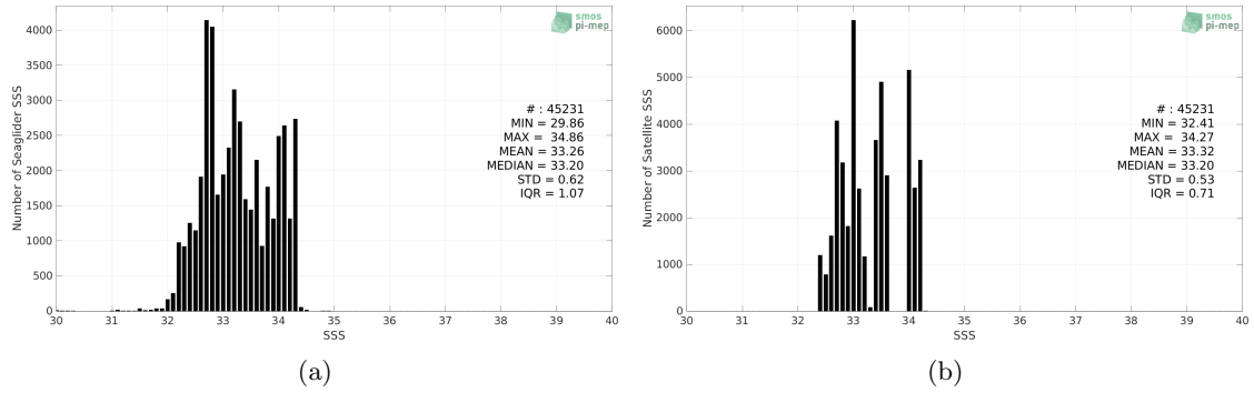
Figure 2: Histograms of SSS from Seaglider (a) and SMOS SSS L4 v1 - Monthly (CMEMS-CNR) (b) considering all match-up pairs per bins of 0.1 over the SPURS 2 Pi-MEP region and for the full satellite product period.
