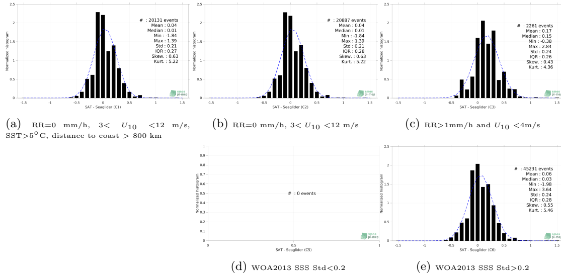
Figure 12: Normalized histogram of \Delta SSS (SMOS SSS L4 v1 - Monthly (CMEMS-CNR) - Seaglider) for 5 different subdatasets corresponding to: RR=0 mm/h, 3 < U_{10} < 12 m/s, SST > 5°C, distance to coast > 800 km (a), RR=0 mm/h, 3 < U_{10} < 12 m/s (b), RR > 1mm/h and U_{10} < 4 m/s (c), WOA2013 SSS Std < 0.2 (d), WOA2013 SSS Std > 0.2 (e).
