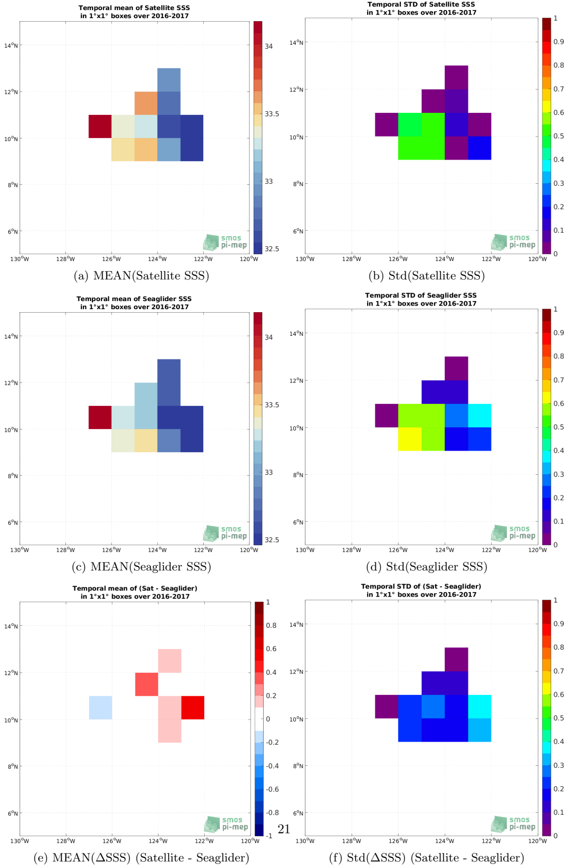
Figure 5: Temporal mean (left) and Std (right) of SSS from SMOS SSS L4 v1 - Monthly (CMEMS-CNR) (top), Seaglider (middle), and of \Delta SSS (Satellite - Seaglider). Only match-pairs are used to generate these maps.
