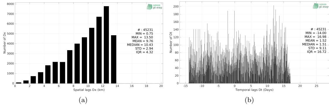
Figure 4: Histograms of the spatial (a) and temporal (b) lags between the location/time of the Seaglider measurement and the date of the corresponding SMOS SSS L4 v1 - Monthly (CMEMS-CNR) SSS pixel.
