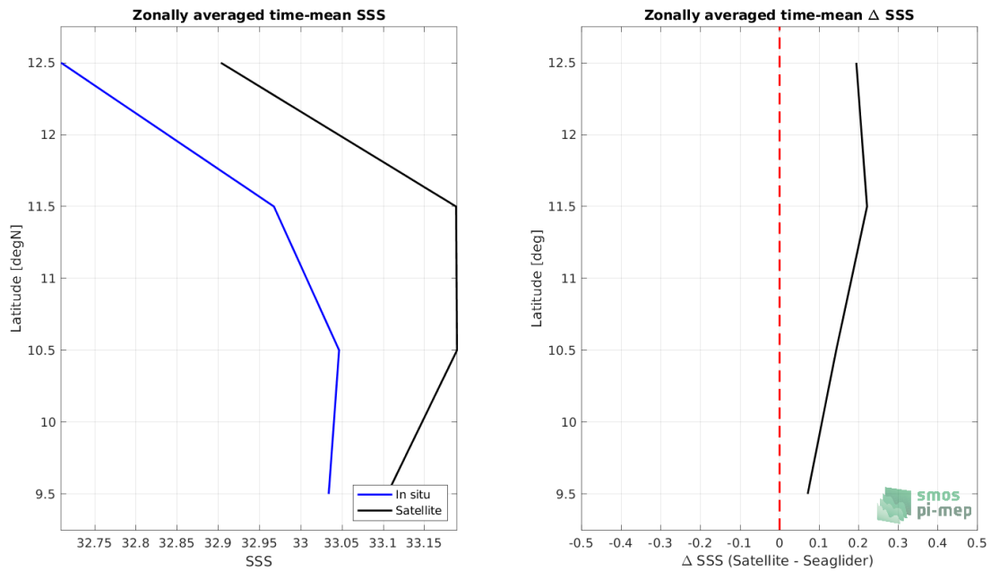
Figure 7: Left panel: Zonal mean SSS from SMOS SSS L4 v1 - Monthly (CMEMS-CNR) satellite product (black) and from Seaglider (blue). Right panel: Zonal mean of \Delta SSS (Satellite - Seaglider) for all the collected Pi-MEP match-up pairs estimated over the full satellite product period.
