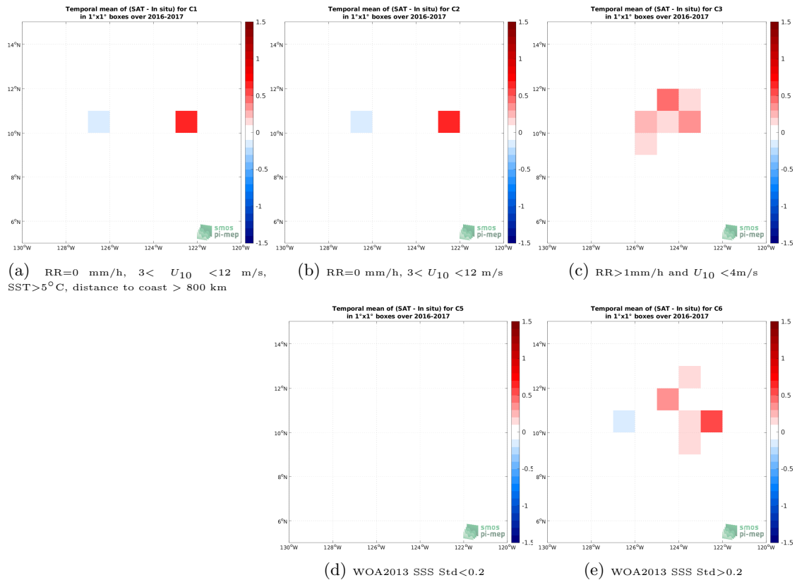
Figure 11: Temporal mean gridded over spatial boxes of size 1^\circ \times 1^\circ of \Delta SSS (SMOS SSS L4 v1 - Monthly (CMEMS-CNR) - Seaglider) for 5 different subdatasets corresponding to:RR=0 mm/h, 3 < U_{10} < 12 m/s, SST >5^\circ C, distance to coast > 800 km (a), RR=0 mm/h, 3 < U_{10} < 12 m/s (b), RR >1 mm/h and U_{10} < 4 m/s (c), WOA2013 SSS Std <0.2 (d), WOA2013 SSS Std >0.2 (e).
