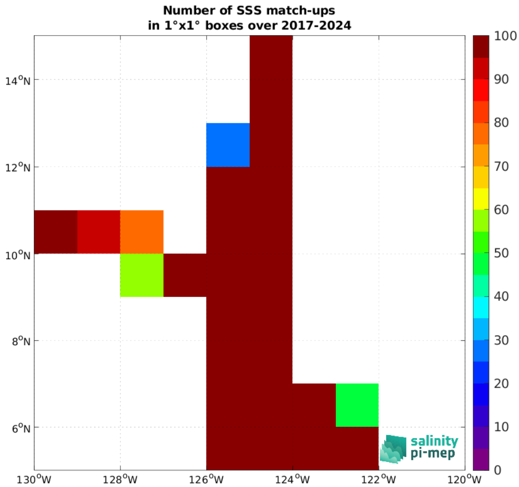
Figure 5: Number of SSS match-ups between Saildrone SSS and the SMOS SSS L4 v1 - Monthly (CMEMS-CNR) SSS product for the SPURS 2 Pi-MEP region over 1°x1° boxes and for the full satellite product period.
