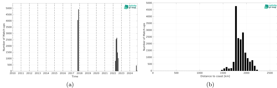
Figure 2: Number of match-ups between Saildrone and SMOS SSS L4 v1 - Monthly (CMEMS-CNR) SSS as a function of time (a) and as function of the distance to coast (b) over the SPURS 2 Pi-MEP region and for the full satellite product period.
