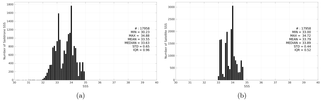
Figure 3: Histograms of SSS from Saildrone (a) and SMOS SSS L4 v1 - Monthly (CMEMS-CNR) (b) considering all match-up pairs per bins of 0.1 over the SPURS 2 Pi-MEP region and for the full satellite product period.
