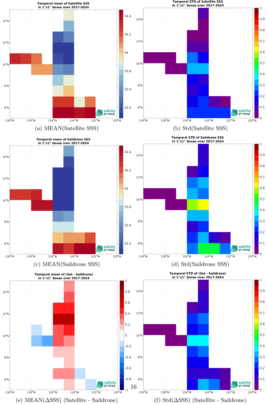
Figure 7: Temporal mean (left) and Std (right) of SSS from SMOS SSS L4 v1 - Monthly (CMEMS-CNR) (top), Saildrone (middle), and of \Delta SSS (Satellite - Saildrone). Only match-pairs are used to generate these maps.
