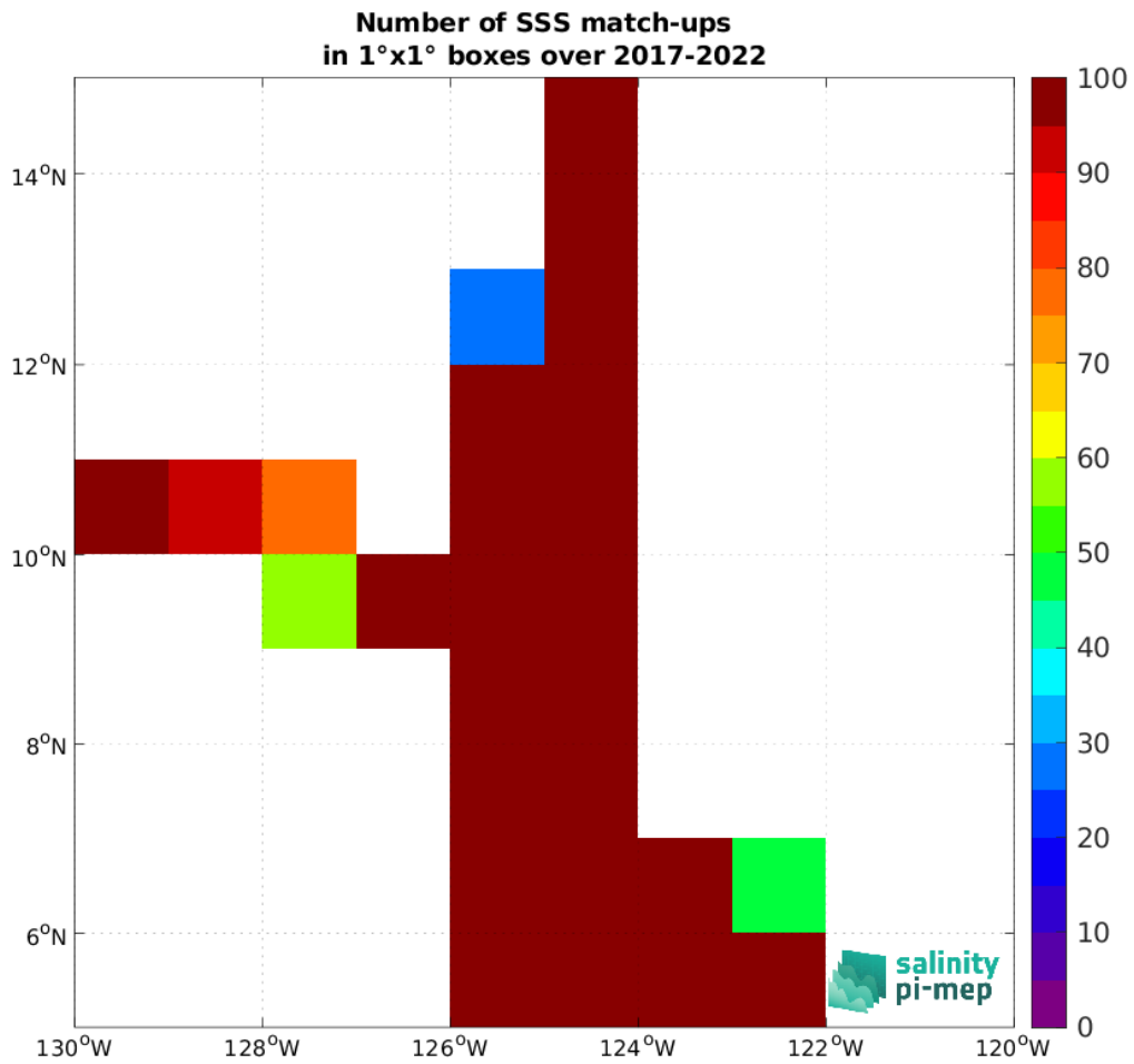
Figure 5: Number of SSS match-ups between Sairdrone SSS and the SMOS SSS L4 v1 - Monthly (CMEMS-CNR) SSS product for the SPURS 2 Pi-MEP region over 1°x1° boxes and for the full satellite product period.
