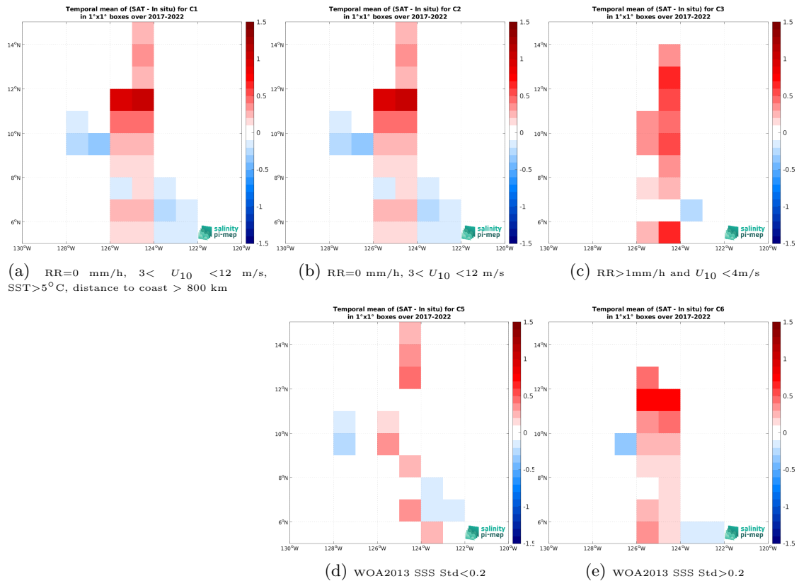
Figure 12: Temporal mean gridded over spatial boxes of size 1^\circ \times 1^\circ of \Delta SSS (SMOS SSS L4 v1 - Monthly (CMEMS-CNR) - Saildrone) for 5 different subdatasets corresponding to:RR=0 mm/h, 3 < U_{10} < 12 m/s, SST >5^\circ\text{C} , distance to coast > 800 km (a), RR=0 mm/h, 3 < U_{10} < 12 m/s (b), RR >1 mm/h and U_{10} < 4 m/s (c), WOA2013 SSS Std <0.2 (d), WOA2013 SSS Std >0.2 (e).
