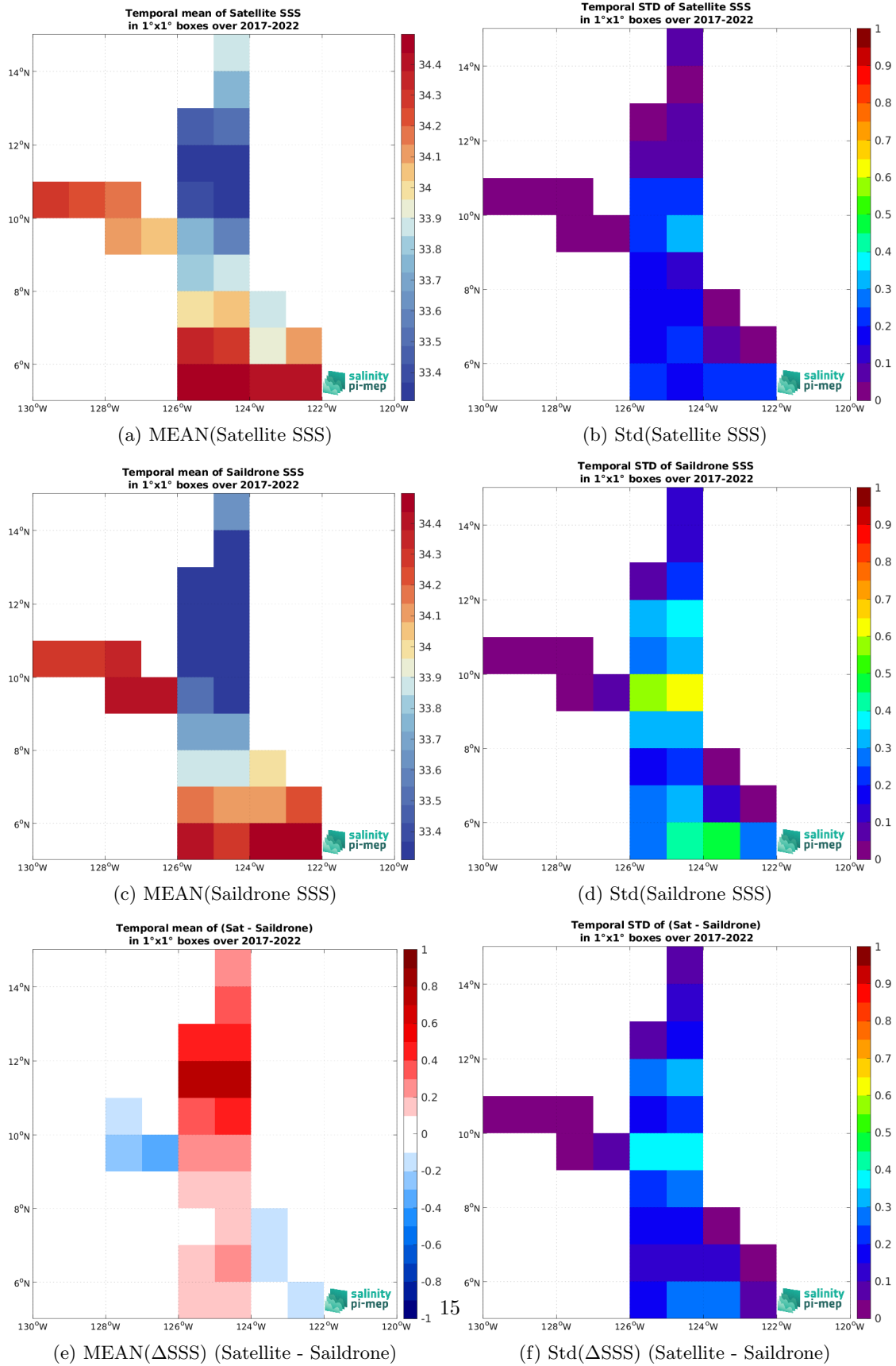
Figure 6: Temporal mean (left) and Std (right) of SSS from SMOS SSS L4 v1 - Monthly (CMEMS-CNR) (top), Saildrone (middle), and of \Delta SSS (Satellite - Saildrone). Only match-pairs are used to generate these maps.
