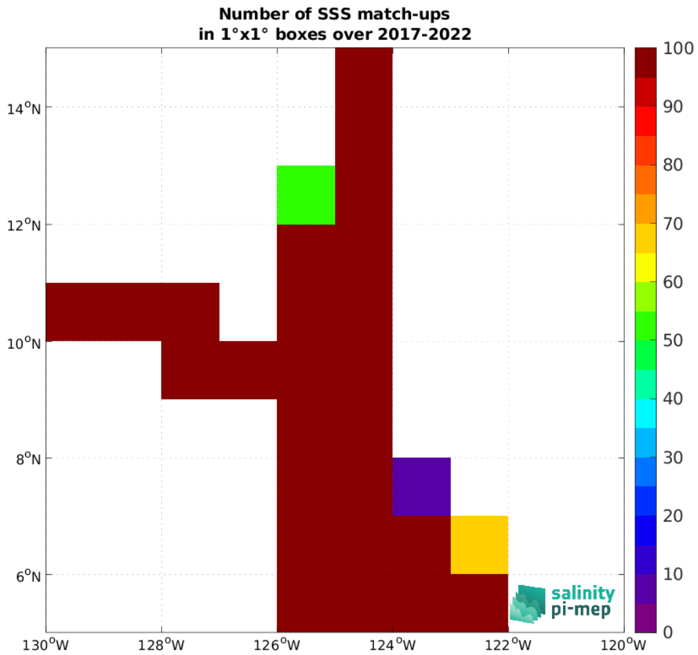
Figure 4: Number of SSS match-ups between Saildrone SSS and the SMOS SSS L4 v1 - Monthly (CMEMS-CNR) SSS product for the SPURS 2 Pi-MEP region over 1^\circ \times 1^\circ boxes and for the full satellite product period.
