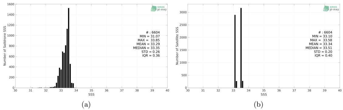
Figure 2: Histograms of SSS from Saïdrone (a) and SMOS SSS L4 v1 - Monthly (CMEMS-CNR) (b) considering all match-up pairs per bins of 0.1 over the SPURS 2 Pi-MEP region and for the full satellite product period.
