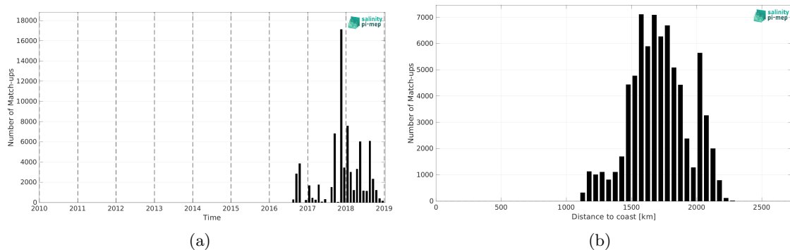
Figure 2: Number of match-ups between Surface drifters and SMOS SSS L4 v1 - Monthly (CMEMS-CNR) SSS as a function of time (a) and as function of the distance to coast (b) over the SPURS 2 Pi-MEP region and for the full satellite product period.
