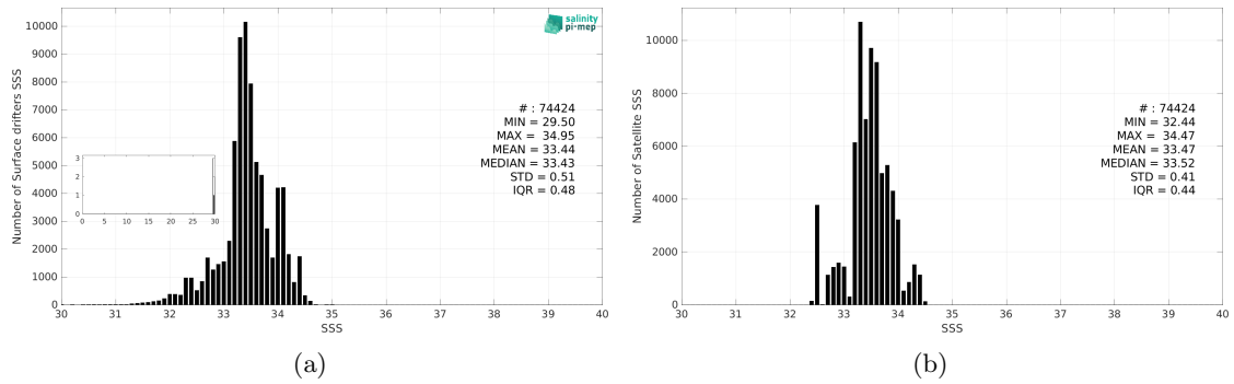
Figure 3: Histograms of SSS from Surface drifters (a) and SMOS SSS L4 v1 - Monthly (CMEMS-CNR) (b) considering all match-up pairs per bins of 0.1 over the SPURS 2 Pi-MEP region and for the full satellite product period.
