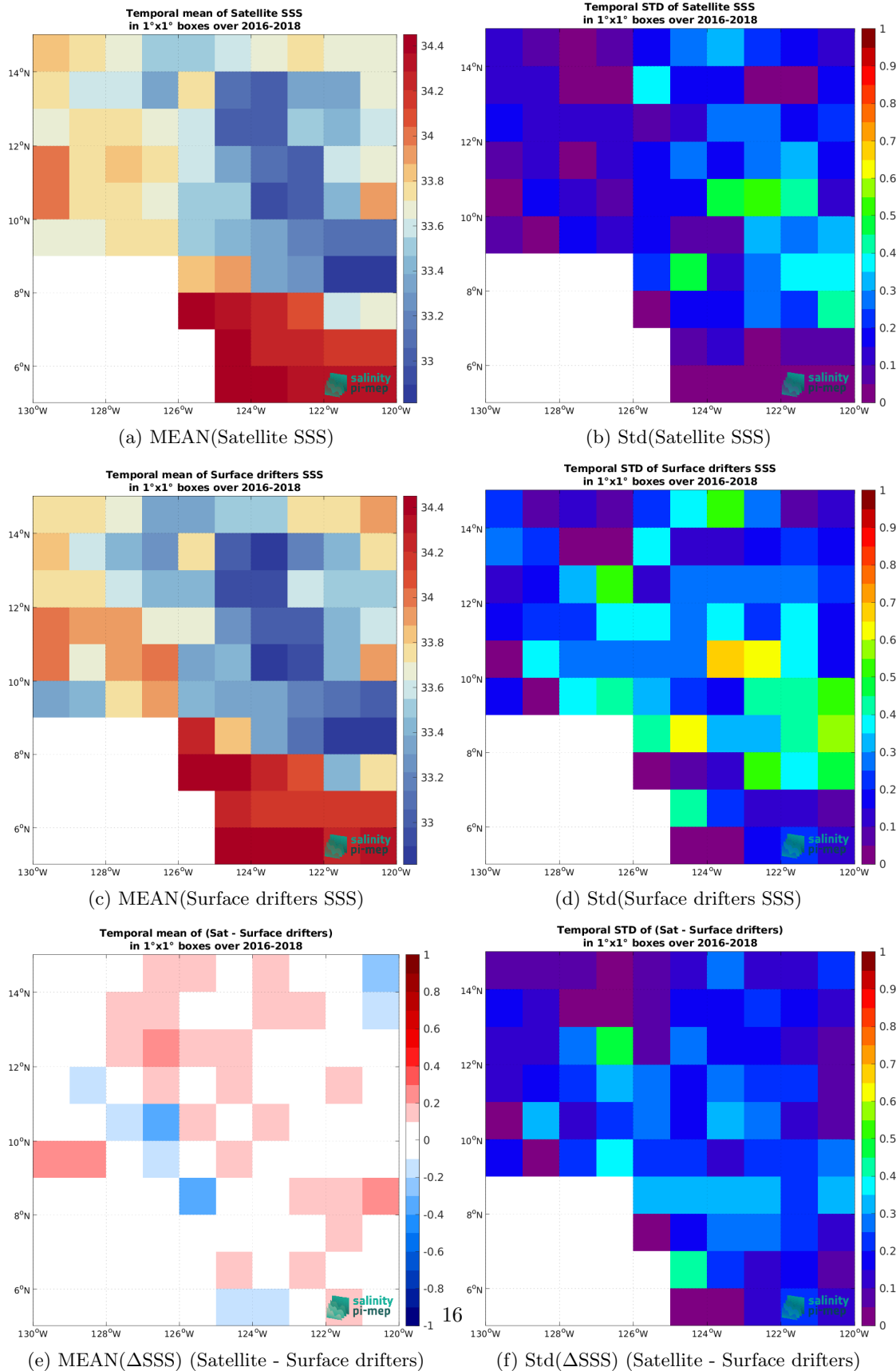
Figure 6: Temporal mean (left) and Std (right) of SSS from SMOS SSS L4 v1 - Monthly (CMEMS-CNR) (top), Surface drifters (middle), and of \Delta SSS (Satellite - Surface drifters). Only match-up pairs are used to generate these maps.
