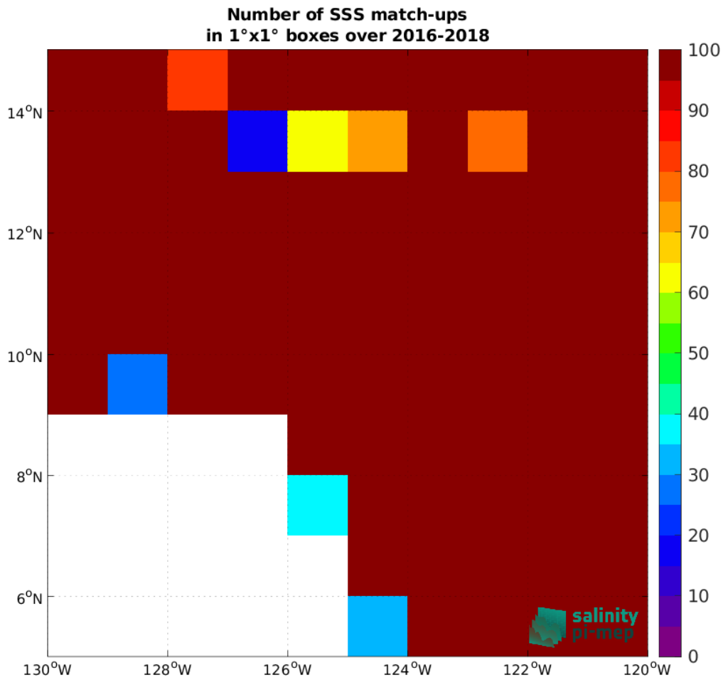
Figure 4: Number of SSS match-ups between Surface drifters SSS and the SMOS SSS L4 v1 - Monthly (CMEMS-CNR) SSS product for the SPURS 2 Pi-MEP region over 1°x1° boxes and for the full satellite product period.
