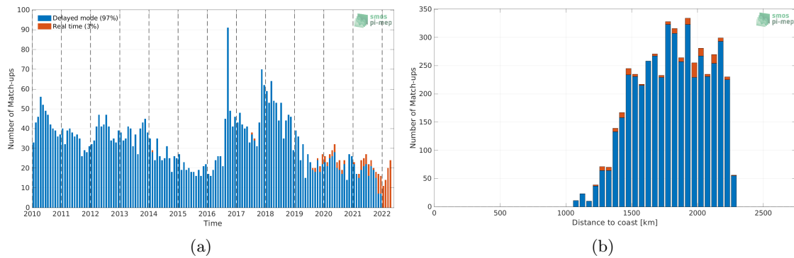
Figure 1: Number of match-ups between Argo and SMOS SSS L4 v1 - Monthly (CMEMS-CNR) SSS as a function of time (a) and as function of the distance to coast (b) over the SPURS 2 Pi-MEP region and for the full satellite product period.
