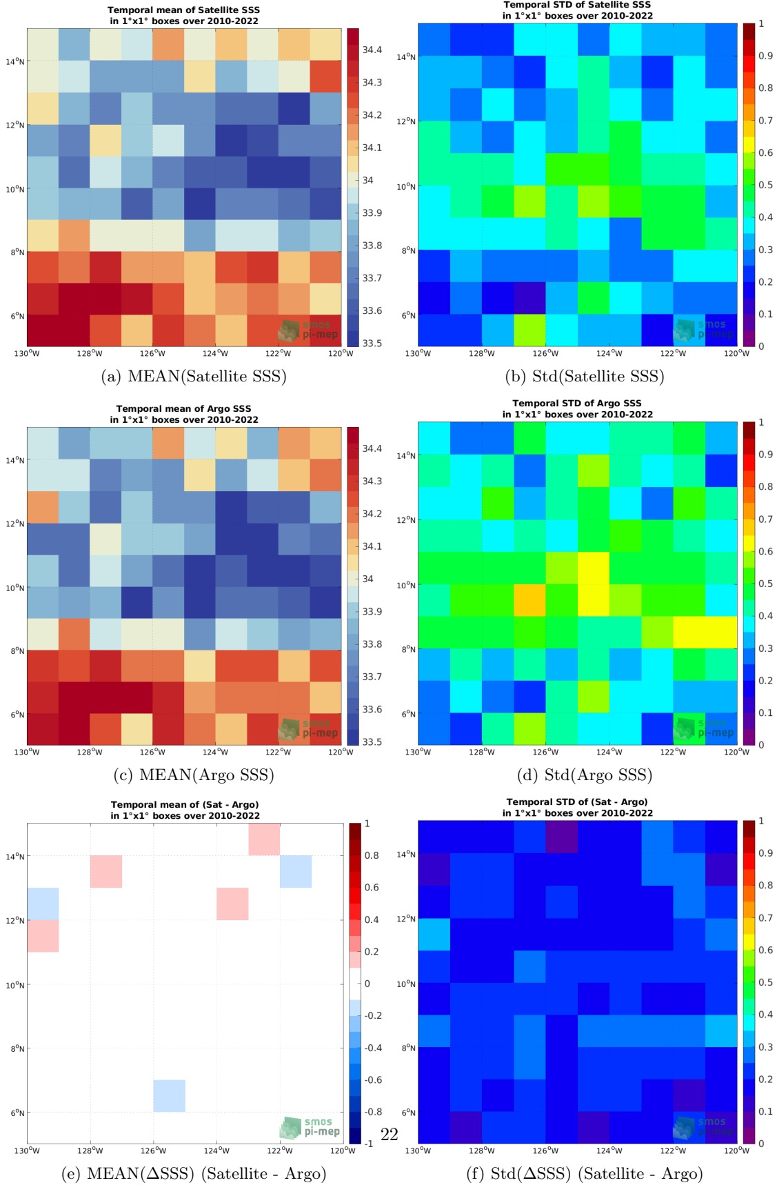
Figure 6: Temporal mean (left) and Std (right) of SSS from SMOS SSS L4 v1 - Monthly (CMEMS-CNR) (top), Argo (middle), and of \Delta SSS (Satellite - Argo). Only match-up pairs are used to generate these maps.
