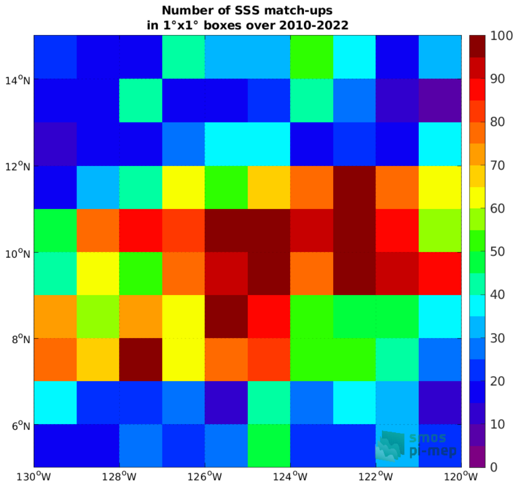
Figure 4: Number of SSS match-ups between Argo SSS and the SMOS SSS L4 v1 - Monthly (CMEMS-CNR) SSS product for the SPURS 2 Pi-MEP region over 1°x1° boxes and for the full satellite product period.
