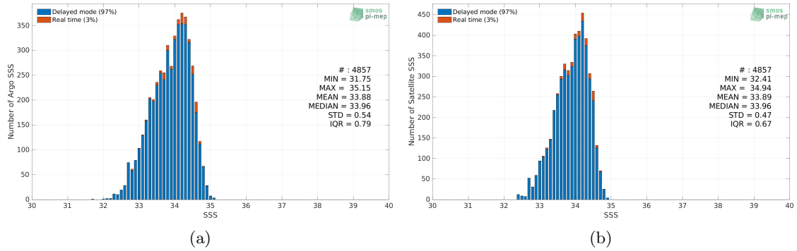
Figure 2: Histograms of SSS from Argo (a) and SMOS SSS L4 v1 - Monthly (CMEMS-CNR) (b) considering all match-up pairs per bins of 0.1 over the SPURS 2 Pi-MEP region and for the full satellite product period.
