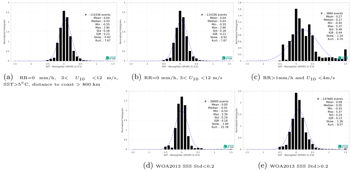
Figure 15: Normalized histogram of \Delta SSS (SMOS SSS L4 v1 - Daily (CMEMS-CNR) - Waveglider (SPURS 2)) for 5 different subdatasets corresponding to: RR=0 mm/h, 3 < U_{10} < 12 m/s, SST>5°C, distance to coast > 800 km (a), RR=0 mm/h, 3 < U_{10} < 12 m/s (b), RR>1mm/h and U_{10} < 4 m/s (c), WOA2013 SSS Std<0.2 (d), WOA2013 SSS Std>0.2 (e).
