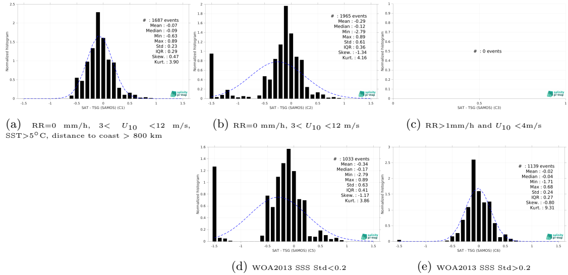
Figure 15: Normalized histogram of \Delta SSS (SMOS SSS L4 v1 - Daily (CMEMS-CNR) - TSG (SAMOS)) for 5 different subdatasets corresponding to: RR=0 mm/h, 3 < U_{10} < 12 m/s, SST > 5°C, distance to coast > 800 km (a), RR=0 mm/h, 3 < U_{10} < 12 m/s (b), RR > 1mm/h and U_{10} < 4 m/s (c), WOA2013 SSS Std < 0.2 (d), WOA2013 SSS Std > 0.2 (e).
