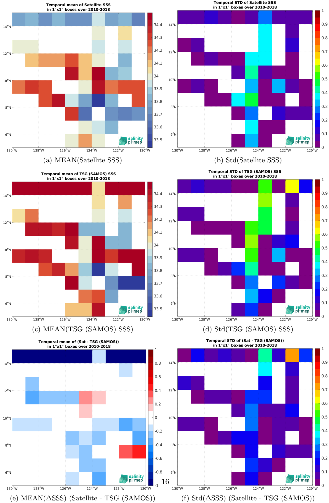
Figure 7: Temporal mean (left) and Std (right) of SSS from SMOS SSS L4 v1 - Daily (CMEMS-CNR) (top), TSG (SAMOS) (middle), and of \Delta SSS (Satellite - TSG (SAMOS)). Only match-up pairs are used to generate these maps.
