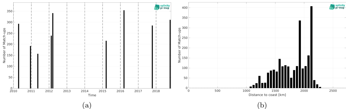
Figure 2: Number of match-ups between TSG (SAMOS) and SMOS SSS L4 v1 - Daily (CMEMS-CNR) SSS as a function of time (a) and as function of the distance to coast (b) over the SPURS 2 Pi-MEP region and for the full satellite product period.
