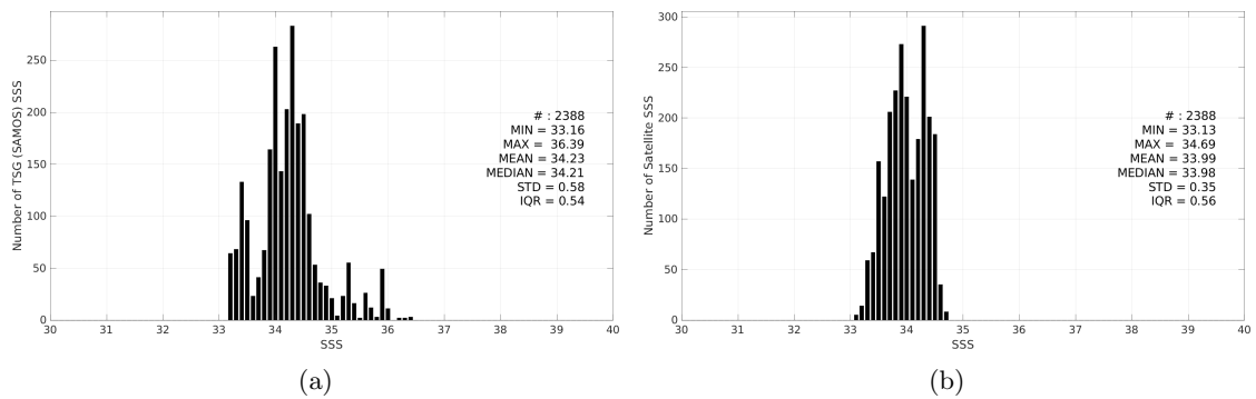
Figure 3: Histograms of SSS from TSG (SAMOS) (a) and SMOS SSS L4 v1 - Daily (CMEMS-CNR) (b) considering all match-up pairs per bins of 0.1 over the SPURS 2 Pi-MEP region and for the full satellite product period.
