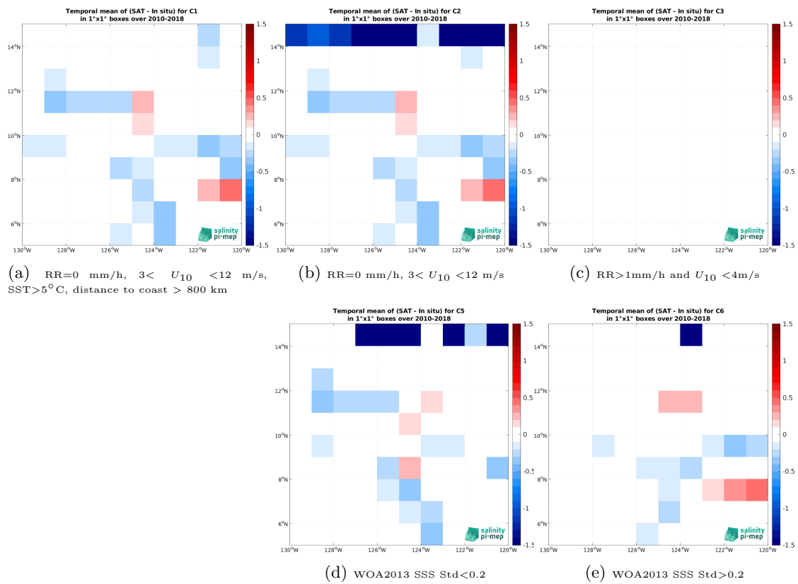
Figure 14: Temporal mean gridded over spatial boxes of size 1^\circ \times 1^\circ of \Delta\text{SSS} (SMOS SSS L4 v1 - Daily (CMEMS-CNR) - TSG (SAMOS)) for 5 different subdatasets corresponding to:RR=0 mm/h, 3 < U_{10} < 12 m/s, SST > 5°C, distance to coast > 800 km (a), RR=0 mm/h, 3 < U_{10} < 12 m/s (b), RR > 1mm/h and U_{10} < 4 m/s (c), WOA2013 SSS Std < 0.2 (d), WOA2013 SSS Std > 0.2 (e).
