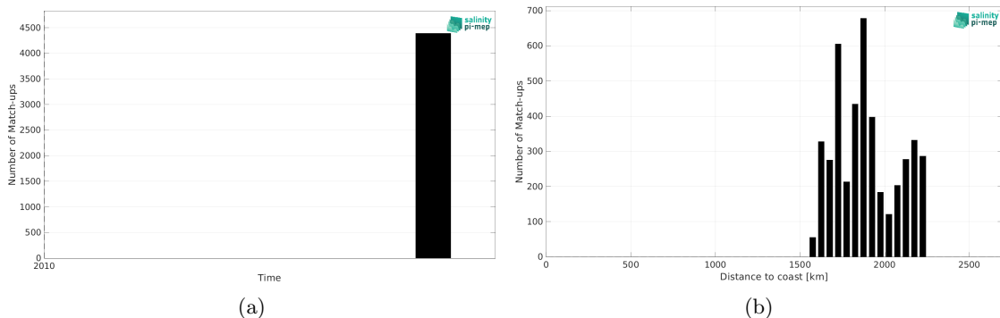
Figure 2: Number of match-ups between TSG (GOSUD-Sailing-ship) and SMOS SSS L4 v1 - Daily (CMEMS-CNR) SSS as a function of time (a) and as function of the distance to coast (b) over the SPURS 2 Pi-MEP region and for the full satellite product period.
