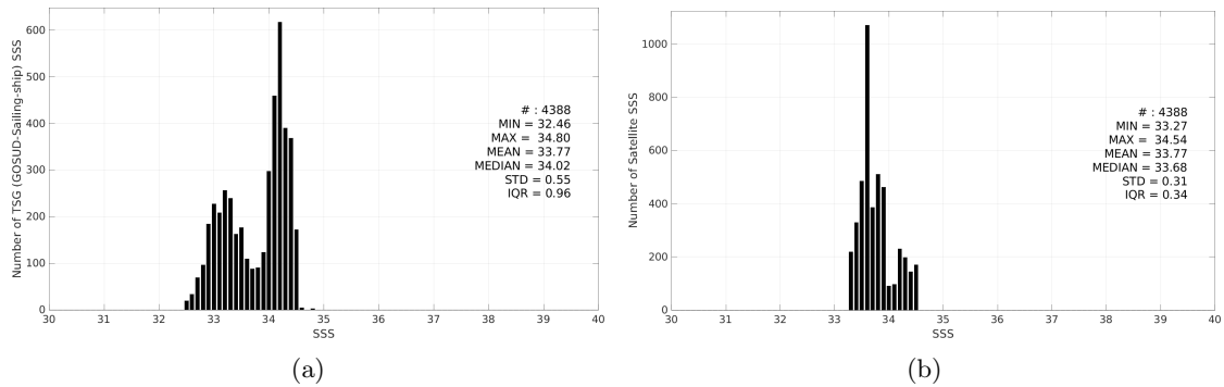
Figure 3: Histograms of SSS from TSG (GOSUD-Sailing-ship) (a) and SMOS SSS L4 v1 - Daily (CMEMS-CNR) (b) considering all match-up pairs per bins of 0.1 over the SPURS 2 Pi-MEP region and for the full satellite product period.
