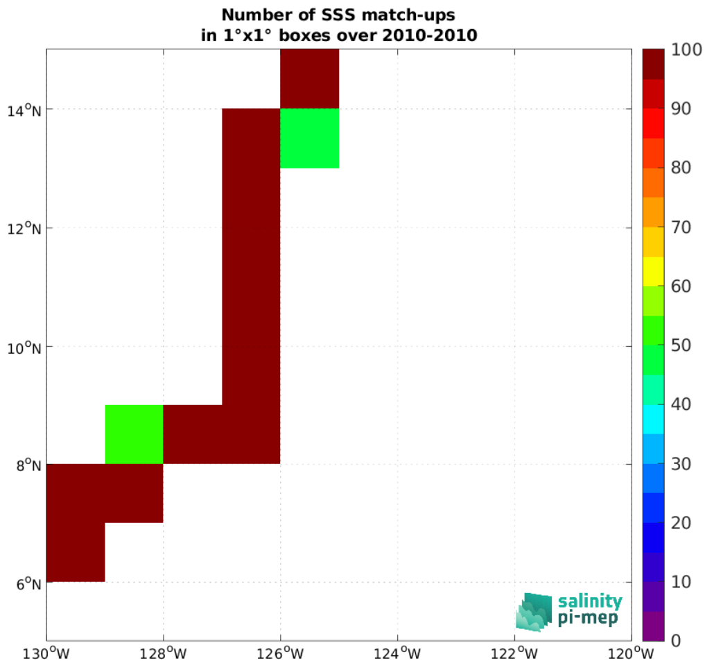
Figure 5: Number of SSS match-ups between TSG (GOSUD-Sailing-ship) SSS and the SMOS SSS L4 v1 - Daily (CMEMS-CNR) SSS product for the SPURS 2 Pi-MEP region over 1°x1° boxes and for the full satellite product period.
