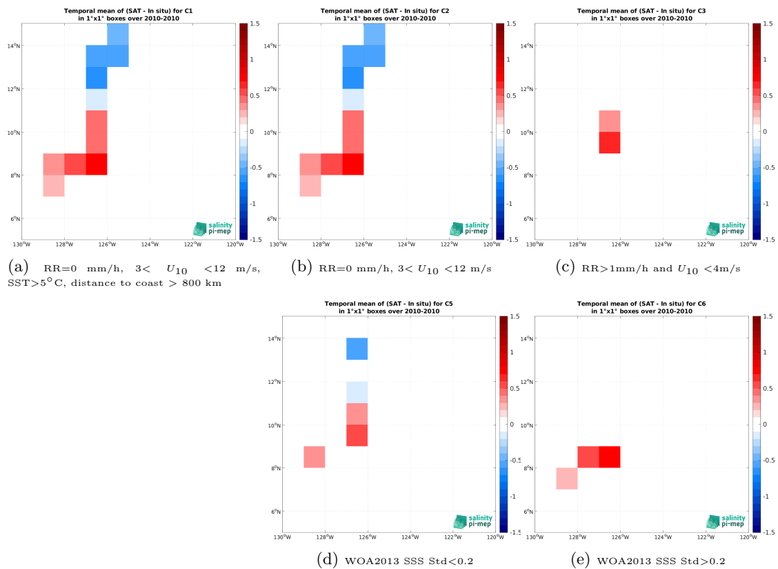
Figure 14: Temporal mean gridded over spatial boxes of size 1^\circ \times 1^\circ of \Delta\text{SSS} (SMOS SSS L4 v1 - Daily (CMEMS-CNR) - TSG (GOSUD-Sailing-ship)) for 5 different subdatasets corresponding to:RR=0 mm/h, 3 < U_{10} < 12 m/s, SST>5°C, distance to coast > 800 km (a), RR=0 mm/h, 3 < U_{10} < 12 m/s (b), RR>1mm/h and U_{10} < 4 m/s (c), WOA2013 SSS Std<0.2 (d), WOA2013 SSS Std>0.2 (e).
