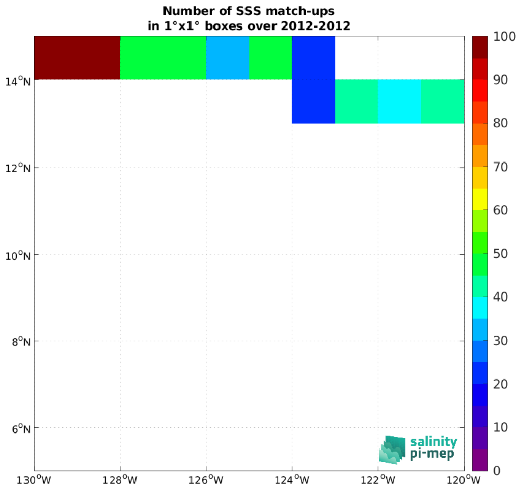
Figure 5: Number of SSS match-ups between TSG (GOSUD-Research-vessel) SSS and the SMOS SSS L4 v1 - Daily (CMEMS-CNR) SSS product for the SPURS 2 Pi-MEP region over 1°x1° boxes and for the full satellite product period.
