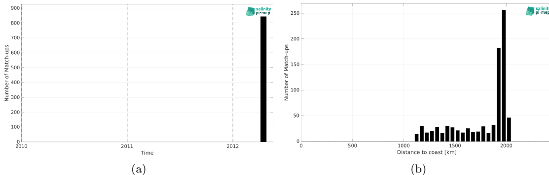
Figure 2: Number of match-ups between TSG (GOSUD-Research-vessel) and SMOS SSS L4 v1 - Daily (CMEMS-CNR) SSS as a function of time (a) and as function of the distance to coast (b) over the SPURS 2 Pi-MEP region and for the full satellite product period.
