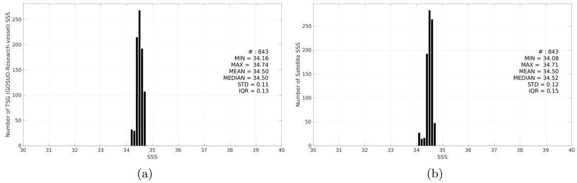
Figure 3: Histograms of SSS from TSG (GOSUD-Research-vessel) (a) and SMOS SSS L4 v1 - Daily (CMEMS-CNR) (b) considering all match-up pairs per bins of 0.1 over the SPURS 2 Pi-MEP region and for the full satellite product period.
