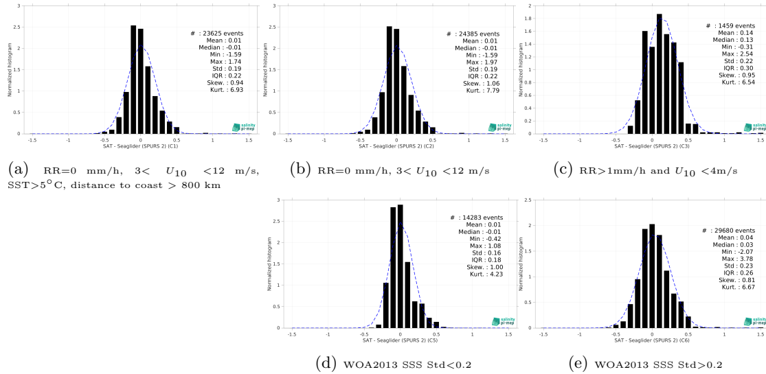
Figure 15: Normalized histogram of \Delta\text{SSS} (SMOS SSS L4 v1 - Daily (CMEMS-CNR) - Seaglider (SPURS 2)) for 5 different subdatasets corresponding to: RR=0 mm/h, 3 < U_{10} < 12 m/s, SST>5°C, distance to coast > 800 km (a), RR=0 mm/h, 3 < U_{10} < 12 m/s (b), RR>1mm/h and U_{10} < 4 m/s (c), WOA2013 SSS Std<0.2 (d), WOA2013 SSS Std>0.2 (e).
