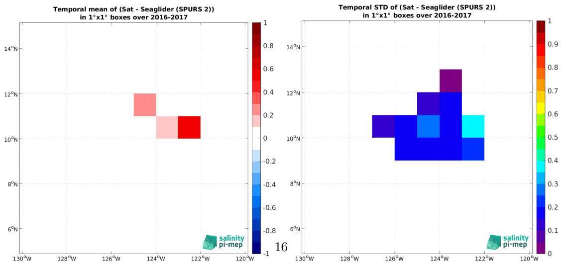
(e) MEAN( \Delta SSS) (Satellite - Seaglider (SPURS 2)) (f) Std( \Delta SSS) (Satellite - Seaglider (SPURS 2))
