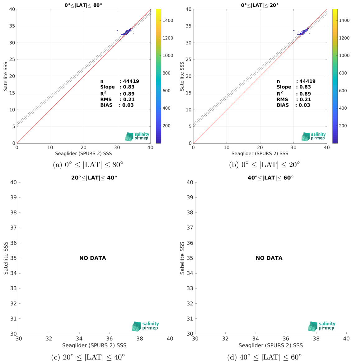
Figure 10: Contour maps of the concentration of SMOS SSS L4 v1 - Daily (CMEMS-CNR) SSS (y-axis) versus Seaglider (SPURS 2) SSS (x-axis) at match-up pairs for different latitude bands. For each plot, the red line shows x=y . The black thin and dashed lines indicate a linear fit through the data cloud and the \pm 95\% confidence levels, respectively. The number match-up pairs n , the slope and R^2 coefficient of the linear fit, the root mean square (RMS) and the mean bias between satellite and in situ data are indicated for each latitude band in each plots.
