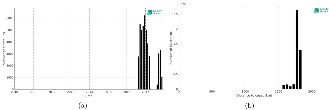
Figure 2: Number of match-ups between Seaglider (SPURS 2) and SMOS SSS L4 v1 - Daily (CMEMS-CNR) SSS as a function of time (a) and as function of the distance to coast (b) over the SPURS 2 Pi-MEP region and for the full satellite product period.
