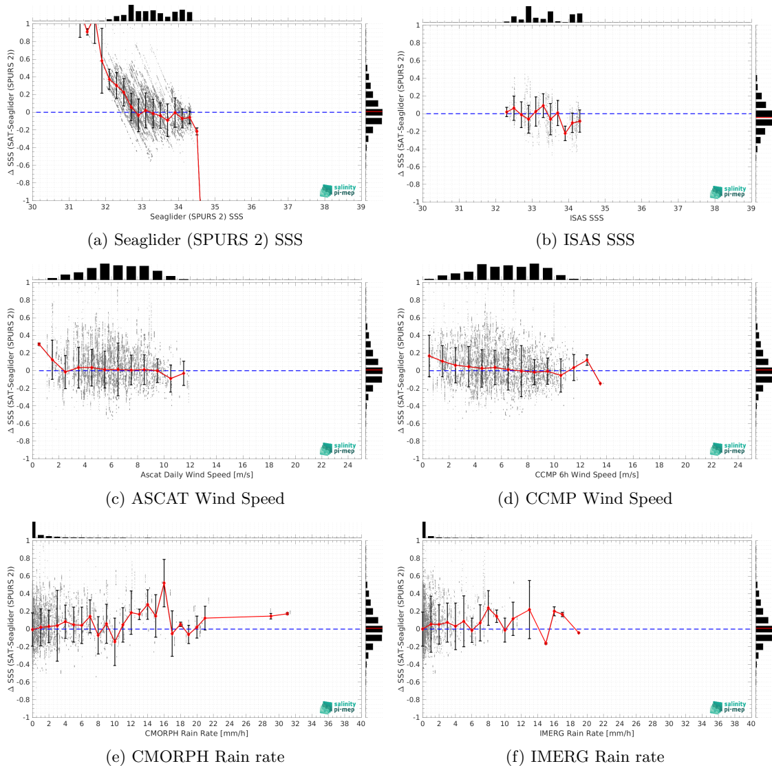
Figure 12: \Delta \text{SSS} (Satellite - Seaglider (SPURS 2)) sorted as function of Seaglider (SPURS 2) SSS values (a), ISAS SSS (b), ASCAT Wind speed (c), CCMP Wind speed (d), CMORPH rain rate (e) and IMERG rain rate (f). In all plots the median and Std of \Delta \text{SSS} for each bin is indicated by the red curves and black vertical thick bars ( \pm 1 \text{ Std} ).
