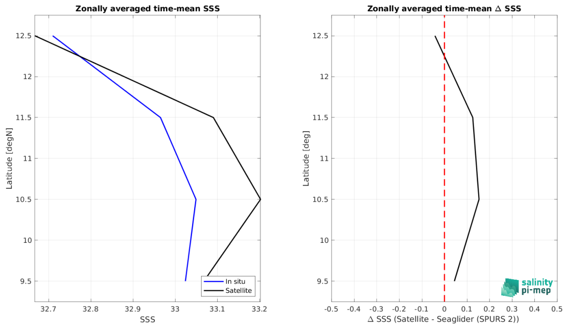
Figure 9: Left panel: Zonal mean SSS from SMOS SSS L4 v1 - Daily (CMEMS-CNR) satellite product (black) and from Seaglider (SPURS 2) (blue). Right panel: Zonal mean of \Delta SSS (Satellite - Seaglider (SPURS 2)) for all the collected Pi-MEP match-up pairs estimated over the full satellite product period.
