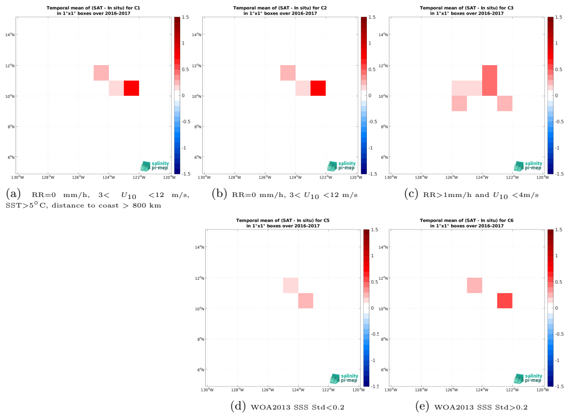
Figure 14: Temporal mean gridded over spatial boxes of size 1^\circ \times 1^\circ of \Delta SSS (SMOS SSS L4 v1 - Daily (CMEMS-CNR) - Seaglider (SPURS 2)) for 5 different subdatasets corresponding to:RR=0 mm/h, 3 < U_{10} < 12 m/s, SST>5°C, distance to coast > 800 km (a), RR=0 mm/h, 3 < U_{10} < 12 m/s (b), RR>1mm/h and U_{10} < 4 m/s (c), WOA2013 SSS Std<0.2 (d), WOA2013 SSS Std>0.2 (e).
