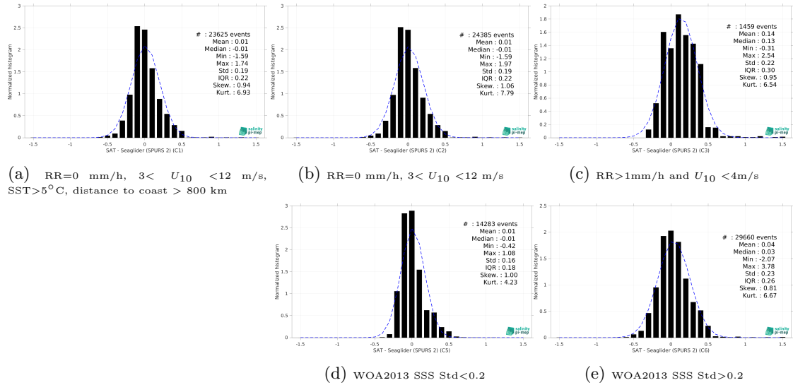
Figure 15: Normalized histogram of \Delta SSS (SMOS SSS L4 v1 - Daily (CMEMS-CNR) - Seaglider (SPURS 2)) for 5 different subdatasets corresponding to: RR=0 mm/h, 3 < U_{10} < 12 m/s, SST>5°C, distance to coast > 800 km (a), RR=0 mm/h, 3 < U_{10} < 12 m/s (b), RR>1mm/h and U_{10} < 4 m/s (c), WOA2013 SSS Std<0.2 (d), WOA2013 SSS Std>0.2 (e).
