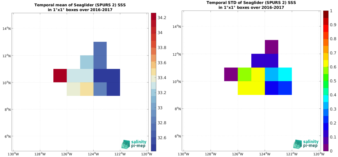
(c) MEAN(Seaglider (SPURS 2) SSS)
