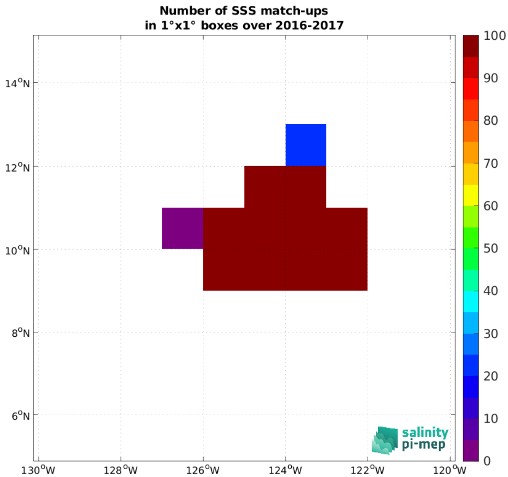
Figure 5: Number of SSS match-ups between Seaglider (SPURS 2) SSS and the SMOS SSS L4 v1 - Daily (CMEMS-CNR) SSS product for the SPURS 2 Pi-MEP region over 1^\circ \times 1^\circ boxes and for the full satellite product period.
