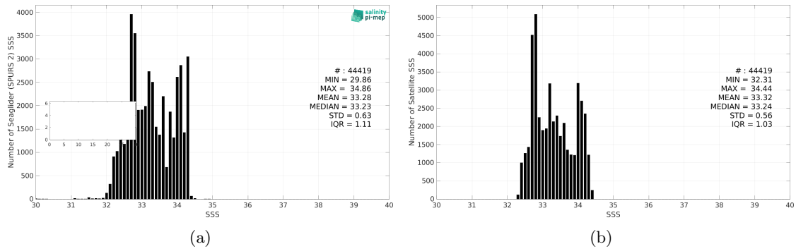
Figure 3: Histograms of SSS from Seaglider (SPURS 2) (a) and SMOS SSS L4 v1 - Daily (CMEMS-CNR) (b) considering all match-up pairs per bins of 0.1 over the SPURS 2 Pi-MEP region and for the full satellite product period.
