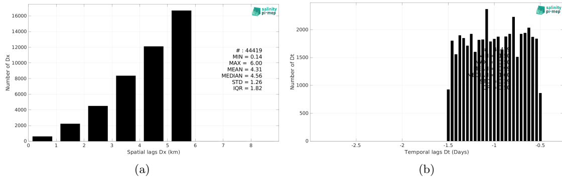
Figure 6: Histograms of the spatial (a) and temporal (b) lags between the location/time of the Seaglider (SPURS 2) measurement and the date of the corresponding SMOS SSS L4 v1 - Daily (CMEMS-CNR) SSS pixel.
