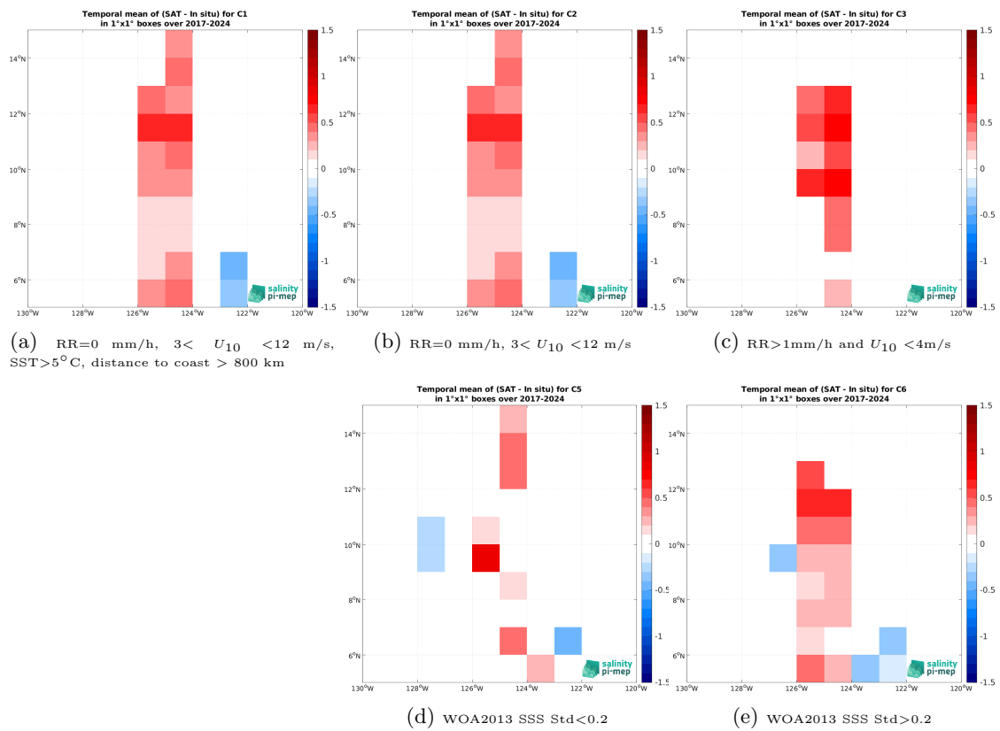
Figure 14: Temporal mean gridded over spatial boxes of size 1^\circ \times 1^\circ of \Delta SSS (SMOS SSS L4 v1 - Daily (CMEMS-CNR) - Sairdrone) for 5 different subdatasets corresponding to:RR=0 mm/h, 3 < U_{10} < 12 m/s, SST >5^\circ\text{C} , distance to coast > 800 km (a), RR=0 mm/h, 3 < U_{10} < 12 m/s (b), RR >1 mm/h and U_{10} < 4 m/s (c), WOA2013 SSS Std <0.2 (d), WOA2013 SSS Std >0.2 (e).
