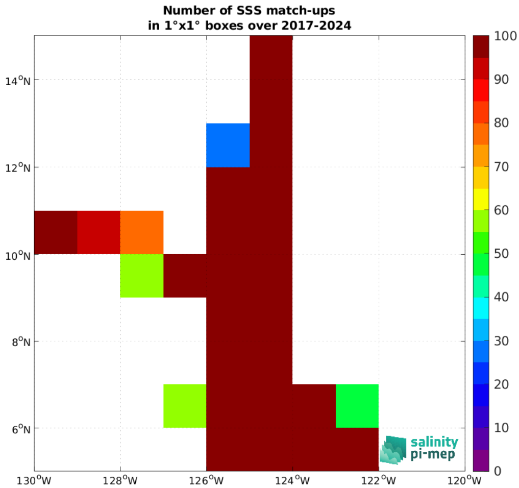
Figure 5: Number of SSS match-ups between Saildrone SSS and the SMOS SSS L4 v1 - Daily (CMEMS-CNR) SSS product for the SPURS 2 Pi-MEP region over 1^\circ \times 1^\circ boxes and for the full satellite product period.
