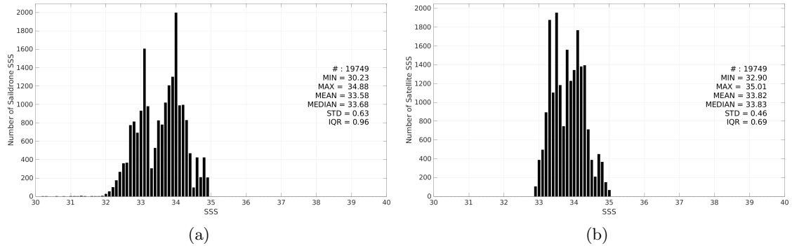
Figure 3: Histograms of SSS from Saildrone (a) and SMOS SSS L4 v1 - Daily (CMEMS-CNR) (b) considering all match-up pairs per bins of 0.1 over the SPURS 2 Pi-MEP region and for the full satellite product period.
