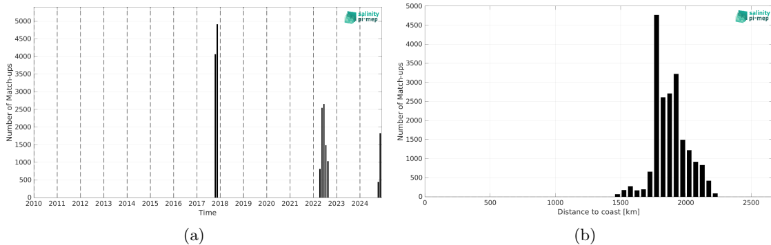
Figure 2: Number of match-ups between Saildrone and SMOS SSS L4 v1 - Daily (CMEMS-CNR) SSS as a function of time (a) and as function of the distance to coast (b) over the SPURS 2 Pi-MEP region and for the full satellite product period.
