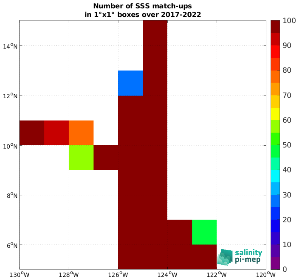
Figure 5: Number of SSS match-ups between Saildrone SSS and the SMOS SSS L4 v1 - Daily (CMEMS-CNR) SSS product for the SPURS 2 Pi-MEP region over 1°x1° boxes and for the full satellite product period.
