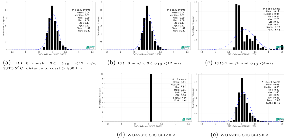
Figure 15: Normalized histogram of \Delta SSS (SMOS SSS L4 v1 - Daily (CMEMS-CNR) - Saldrone (SPURS 2)) for 5 different subdatasets corresponding to: RR=0 mm/h, 3 < U_{10} < 12 m/s, SST > 5°C, distance to coast > 800 km (a), RR=0 mm/h, 3 < U_{10} < 12 m/s (b), RR > 1mm/h and U_{10} < 4 m/s (c), WOA2013 SSS Std < 0.2 (d), WOA2013 SSS Std > 0.2 (e).
