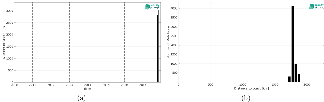
Figure 2: Number of match-ups between Sairdron (SPURS 2) and SMOS SSS L4 v1 - Daily (CMEMS-CNR) SSS as a function of time (a) and as function of the distance to coast (b) over the SPURS 2 Pi-MEP region and for the full satellite product period.
