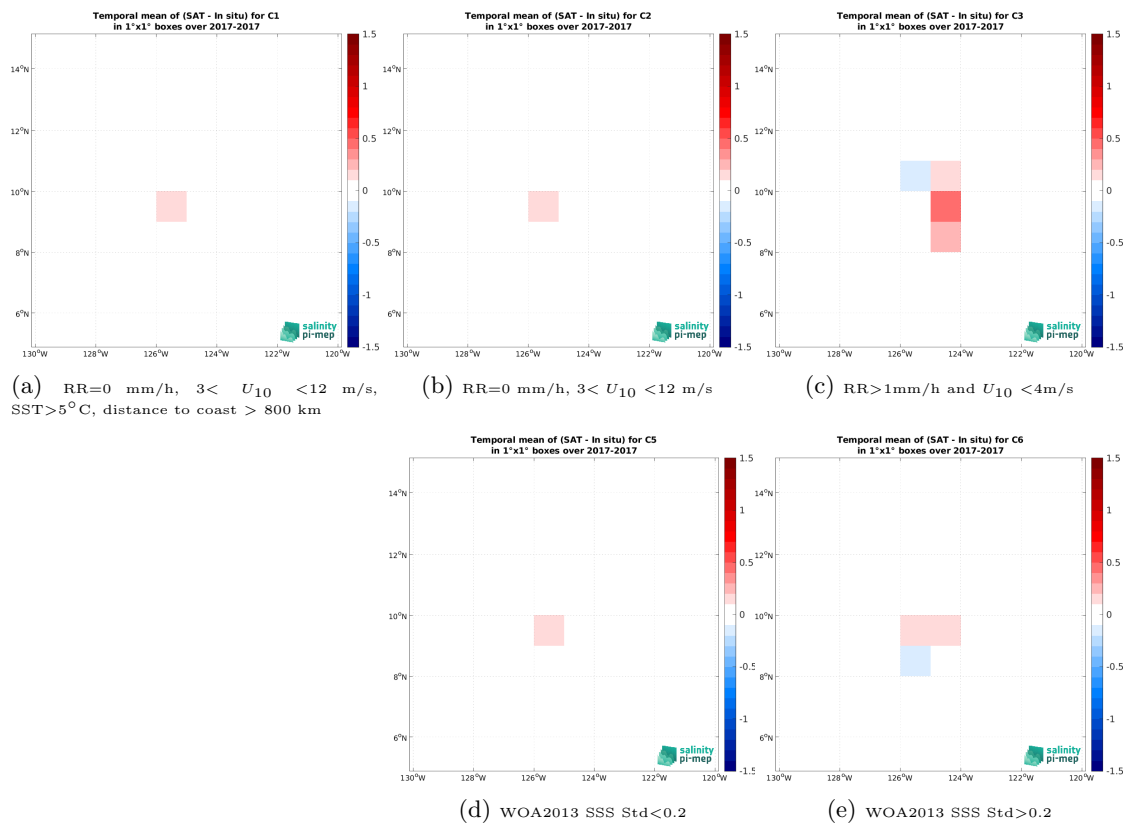
Figure 14: Temporal mean gridded over spatial boxes of size 1^\circ \times 1^\circ of \Delta SSS (SMOS SSS L4 v1 - Daily (CMEMS-CNR) - Saifdrone (SPURS 2)) for 5 different subdatasets corresponding to:RR=0 mm/h, 3 < U_{10} < 12 m/s, SST >5^\circ C, distance to coast > 800 km (a), RR=0 mm/h, 3 < U_{10} < 12 m/s (b), RR >1 mm/h and U_{10} < 4 m/s (c), WOA2013 SSS Std <0.2 (d), WOA2013 SSS Std >0.2 (e).
