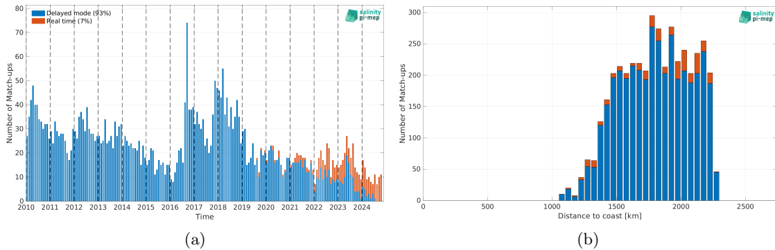
Figure 2: Number of match-ups between Argo and SMOS SSS L4 v1 - Daily (CMEMS-CNR) SSS as a function of time (a) and as function of the distance to coast (b) over the SPURS 2 Pi-MEP region and for the full satellite product period.
