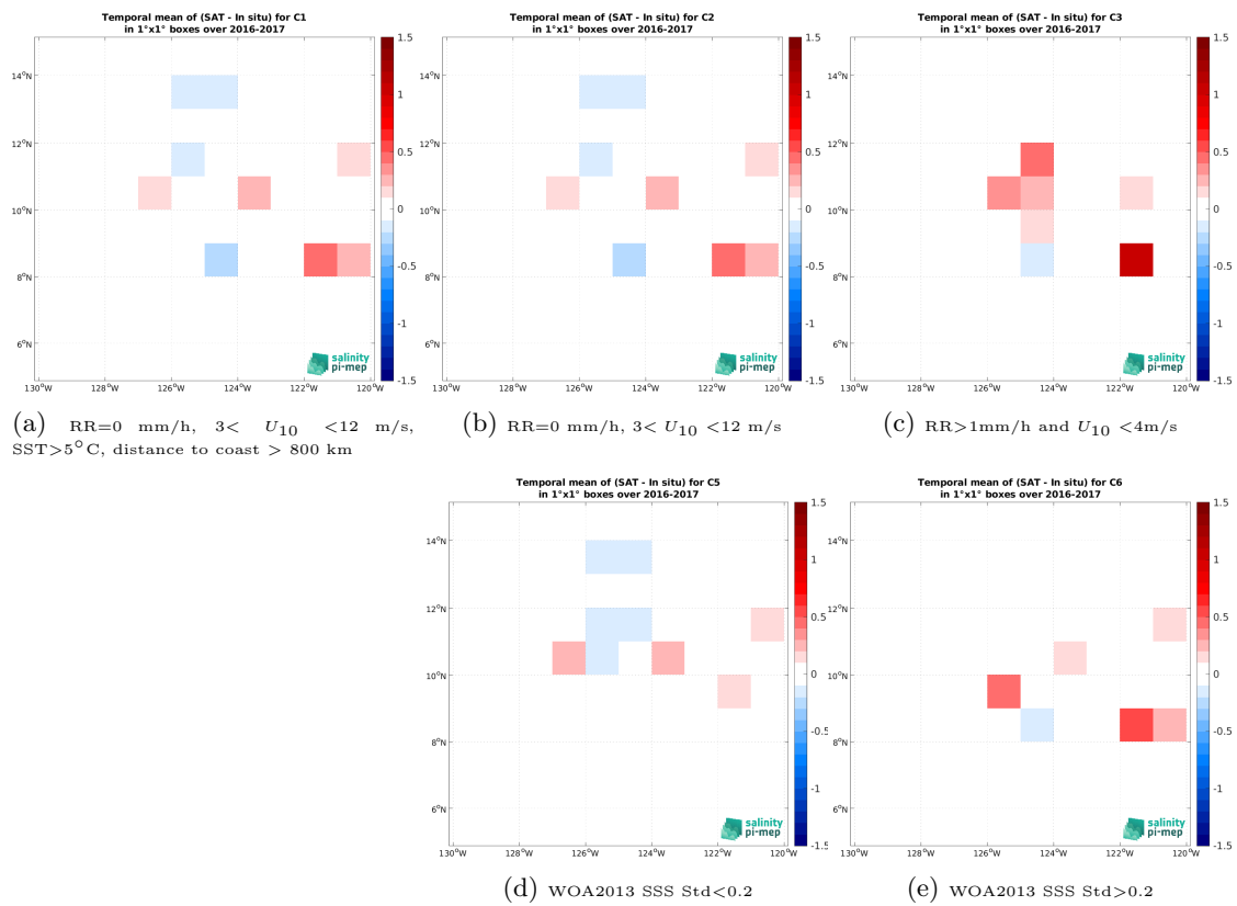
Figure 14: Temporal mean gridded over spatial boxes of size 1^\circ \times 1^\circ of \Delta SSS (SMOS SSS L4 OI v346 - Weekly (CMEMS-CATDS-LOPS) - Waveglider (SPURS 2)) for 5 different subdatasets corresponding to:RR=0 mm/h, 3 < U_{10} < 12 m/s, SST >5^\circ C, distance to coast > 800 km (a), RR=0 mm/h, 3 < U_{10} < 12 m/s (b), RR >1 mm/h and U_{10} < 4 m/s (c), WOA2013 SSS Std <0.2 (d), WOA2013 SSS Std >0.2 (e).
