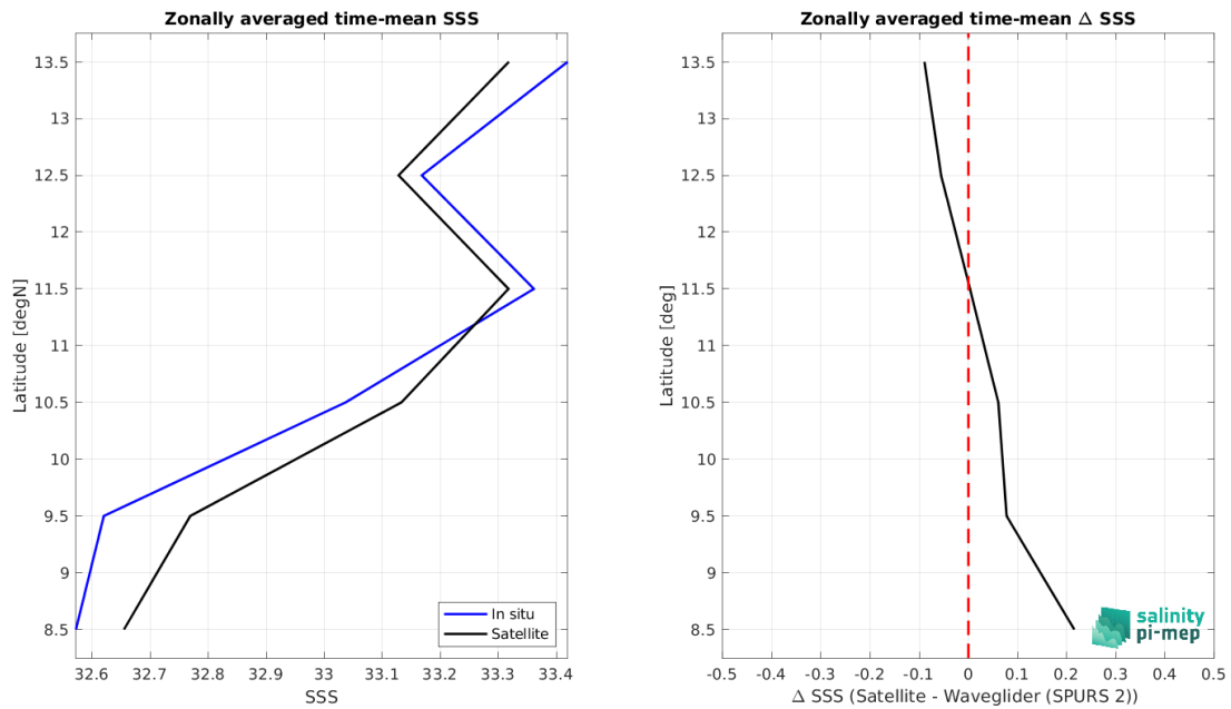
Figure 9: Left panel: Zonal mean SSS from SMOS SSS L4 OI v346 - Weekly (CMEMS-CATDS-LOPS) satellite product (black) and from Waveglider (SPURS 2) (blue). Right panel: Zonal mean of \Delta SSS (Satellite - Waveglider (SPURS 2)) for all the collected Pi-MEP match-up pairs estimated over the full satellite product period.
