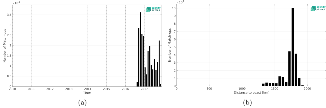
Figure 2: Number of match-ups between Waveglider (SPURS 2) and SMOS SSS L4 OI v346 - Weekly (CMEMS-CATDS-LOPS) SSS as a function of time (a) and as function of the distance to coast (b) over the SPURS 2 Pi-MEP region and for the full satellite product period.
