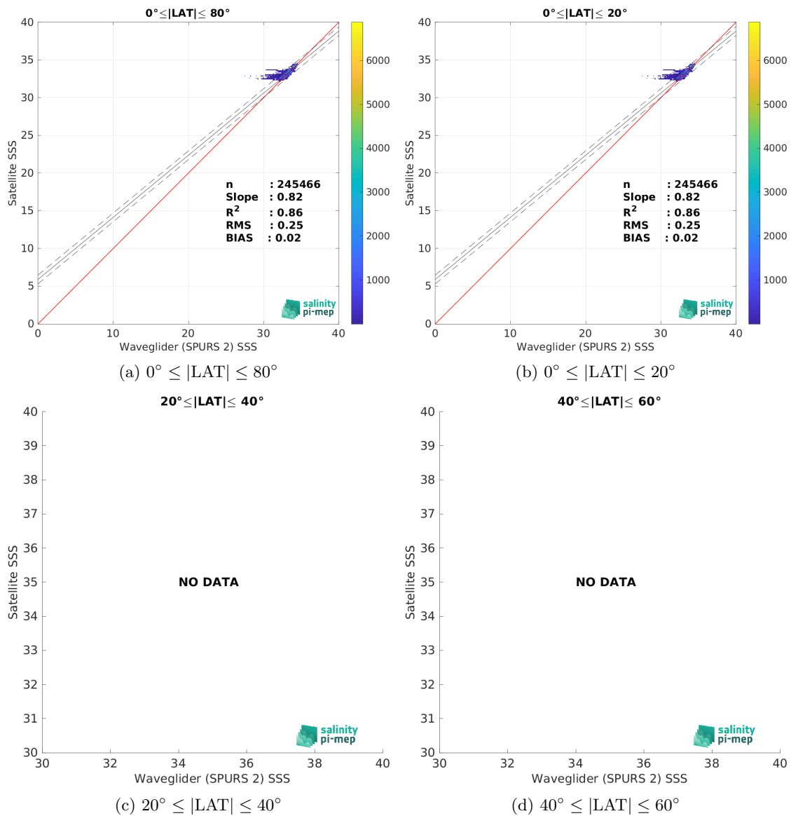
Figure 10: Contour maps of the concentration of SMOS SSS L4 OI v346 - Weekly (CMEMS-CATDS-LOPS) SSS (y-axis) versus Waveglider (SPURS 2) SSS (x-axis) at match-up pairs for different latitude bands. For each plot, the red line shows x=y . The black thin and dashed lines indicate a linear fit through the data cloud and the \pm 95\% confidence levels, respectively. The number match-up pairs n , the slope and R^2 coefficient of the linear fit, the root mean square (RMS) and the mean bias between satellite and in situ data are indicated for each latitude band in each plots.
