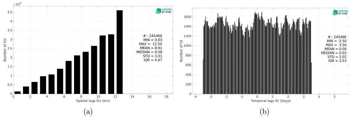
Figure 6: Histograms of the spatial (a) and temporal (b) lags between the location/time of the Waveglider (SPURS 2) measurement and the date of the corresponding SMOS SSS L4 OI v346 - Weekly (CMEMS-CATDS-LOPS) SSS pixel.
