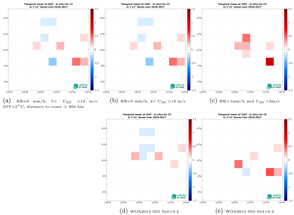
Figure 14: Temporal mean gridded over spatial boxes of size 1^\circ \times 1^\circ of \Delta\text{SSS} (SMOS SSS L4 OI v346 - Weekly (CMEMS-CATDS-LOPS) - Waveglider (SPURS 2)) for 5 different subdatasets corresponding to:RR=0 mm/h, 3 < U_{10} < 12 m/s, SST >5^\circ\text{C} , distance to coast > 800 km (a), RR=0 mm/h, 3 < U_{10} < 12 m/s (b), RR >1 mm/h and U_{10} < 4 m/s (c), WOA2013 SSS Std <0.2 (d), WOA2013 SSS Std >0.2 (e).
