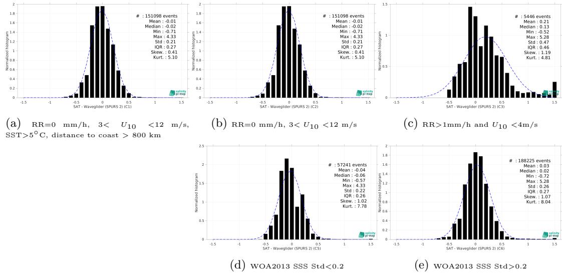
Figure 15: Normalized histogram of \Delta SSS (SMOS SSS L4 OI v346 - Weekly (CMEMS-CATDS-LOPS) - Waveglider (SPURS 2)) for 5 different subdatasets corresponding to: RR=0 mm/h, 3 < U_{10} < 12 m/s, SST > 5°C, distance to coast > 800 km (a), RR=0 mm/h, 3 < U_{10} < 12 m/s (b), RR > 1mm/h and U_{10} < 4 m/s (c), WOA2013 SSS Std < 0.2 (d), WOA2013 SSS Std > 0.2 (e).
