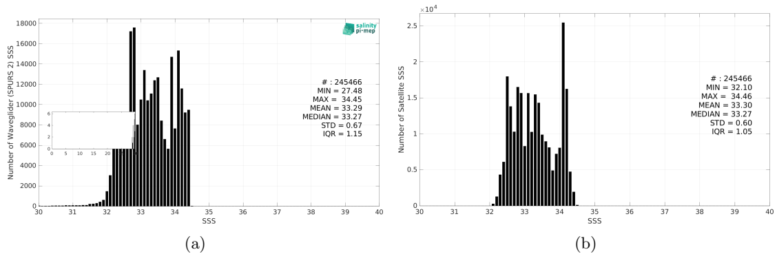
Figure 3: Histograms of SSS from Waveglider (SPURS 2) (a) and SMOS SSS L4 OI v346 - Weekly (CMEMS-CATDS-LOPS) (b) considering all match-up pairs per bins of 0.1 over the SPURS 2 Pi-MEP region and for the full satellite product period.
