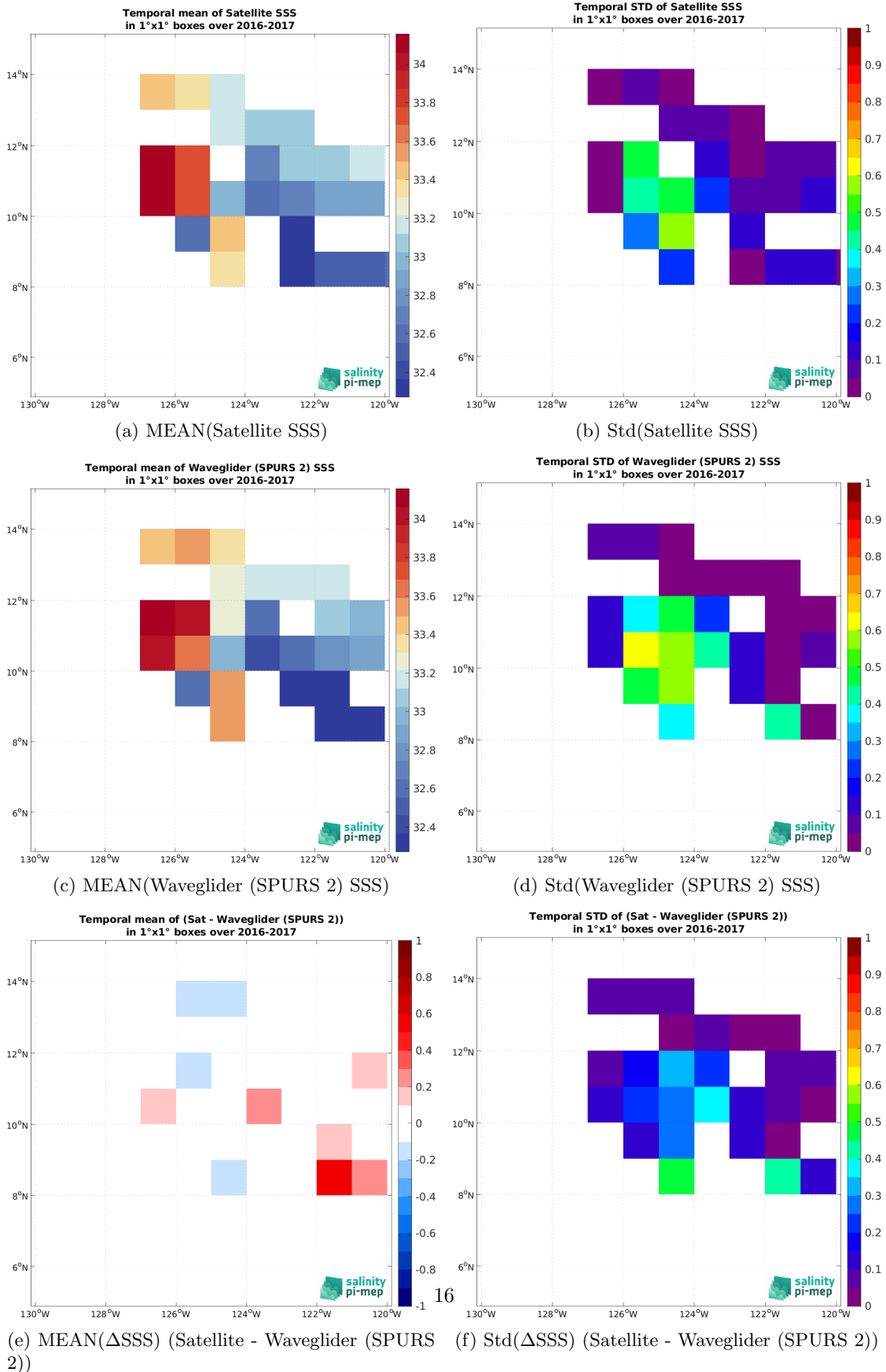
Figure 7: Temporal mean (left) and Std (right) of SSS from SMOS SSS L4 OI v346 - Weekly (CMEMS-CATDS-LOPS) (top), Waveglider (SPURS 2) (middle), and of \Delta SSS (Satellite - Waveglider (SPURS 2)). Only match-up pairs are used to generate these maps.
