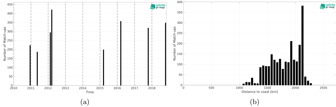
Figure 2: Number of match-ups between TSG (SAMOS) and SMOS SSS L4 OI v346 - Weekly (CMEMS-CATDS-LOPS) SSS as a function of time (a) and as function of the distance to coast (b) over the SPURS 2 Pi-MEP region and for the full satellite product period.
