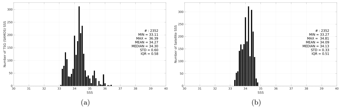
Figure 3: Histograms of SSS from TSG (SAMOS) (a) and SMOS SSS L4 OI v346 - Weekly (CMEMS-CATDS-LOPS) (b) considering all match-up pairs per bins of 0.1 over the SPURS 2 Pi-MEP region and for the full satellite product period.
