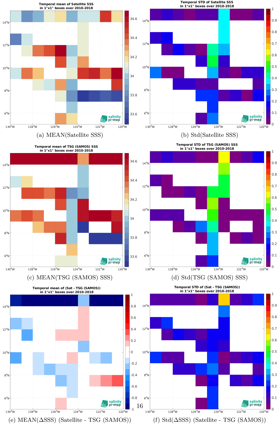
Figure 7: Temporal mean (left) and Std (right) of SSS from SMOS SSS L4 OI v346 - Weekly (CMEMS-CATDS-LOPS) (top), TSG (SAMOS) (middle), and of \Delta SSS (Satellite - TSG (SAMOS)). Only match-up pairs are used to generate these maps.
