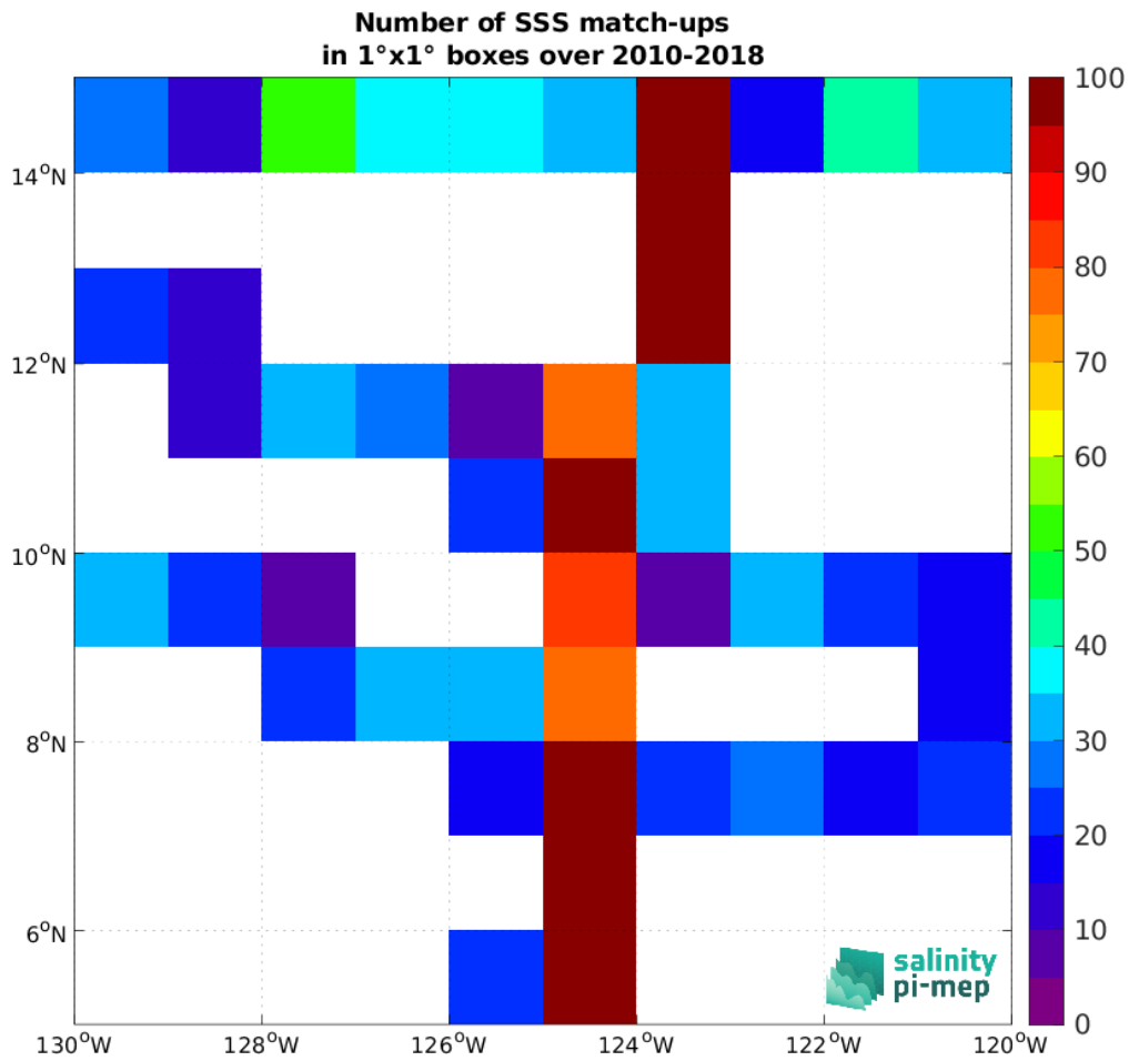
Figure 5: Number of SSS match-ups between TSG (SAMOS) SSS and the SMOS SSS L4 OI v346 - Weekly (CMEMS-CATDS-LOPS) SSS product for the SPURS 2 Pi-MEP region over 1°x1° boxes and for the full satellite product period.
