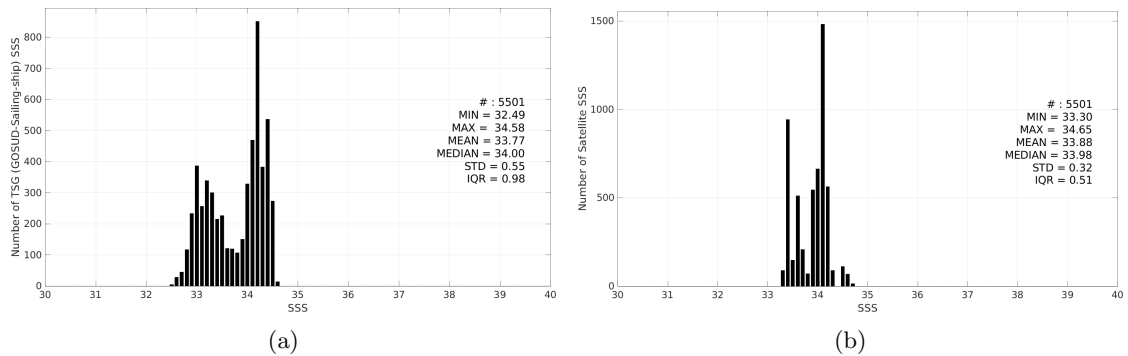
Figure 3: Histograms of SSS from TSG (GOSUD-Sailing-ship) (a) and SMOS SSS L4 OI v346 - Weekly (CMEMS-CATDS-LOPS) (b) considering all match-up pairs per bins of 0.1 over the SPURS 2 Pi-MEP region and for the full satellite product period.
