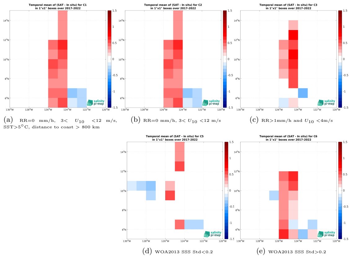
Figure 14: Temporal mean gridded over spatial boxes of size 1^\circ \times 1^\circ of \Delta\text{SSS} (SMOS SSS L4 OI v346 - Weekly (CMEMS-CATDS-LOPS) - Saildrone) for 5 different subdatasets corresponding to: RR=0 mm/h, 3 < U_{10} < 12 m/s, SST > 5°C, distance to coast > 800 km (a), RR=0 mm/h, 3 < U_{10} < 12 m/s (b), RR > 1mm/h and U_{10} < 4 m/s (c), WOA2013 SSS Std < 0.2 (d), WOA2013 SSS Std > 0.2 (e).
