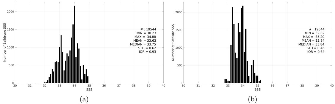
Figure 3: Histograms of SSS from Saildrone (a) and SMOS SSS L4 OI v346 - Weekly (CMEMS-CATDS-LOPS) (b) considering all match-up pairs per bins of 0.1 over the SPURS 2 Pi-MEP region and for the full satellite product period.
