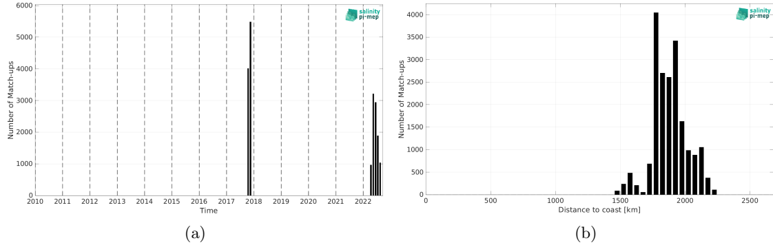
Figure 2: Number of match-ups between Saildrone and SMOS SSS L4 OI v346 - Weekly (CMEMS-CATDS-LOPS) SSS as a function of time (a) and as function of the distance to coast (b) over the SPURS 2 Pi-MEP region and for the full satellite product period.
