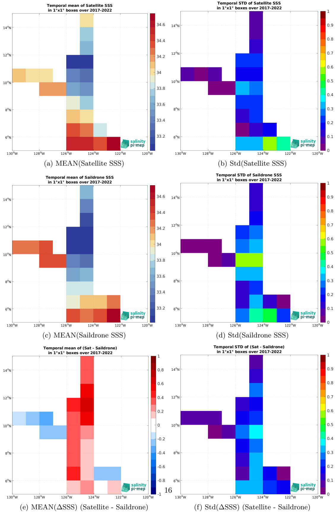
Figure 7: Temporal mean (left) and Std (right) of SSS from SMOS SSS L4 OI v346 - Weekly (CMEMS-CATDS-LOPS) (top), Saildrone (middle), and of \Delta SSS (Satellite - Saildrone). Only match-up pairs are used to generate these maps.
