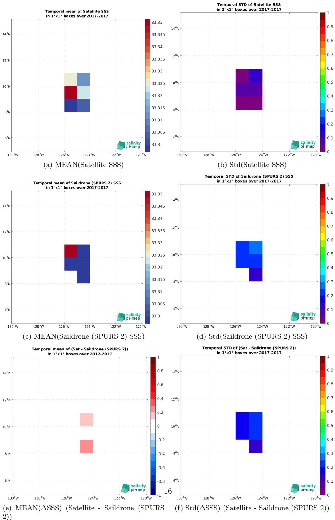
Figure 7: Temporal mean (left) and Std (right) of SSS from SMOS SSS L4 OI v346 - Weekly (CMEMS-CATDS-LOPS) (top), Saildrone (SPURS 2) (middle), and of \Delta SSS (Satellite - Saildrone (SPURS 2)). Only match-up pairs are used to generate these maps.
