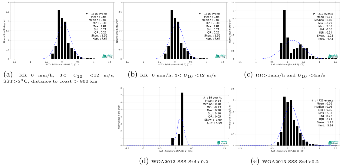
Figure 15: Normalized histogram of \Delta SSS (SMOS SSS L4 OI v346 - Weekly (CMEMS-CATDS-LOPS) - Saldrone (SPURS 2)) for 5 different subdatasets corresponding to: RR=0 mm/h, 3 < U_{10} < 12 m/s, SST > 5°C, distance to coast > 800 km (a), RR=0 mm/h, 3 < U_{10} < 12 m/s (b), RR > 1mm/h and U_{10} < 4 m/s (c), WOA2013 SSS Std < 0.2 (d), WOA2013 SSS Std > 0.2 (e).
