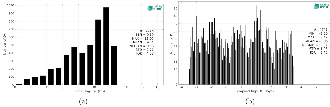
Figure 6: Histograms of the spatial (a) and temporal (b) lags between the location/time of the Saildrone (SPURS 2) measurement and the date of the corresponding SMOS SSS L4 OI v346 - Weekly (CMEMS-CATDS-LOPS) SSS pixel.
