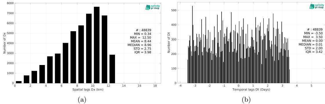
Figure 5: Histograms of the spatial (a) and temporal (b) lags between the location/time of the Seaglider (SPURS 2) measurement and the date of the corresponding SMOS SSS L4 OI v342 - Weekly (CMEMS-CATDS-LOPS) SSS pixel.
