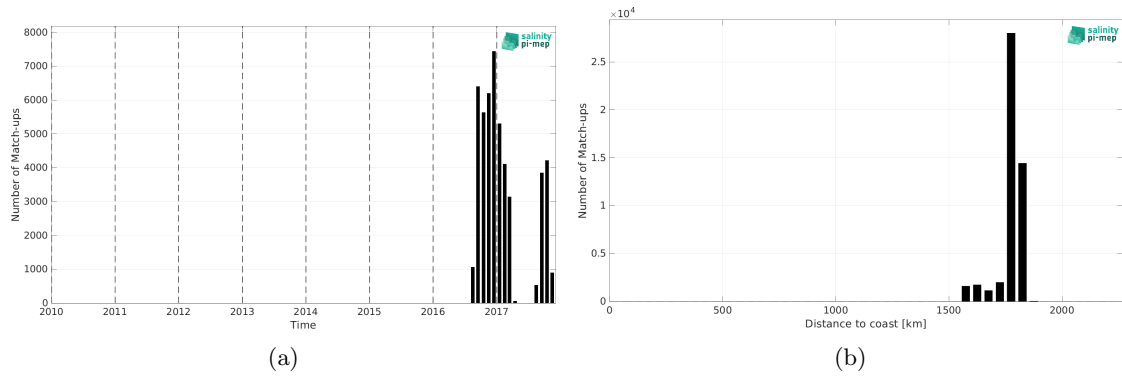
Figure 1: Number of match-ups between Seagliders (SPURS 2) and SMOS SSS L4 OI v342 - Weekly (CMEMS-CATDS-LOPS) SSS as a function of time (a) and as function of the distance to coast (b) over the SPURS 2 Pi-MEP region and for the full satellite product period.
