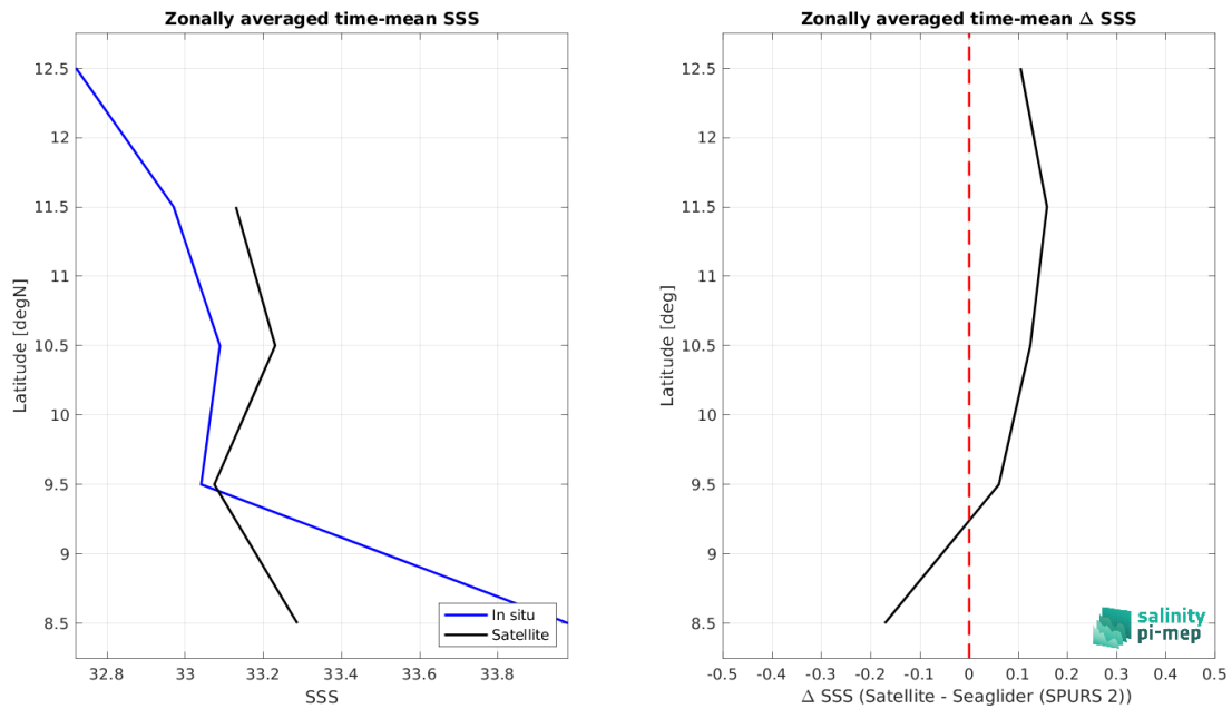
Figure 8: Left panel: Zonal mean SSS from SMOS SSS L4 OI v342 - Weekly (CMEMS-CATDS-LOPS) satellite product (black) and from Seaglider (SPURS 2) (blue). Right panel: Zonal mean of \Delta SSS (Satellite - Seaglider (SPURS 2)) for all the collected Pi-MEP match-up pairs estimated over the full satellite product period.
