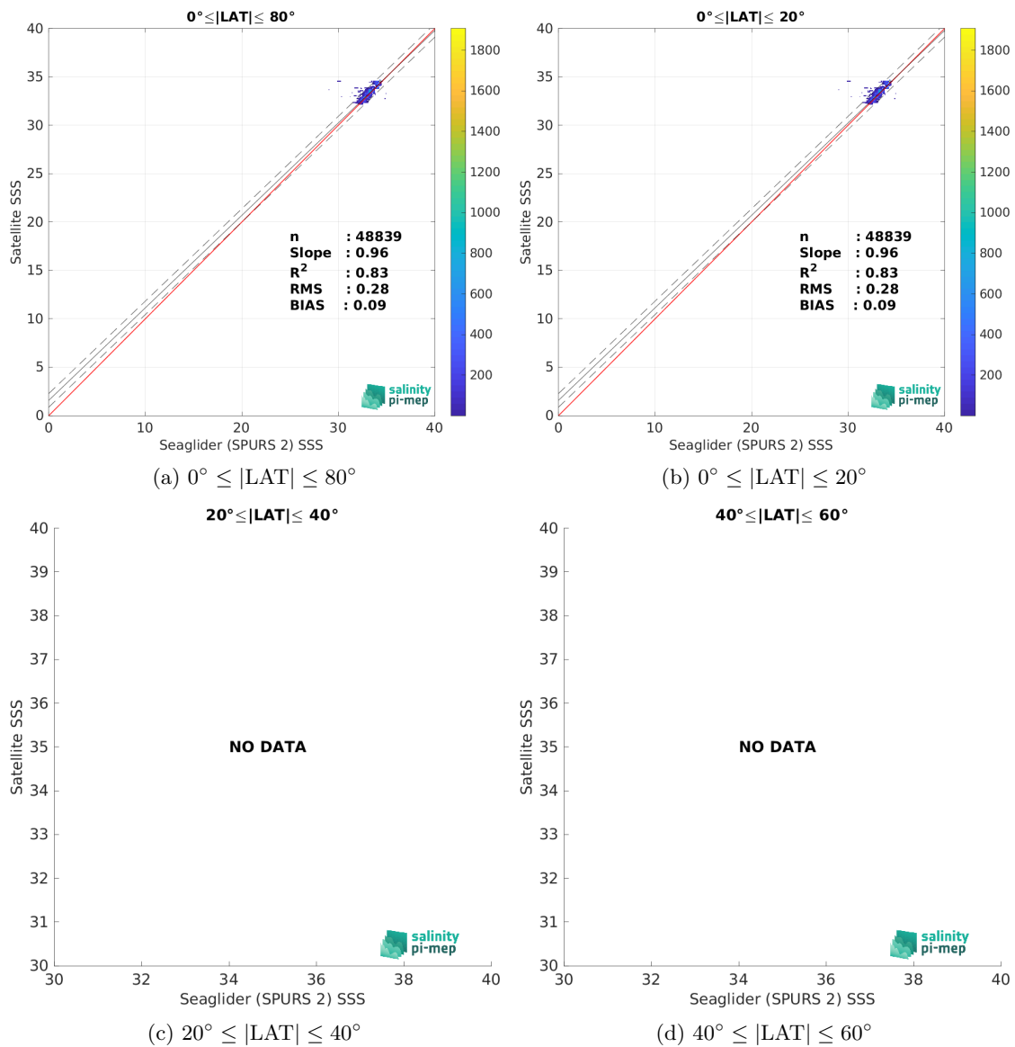
Figure 9: Contour maps of the concentration of SMOS SSS L4 OI v342 - Weekly (CMEMS-CATDS-LOPS) SSS (y-axis) versus Seaglider (SPURS 2) SSS (x-axis) at match-up pairs for different latitude bands. For each plot, the red line shows x=y . The black thin and dashed lines indicate a linear fit through the data cloud and the \pm 95\% confidence levels, respectively. The number match-up pairs n , the slope and R^2 coefficient of the linear fit, the root mean square (RMS) and the mean bias between satellite and in situ data are indicated for each latitude band in each plots.
