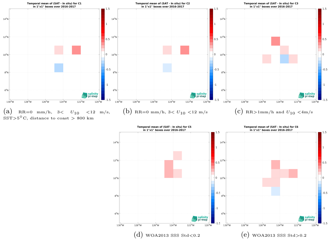
Figure 12: Temporal mean gridded over spatial boxes of size 1^{\circ}\times 1^{\circ} of \Delta\text{SSS} (SMOS SSS L4 OI v342 - Weekly (CMEMS-CATDS-LOPS) - Seaglider (SPURS 2)) for 5 different subdatasets corresponding to:RR=0 mm/h, 3 < U_{10} < 12 m/s, SST > 5^{\circ}\text{C} , distance to coast > 800 km (a), RR=0 mm/h, 3 < U_{10} < 12 m/s (b), RR > 1 mm/h and U_{10} < 4 m/s (c), WOA2013 SSS Std < 0.2 (d), WOA2013 SSS Std > 0.2 (e).
