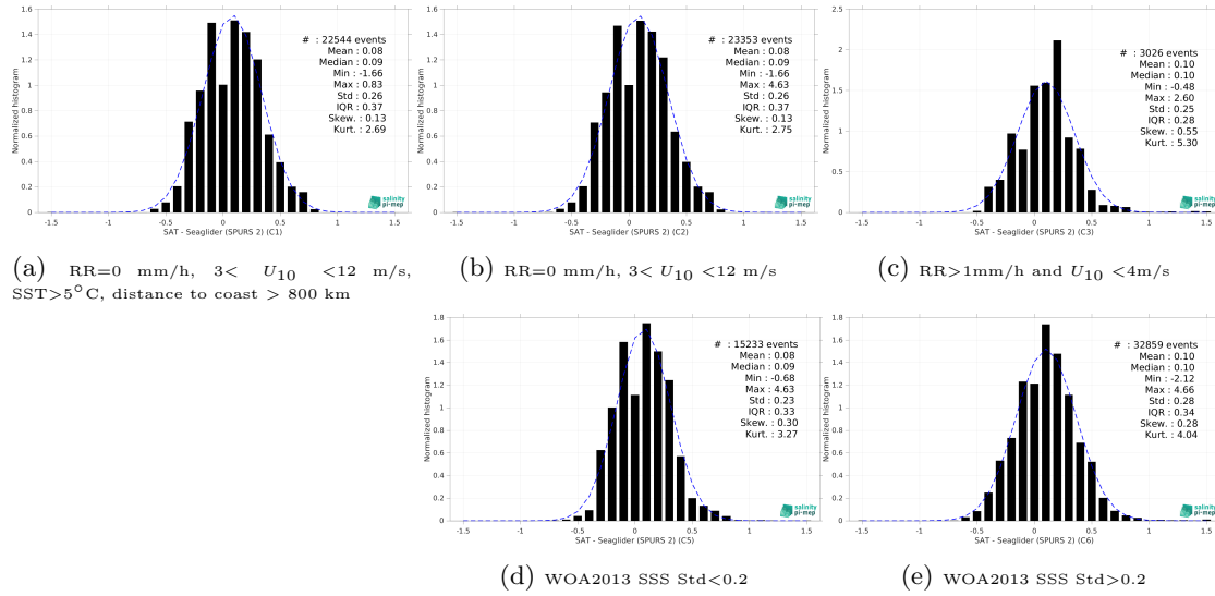
Figure 13: Normalized histogram of \Delta SSS (SMOS SSS L4 OI v342 - Weekly (CMEMS-CATDS-LOPS) - Seaglider (SPURS 2)) for 5 different subdatasets corresponding to: RR=0 mm/h, 3 < U_{10} < 12 m/s, SST>5°C, distance to coast > 800 km (a), RR=0 mm/h, 3 < U_{10} < 12 m/s (b), RR>1mm/h and U_{10} < 4 m/s (c), WOA2013 SSS Std<0.2 (d), WOA2013 SSS Std>0.2 (e).
