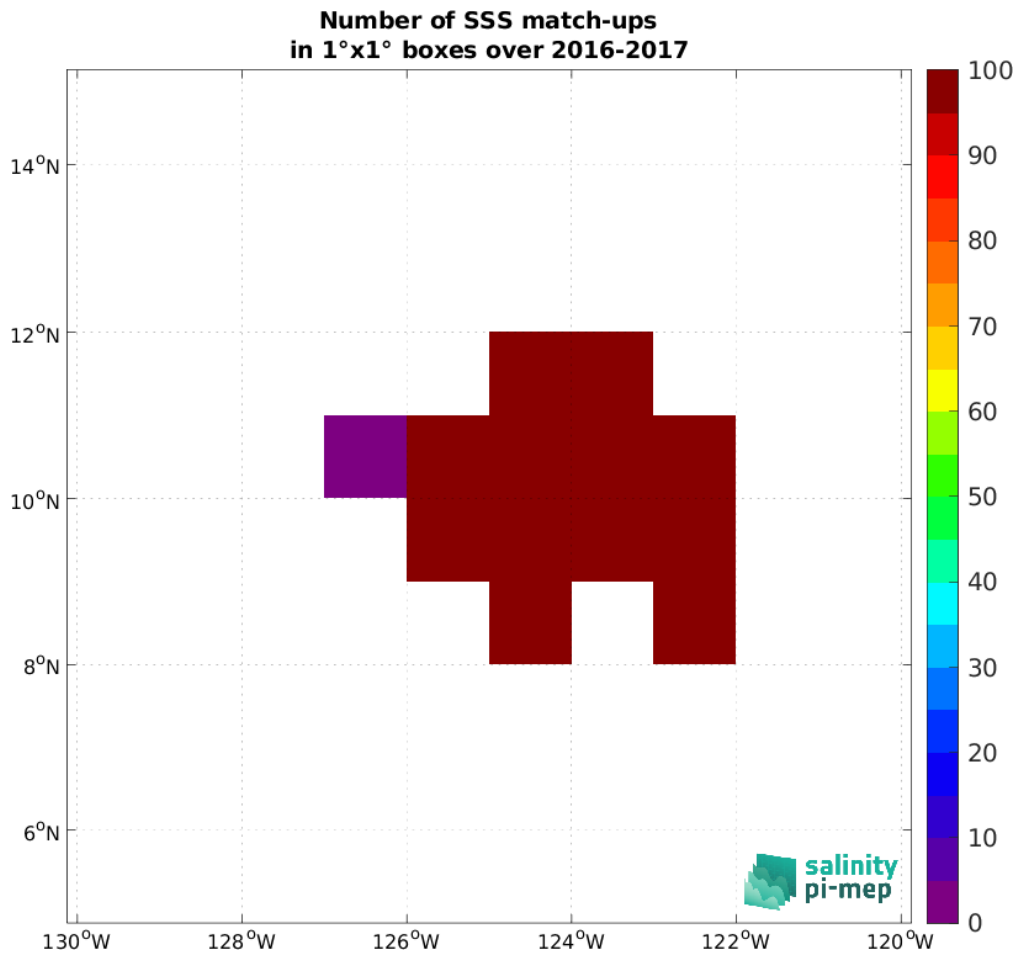
Figure 4: Number of SSS match-ups between Seagliders (SPURS 2) SSS and the SMOS SSS L4 OI v342 - Weekly (CMEMS-CATDS-LOPS) SSS product for the SPURS 2 Pi-MEP region over 1^\circ \times 1^\circ boxes and for the full satellite product period.
