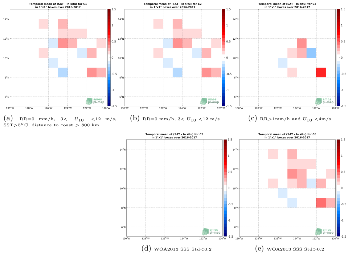
Figure 11: Temporal mean gridded over spatial boxes of size 1^\circ \times 1^\circ of \Delta SSS (SMOS L4 v2 Weekly (CATDS-CECOS-IFREMER) - Waveglider) for 5 different subdatasets corresponding to:RR=0 mm/h, 3 < U_{10} < 12 m/s, SST >5^\circ\text{C} , distance to coast > 800 km (a), RR=0 mm/h, 3 < U_{10} < 12 m/s (b), RR >1 mm/h and U_{10} < 4 m/s (c), WOA2013 SSS Std <0.2 (d), WOA2013 SSS Std >0.2 (e).
