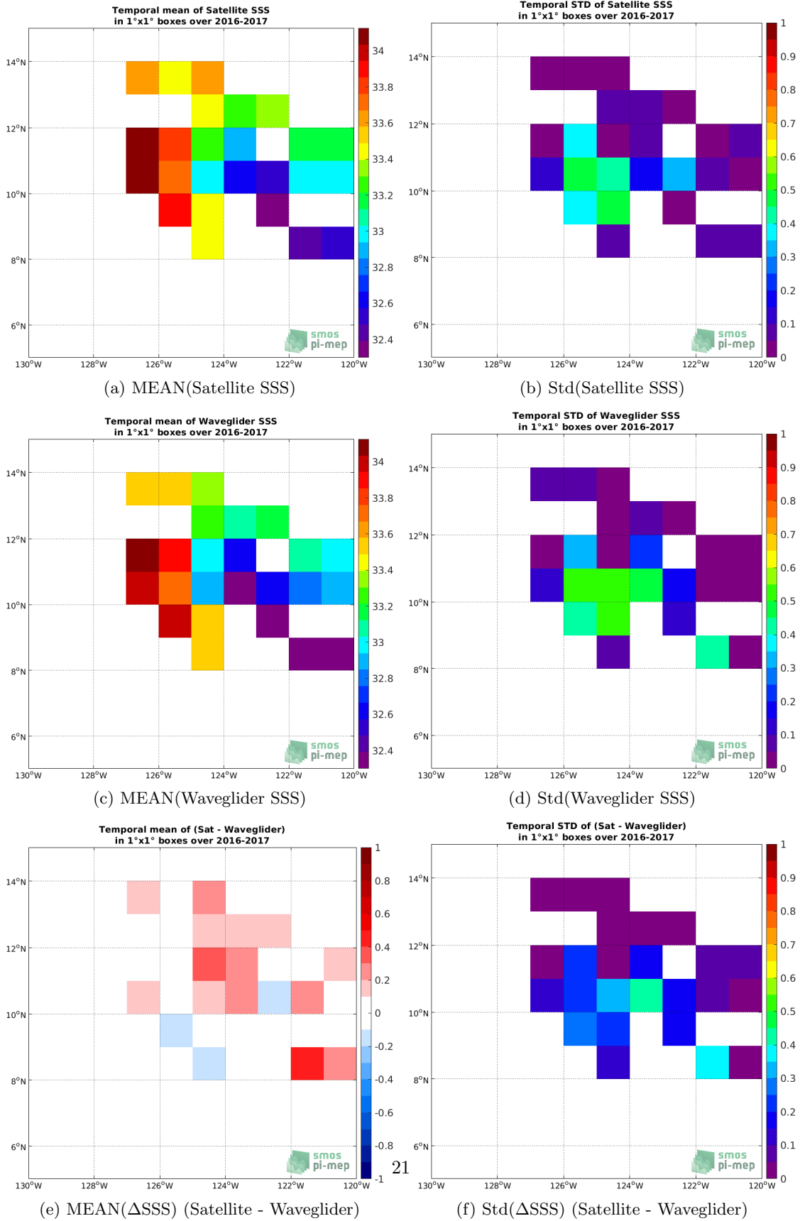
Figure 5: Temporal mean (left) and Std (right) of SSS from SMOS L4 v2 Weekly (CATDS-CECOS-IFREMER) (top), Waveglider (middle), and of \Delta SSS (Satellite - Waveglider). Only match-up pairs are used to generate these maps.
