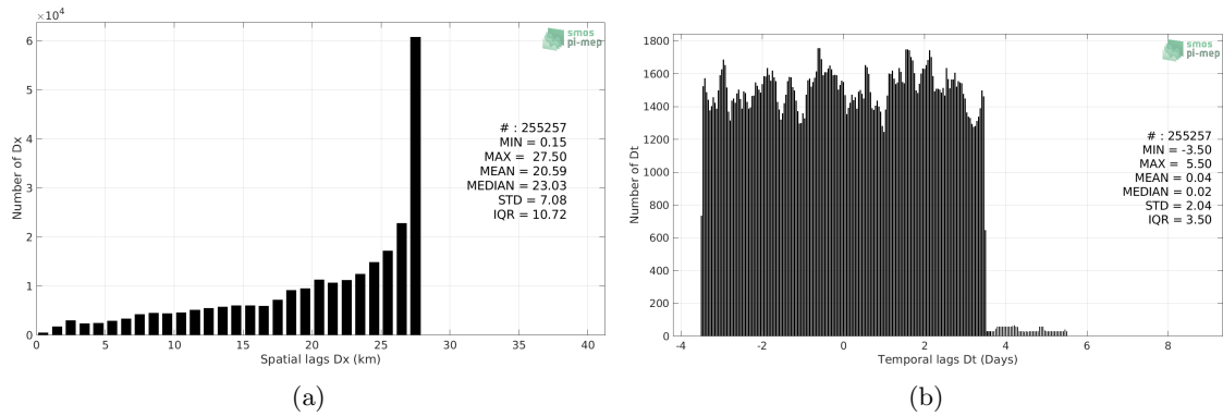
Figure 4: Histograms of the spatial (a) and temporal (b) lags between the location/time of the Waveglider measurement and the date of the corresponding SMOS L4 v2 Weekly (CATDS-CECOS-IFREMER) SSS pixel.
