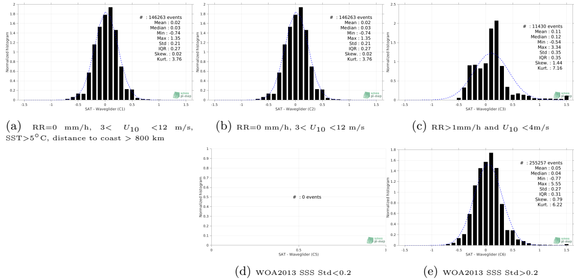
Figure 12: Normalized histogram of \Delta SSS (SMOS L4 v2 Weekly (CATDS-CECOS-IFREMER) - Waveglider) for 5 different subdatasets corresponding to: RR=0 mm/h, 3 < U_{10} < 12 m/s, SST > 5°C, distance to coast > 800 km (a), RR=0 mm/h, 3 < U_{10} < 12 m/s (b), RR > 1mm/h and U_{10} < 4 m/s (c), WOA2013 SSS Std < 0.2 (d), WOA2013 SSS Std > 0.2 (e).
