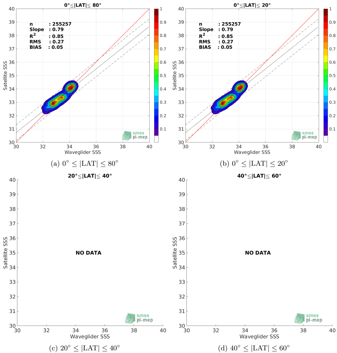
Figure 8: Contour maps of the concentration of SMOS L4 v2 Weekly (CATDS-CECOS-IFREMER) SSS (y-axis) versus Waveglider SSS (x-axis) at match-up pairs for different latitude bands. For each plot, the red line shows x=y . The black thin and dashed lines indicate a linear fit through the data cloud and the \pm 95\% confidence levels, respectively. The number match-up pairs n , the slope and R^2 coefficient of the linear fit, the root mean square (RMS) and the mean bias between satellite and in situ data are indicated for each latitude band in each plots.
