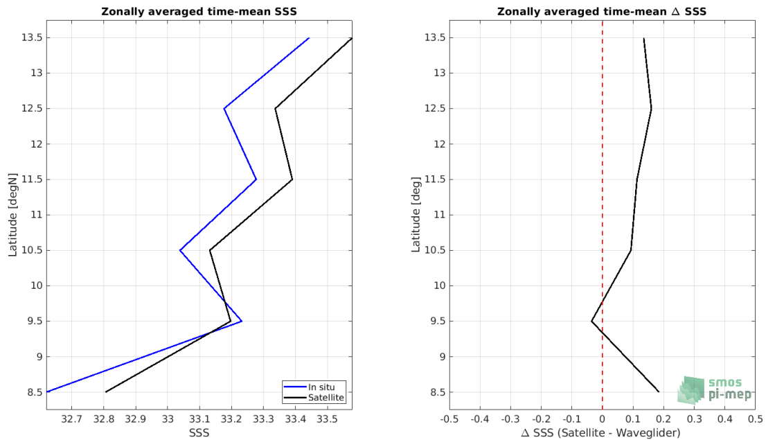
Figure 7: Left panel: Zonal mean SSS from SMOS L4 v2 Weekly (CATDS-CECOS-IFREMER) satellite product (black) and from Waveglider (blue). Right panel: Zonal mean of \Delta SSS (Satellite - Waveglider) for all the collected Pi-MEP match-up pairs estimated over the full satellite product period.
