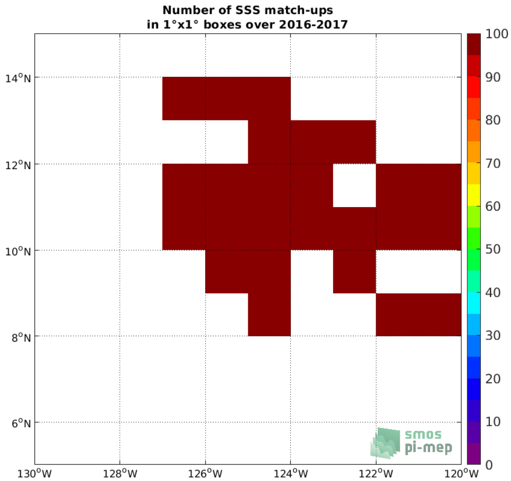
Figure 3: Number of SSS match-ups between Waveglider SSS and the SMOS L4 v2 Weekly (CATDS-CECOS-IFREMER) SSS product for the SPURS 2 Pi-MEP region over 1°x1° boxes and for the full satellite product period.
