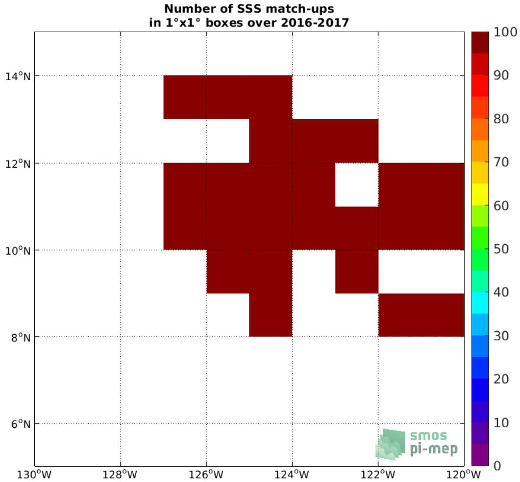
Figure 4: Number of SSS match-ups between Waveglider SSS and the SMOS L4 v2 Weekly (CATDS-CECOS-IFREMER) SSS product for the SPURS 2 Pi-MEP region over 1°x1° boxes and for the full satellite product period.
