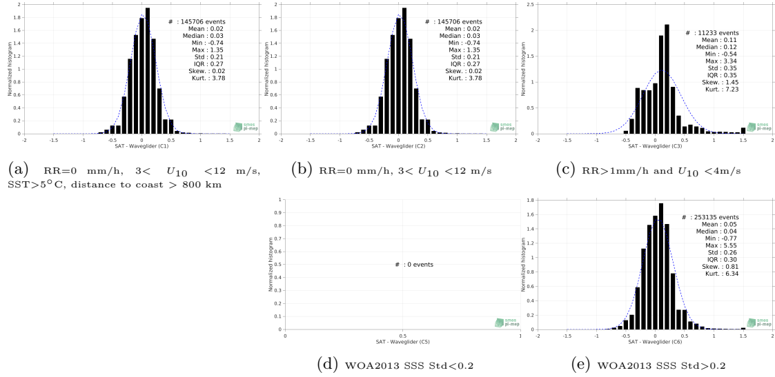
Figure 13: Normalized histogram of \Delta SSS (SMOS L4 v2 Weekly (CATDS-CECOS-IFREMER) - Waveglider) for 5 different subdatasets corresponding to: RR=0 mm/h, 3 < U_{10} < 12 m/s, SST > 5°C, distance to coast > 800 km (a), RR=0 mm/h, 3 < U_{10} < 12 m/s (b), RR > 1mm/h and U_{10} < 4 m/s (c), WOA2013 SSS Std < 0.2 (d), WOA2013 SSS Std > 0.2 (e).
