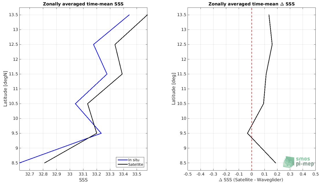
Figure 8: Left panel: Zonal mean SSS from SMOS L4 v2 Weekly (CATDS-CECOS-IFREMER) satellite product (black) and from Waveglider (blue). Right panel: Zonal mean of \Delta SSS (Satellite - Waveglider) for all the collected Pi-MEP match-up pairs estimated over the full satellite product period.
