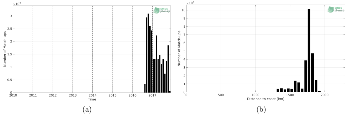
Figure 1: Number of match-ups between Waveglider and SMOS L4 v2 Weekly (CATDS-CECOS-IFREMER) SSS as a function of time (a) and as function of the distance to coast (b) over the SPURS 2 Pi-MEP region and for the full satellite product period.
