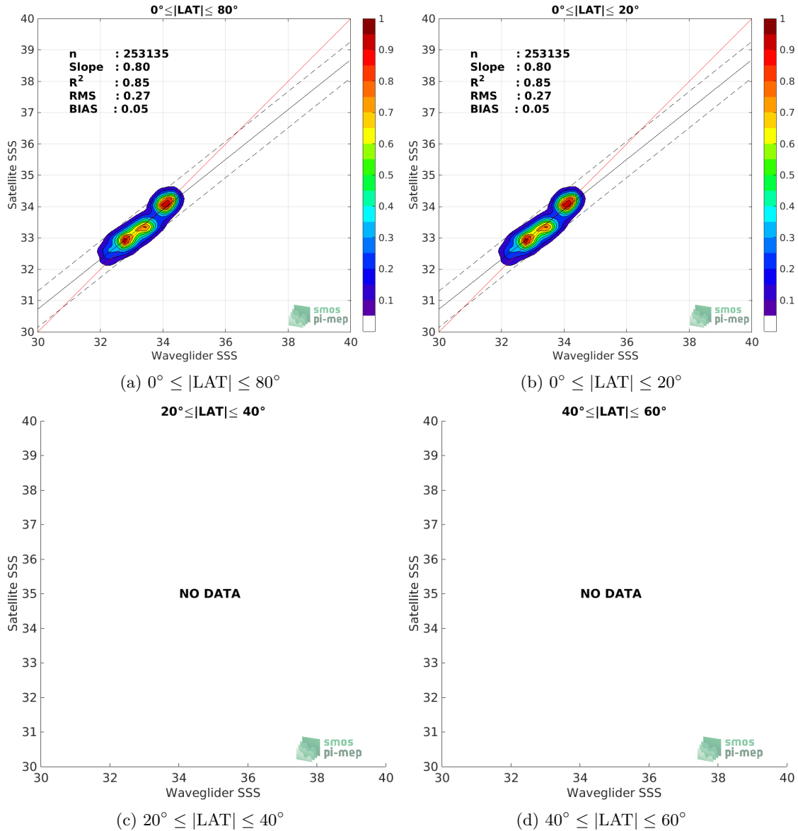
Figure 9: Contour maps of the concentration of SMOS L4 v2 Weekly (CATDS-CECOS-IFREMER) SSS (y-axis) versus Waveglider SSS (x-axis) at match-up pairs for different latitude bands. For each plot, the red line shows x=y . The black thin and dashed lines indicate a linear fit through the data cloud and the \pm 95\% confidence levels, respectively. The number match-up pairs n , the slope and R^2 coefficient of the linear fit, the root mean square (RMS) and the mean bias between satellite and in situ data are indicated for each latitude band in each plots.
