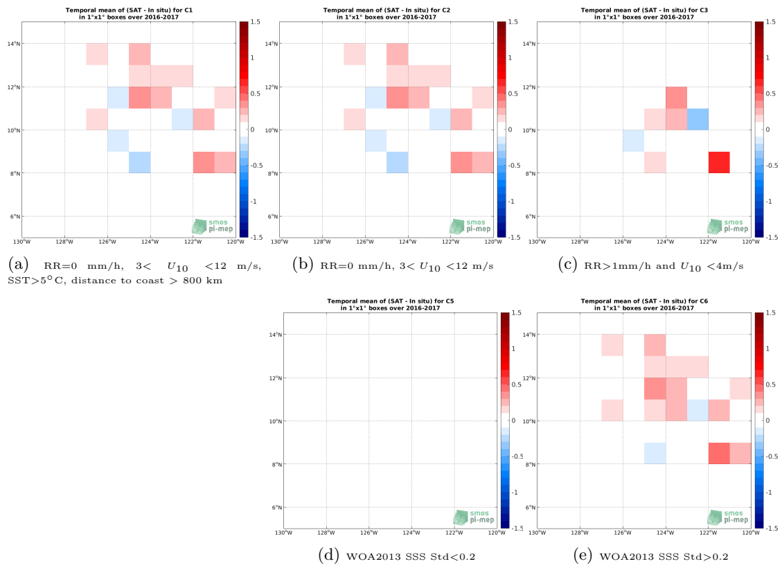
Figure 12: Temporal mean gridded over spatial boxes of size 1^\circ \times 1^\circ of \Delta SSS (SMOS L4 v2 Weekly (CATDS-CECOS-IFREMER) - Waveglider) for 5 different subdatasets corresponding to: RR=0 mm/h, 3 < U_{10} < 12 m/s, SST > 5^\circ\text{C} , distance to coast > 800 km (a), RR=0 mm/h, 3 < U_{10} < 12 m/s (b), RR > 1 mm/h and U_{10} < 4 m/s (c), WOA2013 SSS Std < 0.2 (d), WOA2013 SSS Std > 0.2 (e).
