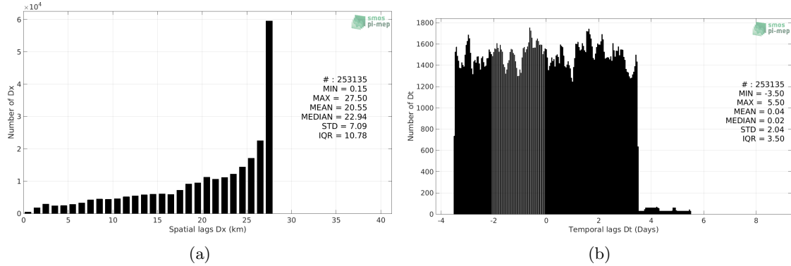
Figure 5: Histograms of the spatial (a) and temporal (b) lags between the time of the Waveglider measurements and the date of the corresponding SMOS L4 v2 Weekly (CATDS-CECOS-IFREMER) SSS product.
