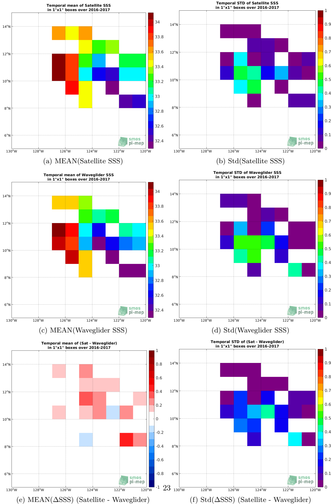
Figure 6: Temporal mean (left) and Std (right) of SSS from SMOS L4 v2 Weekly (CATDS-CECOS-IFREMER) (top), Waveglider (middle), and of \Delta SSS (Satellite - Waveglider). Only match-up pairs are used to generate these maps.
