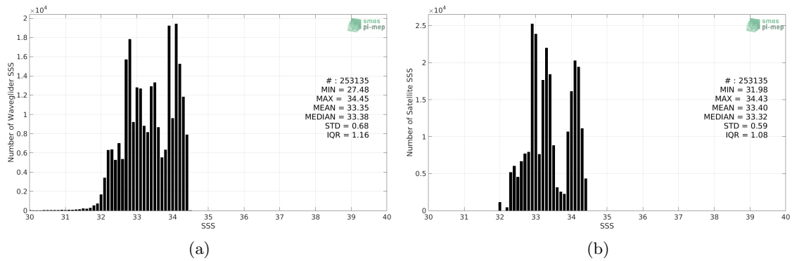
Figure 2: Histograms of SSS from Waveglider (a) and SMOS L4 v2 Weekly (CATDS-CECOS-IFREMER) (b) considering all match-up pairs per bins of 0.1 over the SPURS 2 Pi-MEP region and for the full satellite product period.
