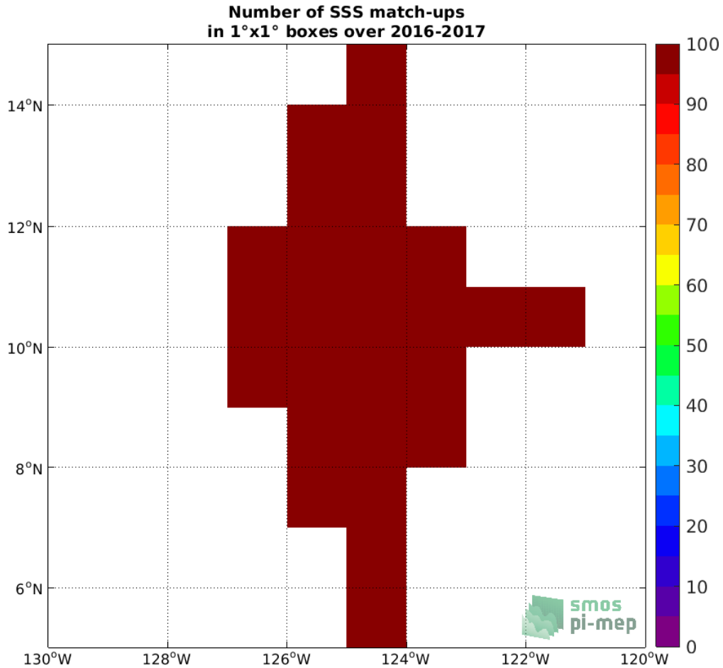
Figure 4: Number of SSS match-ups between Salinity Snake SSS and the SMOS L4 v2 Weekly (CATDS-CECOS-IFREMER) SSS product for the SPURS 2 Pi-MEP region over 1°x1° boxes and for the full satellite product period.
