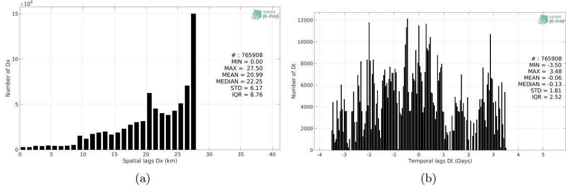
Figure 5: Histograms of the spatial (a) and temporal (b) lags between the time of the Salinity Snake measurements and the date of the corresponding SMOS L4 v2 Weekly (CATDS-CECOS-IFREMER) SSS product.
