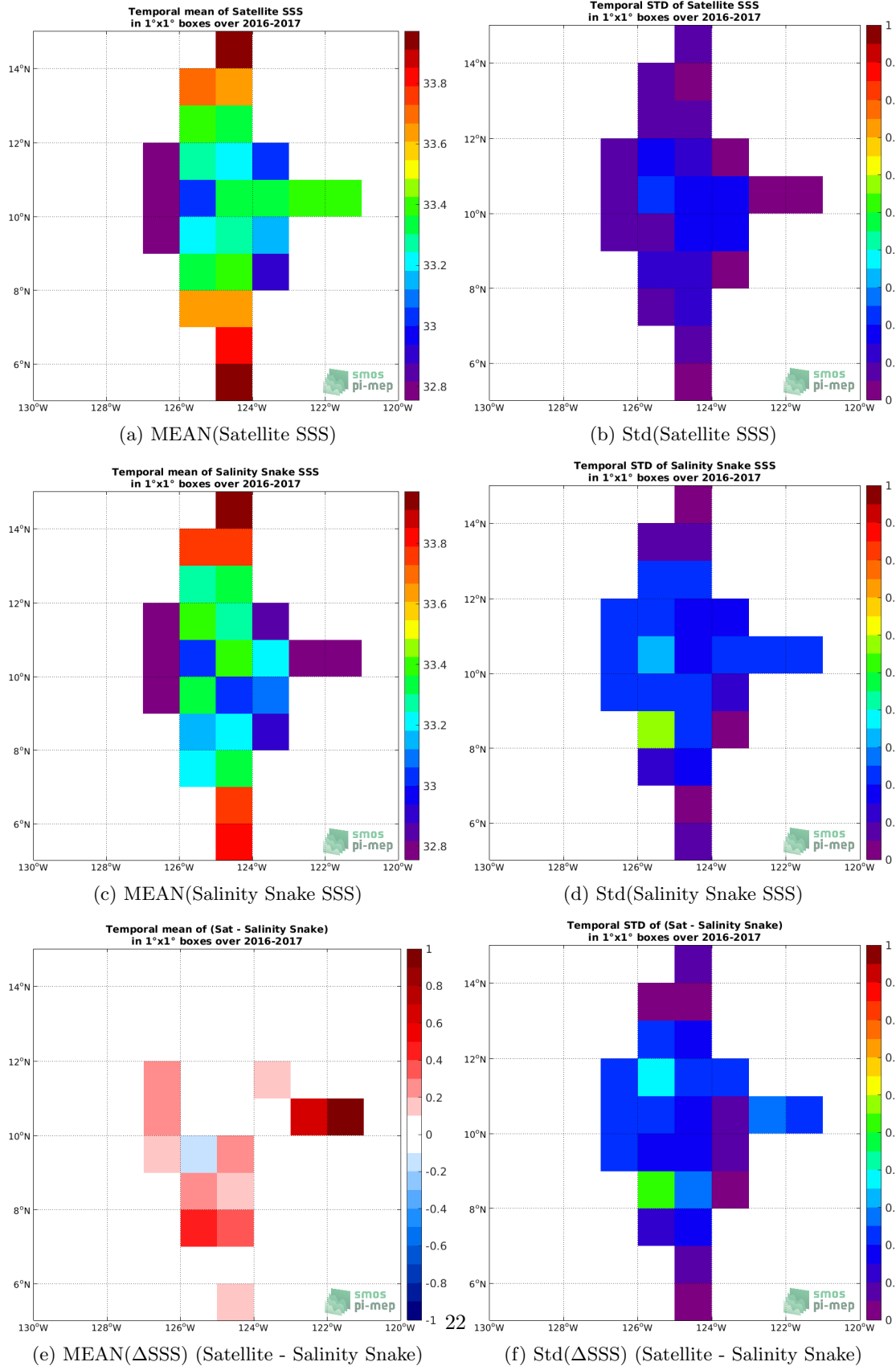
Figure 6: Temporal mean (left) and Std (right) of SSS from SMOS L4 v2 Weekly (CATDS-CECOS-IFREMER) (top), Salinity Snake (middle), and of \Delta SSS (Satellite - Salinity Snake). Only match-up pairs are used to generate these maps.
