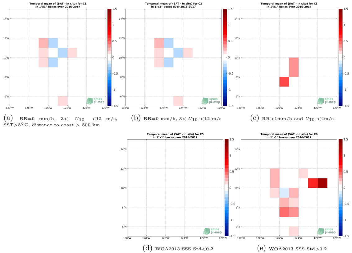
Figure 12: Temporal mean gridded over spatial boxes of size 1^{\circ}\times 1^{\circ} of \Delta\text{SSS} (SMOS L4 v2 Weekly (CATDS-CECOS-IFREMER) - Salinity Snake) for 5 different subdatasets corresponding to:RR=0 mm/h, 3 < U_{10} < 12 m/s, SST >5^{\circ}\text{C} , distance to coast > 800 km (a), RR=0 mm/h, 3 < U_{10} < 12 m/s (b), RR >1 mm/h and U_{10} < 4 m/s (c), WOA2013 SSS Std <0.2 (d), WOA2013 SSS Std >0.2 (e).
