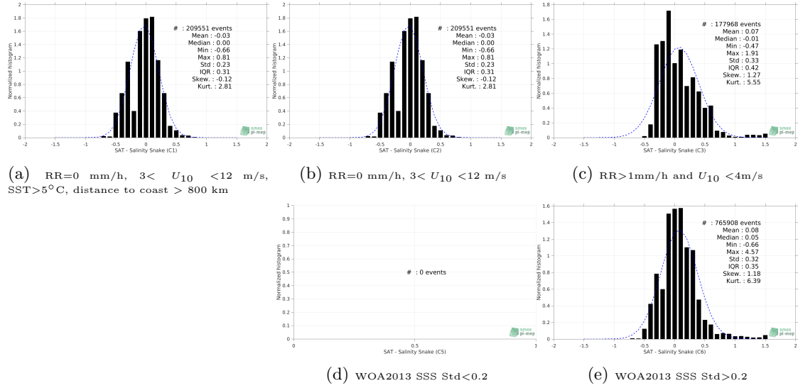
Figure 13: Normalized histogram of \Delta SSS (SMOS L4 v2 Weekly (CATDS-CECOS-IFREMER) - Salinity Snake) for 5 different subdatasets corresponding to: RR=0 mm/h, 3 < U_{10} < 12 m/s, SST>5°C, distance to coast > 800 km (a), RR=0 mm/h, 3 < U_{10} < 12 m/s (b), RR>1mm/h and U_{10} < 4 m/s (c), WOA2013 SSS Std<0.2 (d), WOA2013 SSS Std>0.2 (e).
