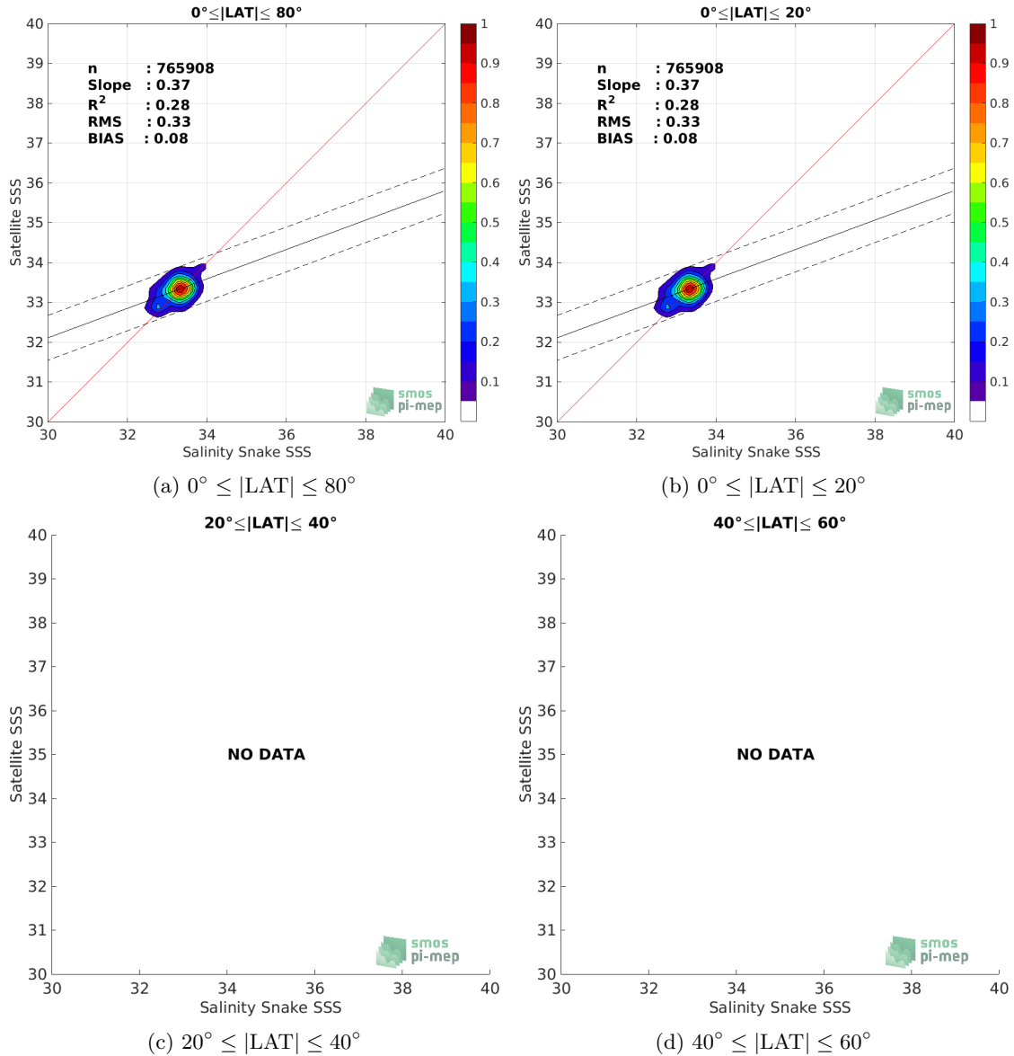
Figure 9: Contour maps of the concentration of SMOS L4 v2 Weekly (CATDS-CECOS-IFREMER) SSS (y-axis) versus Salinity Snake SSS (x-axis) at match-up pairs for different latitude bands. For each plot, the red line shows x=y . The black thin and dashed lines indicate a linear fit through the data cloud and the \pm 95\% confidence levels, respectively. The number match-up pairs n , the slope and R^2 coefficient of the linear fit, the root mean square (RMS) and the mean bias between satellite and in situ data are indicated for each latitude band in each plots.
