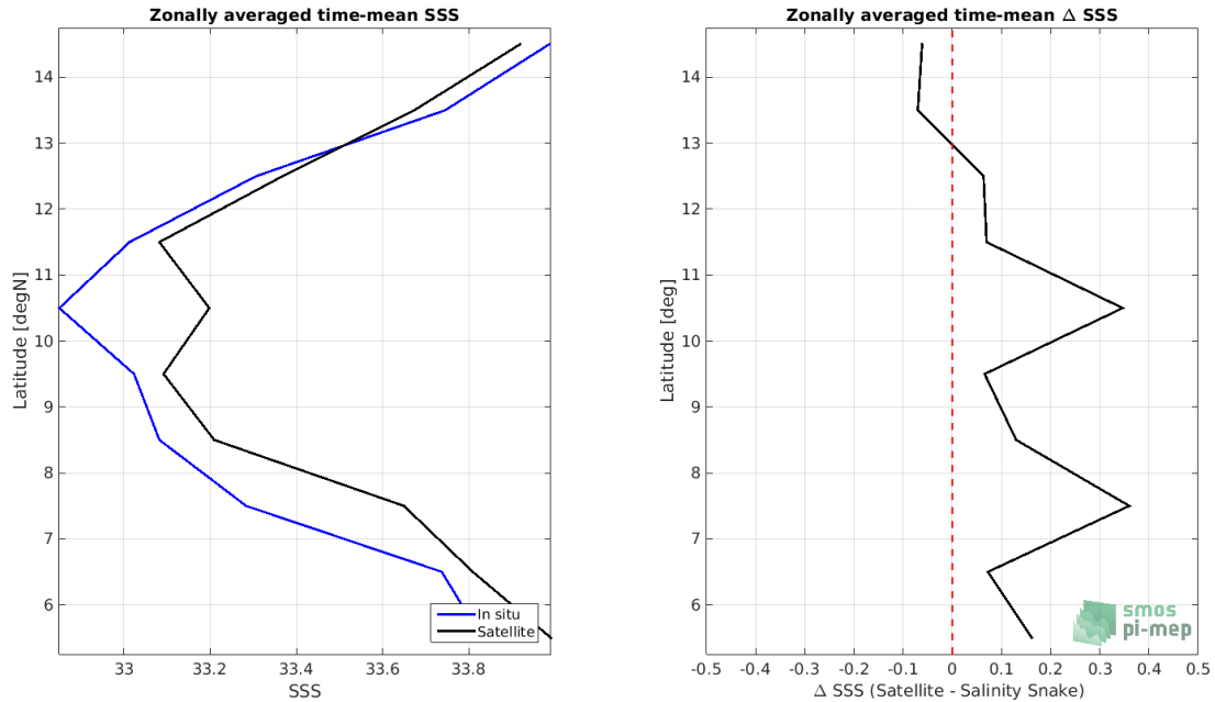
Figure 8: Left panel: Zonal mean SSS from SMOS L4 v2 Weekly (CATDS-CECOS-IFREMER) satellite product (black) and from Salinity Snake (blue). Right panel: Zonal mean of \Delta SSS (Satellite - Salinity Snake) for all the collected Pi-MEP match-up pairs estimated over the full satellite product period.
