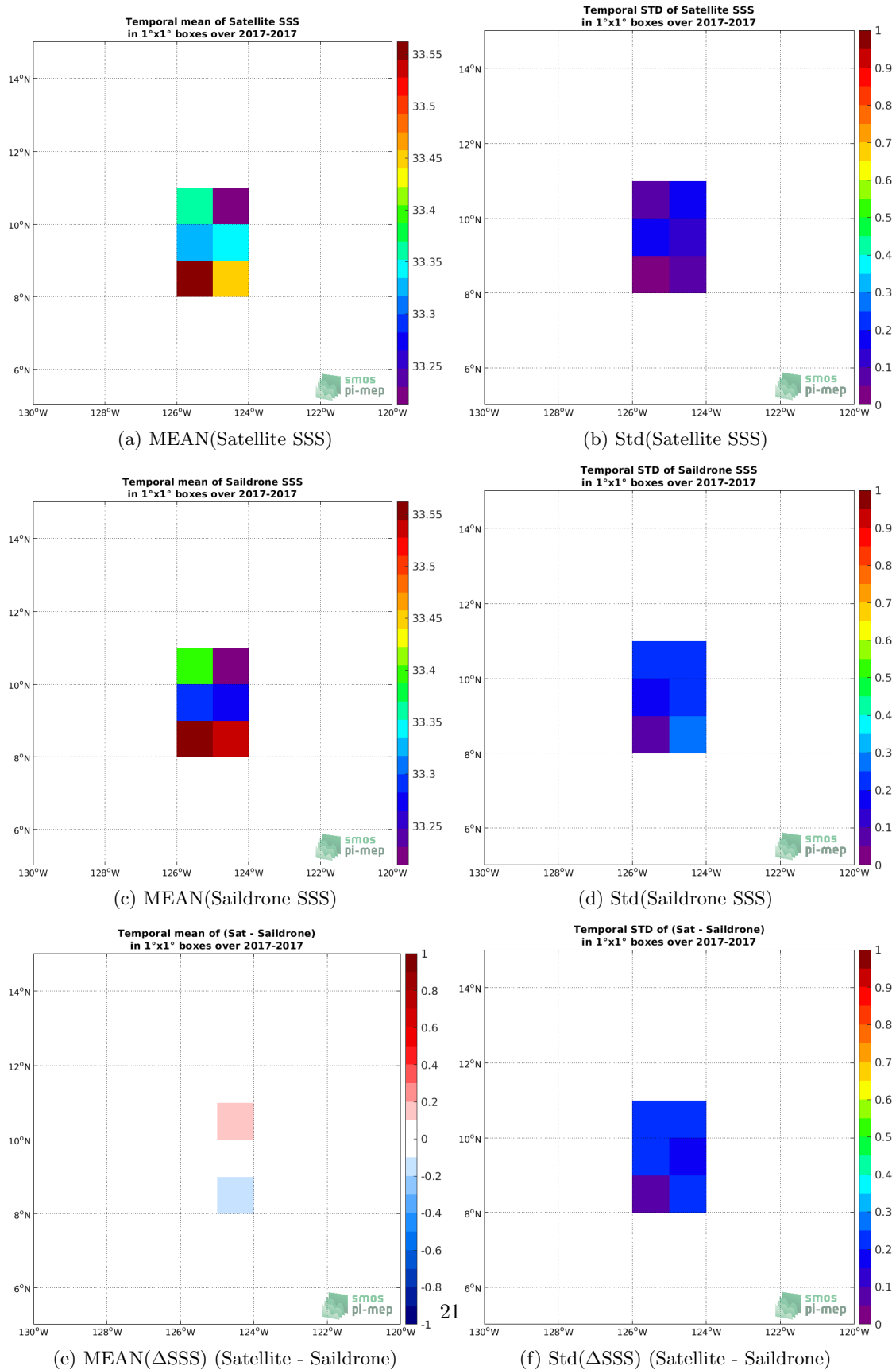
Figure 5: Temporal mean (left) and Std (right) of SSS from SMOS L4 v2 Weekly (CATDS-CECOS-IFREMER) (top), Saildrone (middle), and of \Delta SSS (Satellite - Saildrone). Only match-up pairs are used to generate these maps.
