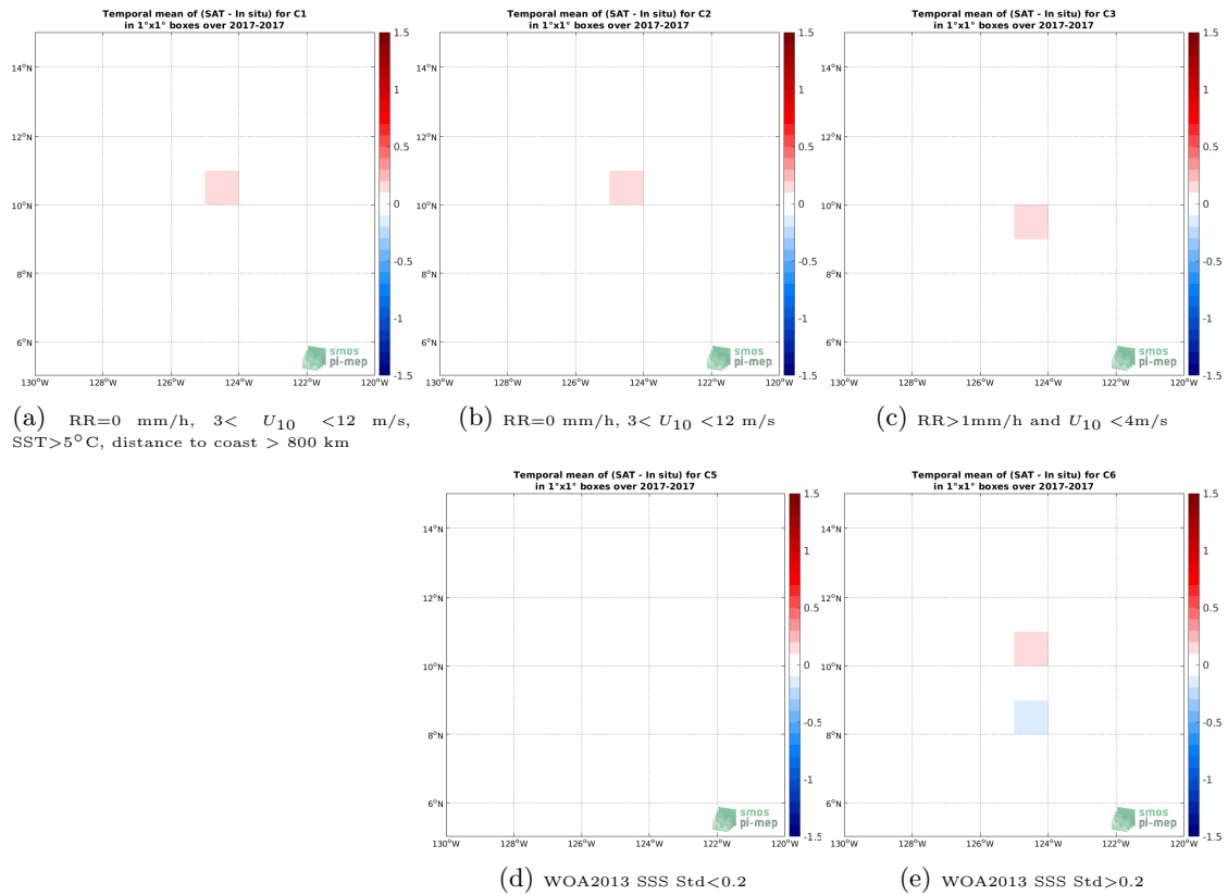
Figure 11: Temporal mean gridded over spatial boxes of size 1^\circ \times 1^\circ of \Delta SSS (SMOS L4 v2 Weekly (CATDS-CECOS-IFREMER) - Saildrone) for 5 different subdatasets corresponding to:RR=0 mm/h, 3 < U_{10} < 12 m/s, SST >5^\circ\text{C} , distance to coast > 800 km (a), RR=0 mm/h, 3 < U_{10} < 12 m/s (b), RR >1 mm/h and U_{10} < 4 m/s (c), WOA2013 SSS Std <0.2 (d), WOA2013 SSS Std >0.2 (e).
