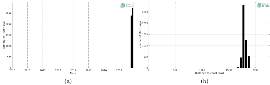
Figure 1: Number of match-ups between Saildrone and SMOS L4 v2 Weekly (CATDS-CECOS-IFREMER) SSS as a function of time (a) and as function of the distance to coast (b) over the SPURS 2 Pi-MEP region and for the full satellite product period.
