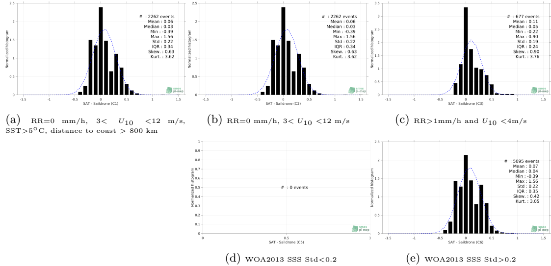
Figure 12: Normalized histogram of \Delta SSS (SMOS L4 v2 Weekly (CATDS-CECOS-IFREMER) - Saildrone) for 5 different subdatasets corresponding to: RR=0 mm/h, 3 < U_{10} < 12 m/s, SST > 5°C, distance to coast > 800 km (a), RR=0 mm/h, 3 < U_{10} < 12 m/s (b), RR > 1mm/h and U_{10} < 4 m/s (c), WOA2013 SSS Std < 0.2 (d), WOA2013 SSS Std > 0.2 (e).
