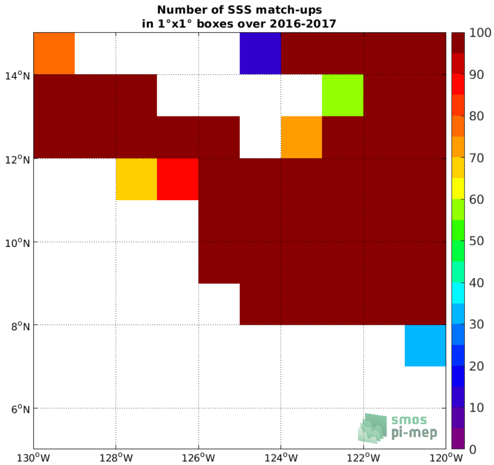
Figure 3: Number of SSS match-ups between Surface drifters SSS and the SMOS L4 v2 Weekly (CATDS-CECOS-IFREMER) SSS product for the SPURS 2 Pi-MEP region over 1°x1° boxes and for the full satellite product period.
